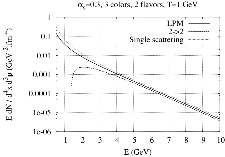
Fig. 47: \mathcal{O}(\alpha_s) contributions to the photon production rate in a QGP. The parameters used in this plot are \alpha_s = 0.3 , 3 colors, 2 flavors and T = 1 \text{ GeV} .
