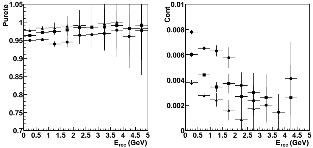
Fig. 14: Photon purity and antineutron contamination to the identified photon spectrum in HIJING Pb-Pb collisions, for three definitions of photon quality: low ( \blacktriangle ), medium ( \blacksquare ) and high ( \bullet ) purity photons.
