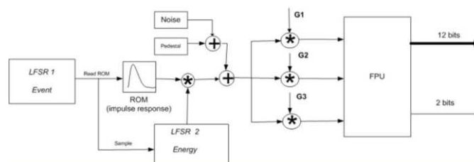
Figure 4: Modelling of signals from VFE
