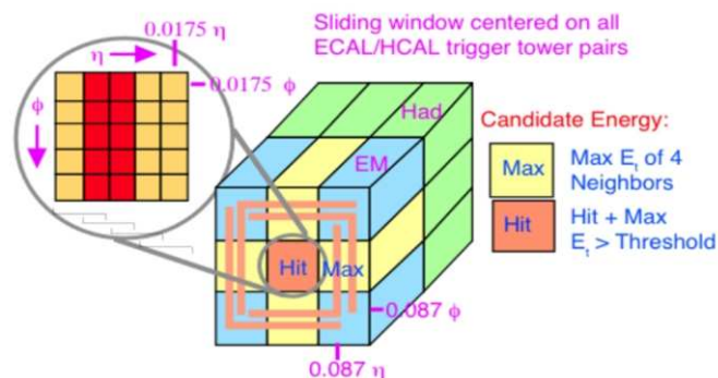
Figure 1: Principle of the Level-1 electron/photon trigger algorithm.
