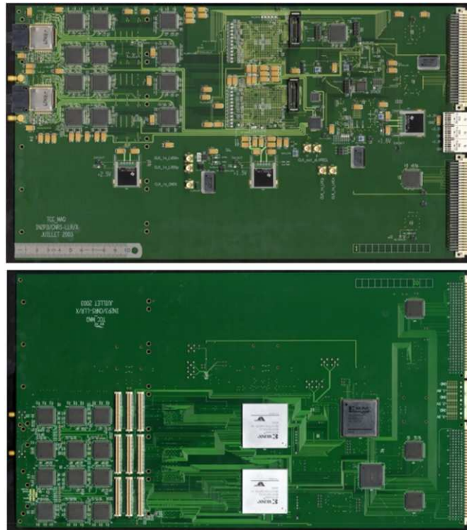
Figure 6: The 2 sides of the Trigger Concentrator Card prototype
