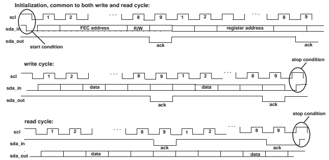
Figure 4: Front-end Control Bus protocol. The standard I 2 C ® SDA line is split in 2 unidirectional lines: SDA_in from the RCU to the FECs and SDA_out in the opposite direction.
