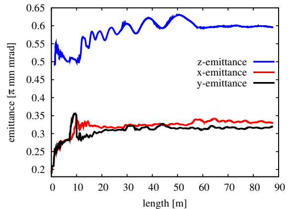
Figure 3: End-to-end (LEBT to 160 MeV) rms emittance evolution (from PATH).
