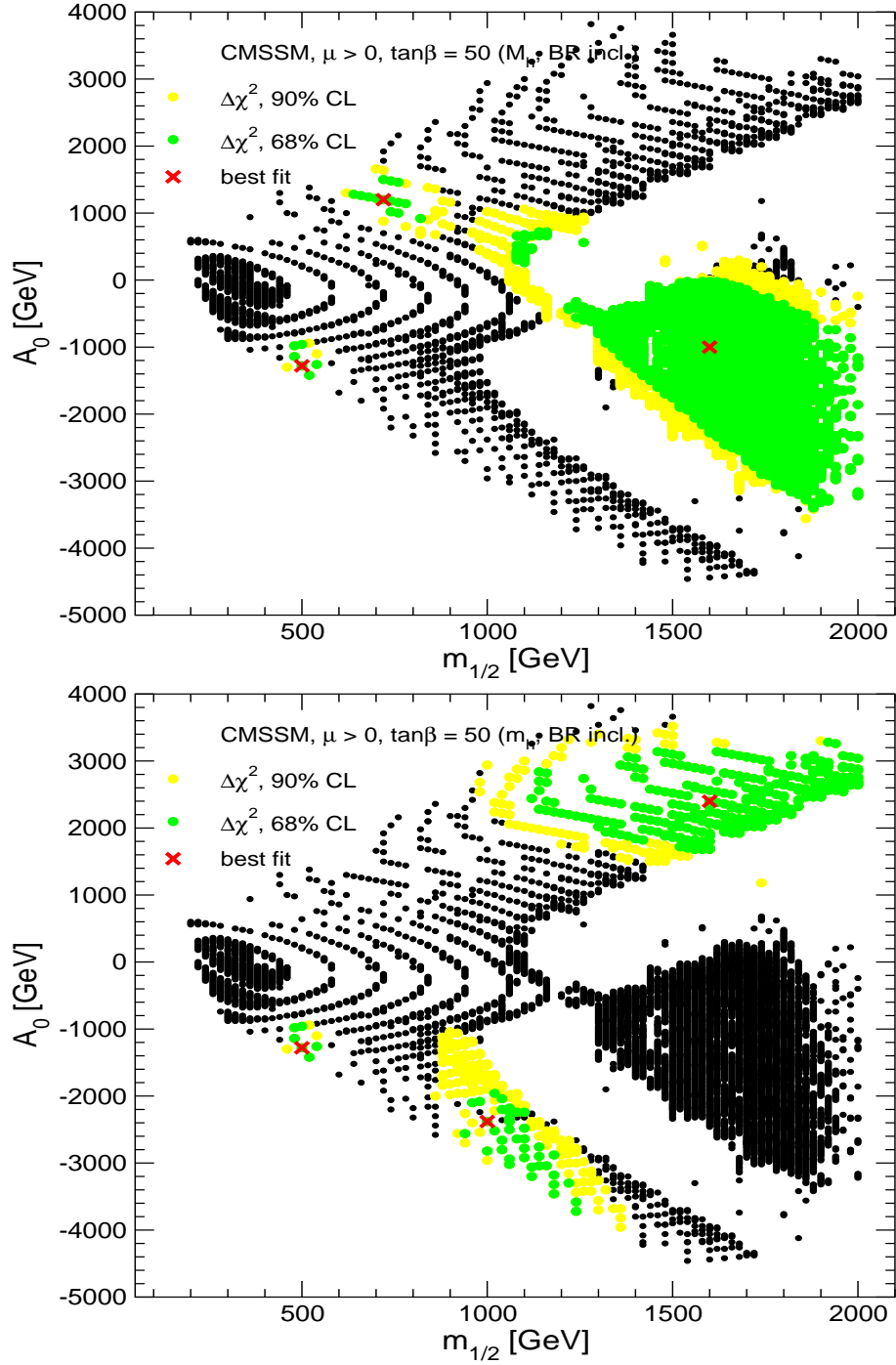
Figure 19: The results of a \chi^2 fit based on the prospective experimental accuracies for the precision observables M_W , \sin^2 \theta_{\text{eff}} , (g-2)_\mu , \text{BR}(b \rightarrow s\gamma) , M_h and Higgs branching ratios at the ILC are shown in the (m_{1/2}, A_0) plane of the CMSSM with WMAP constraints for \tan \beta = 50 . In both plots the WMAP-allowed region and the best-fit point for \tan \beta = 50 according to the current situation (see Fig. 15) are indicated. In both plots two further hypothetical future ‘best-fit’ values have been chosen for illustration. The coloured regions correspond to the 68% and 90% C.L. regions according to the ILC accuracies.
