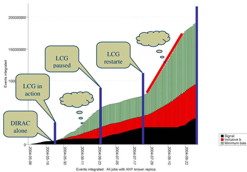
Figure 1: Number of events integrated during the production phase.
