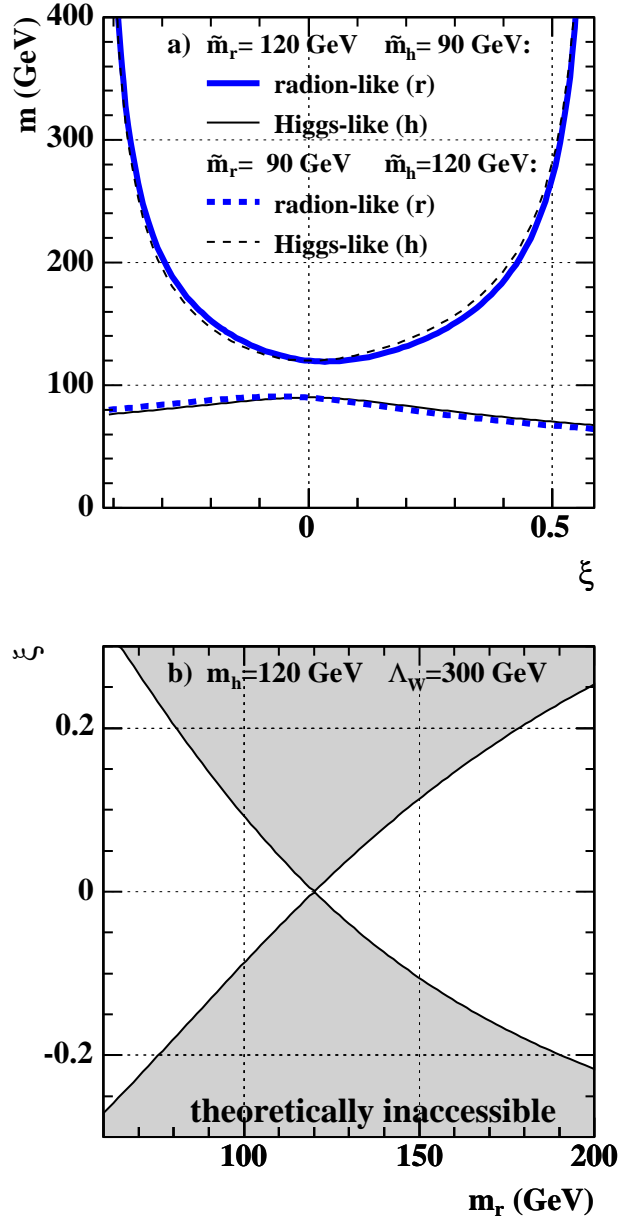
Figure 1: a) Masses m_{r/h} of the heavy and light mass eigenstates for fundamental Higgs boson and radion mass parameters, \tilde{m}_h and \tilde{m}_r , of 90 GeV and 120 GeV. The fundamental radion is chosen to be heavier (lighter) than the Higgs boson, indicated by the solid (dashed) lines. The x -axis extends over the allowed \xi -range. b) Allowed parameter space in the m_r and \xi plane for a Higgs boson mass m_h = 120 GeV. Outside the permitted region the Higgs and radion-like states are unphysical (ghost-like). In both figures the weak scale was chosen to be \Lambda_W = 300 GeV.
