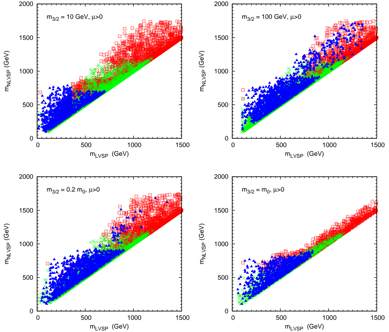
Figure 3: Scatter plots of the masses of the lightest visible supersymmetric particle (LVSP) and the next-to-lightest visible supersymmetric particle (NLVSP) in the GDM with (a) m_{3/2} = 10 \text{ GeV} , (b) m_{3/2} = 100 \text{ GeV} , (c) m_{3/2} = 0.2m_0 and (d) m_{3/2} = m_0 , all for \mu > 0 . The darker (blue) triangles satisfy all the laboratory, astrophysical and cosmological constraints. For comparison, the dark (red) squares and medium-shaded (green) crosses respect the laboratory constraints, but not those imposed by astrophysics and cosmology. In addition, the (green) crosses represent models which are expected to be visible at the LHC.
