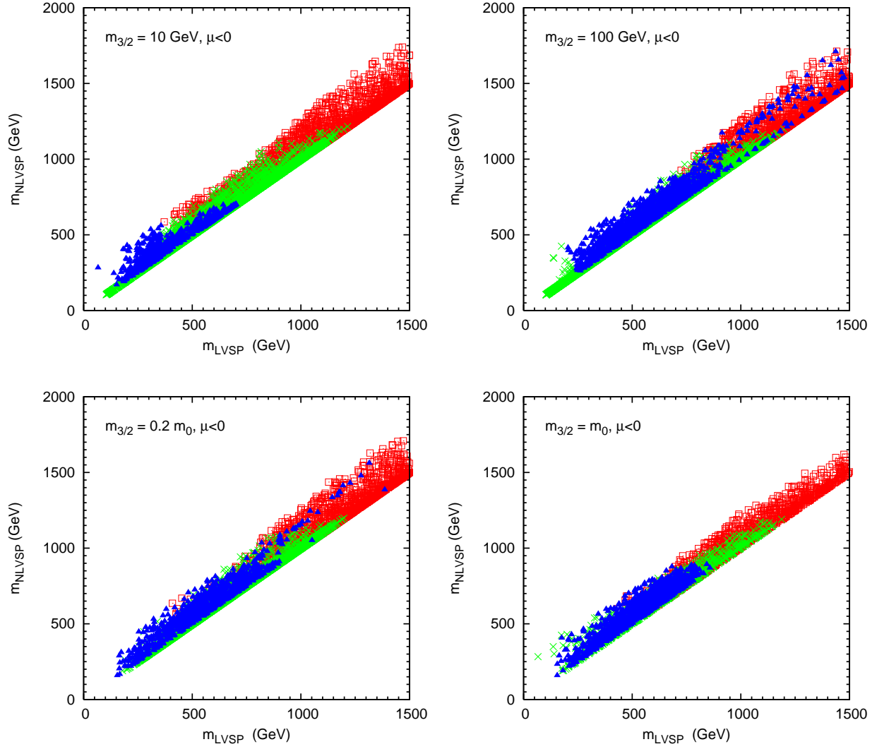
Figure 4: As in Fig. 3, but for \mu < 0 .
