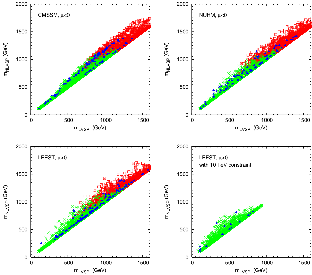
Figure 2: As in Fig. 1, but for \mu < 0 .
