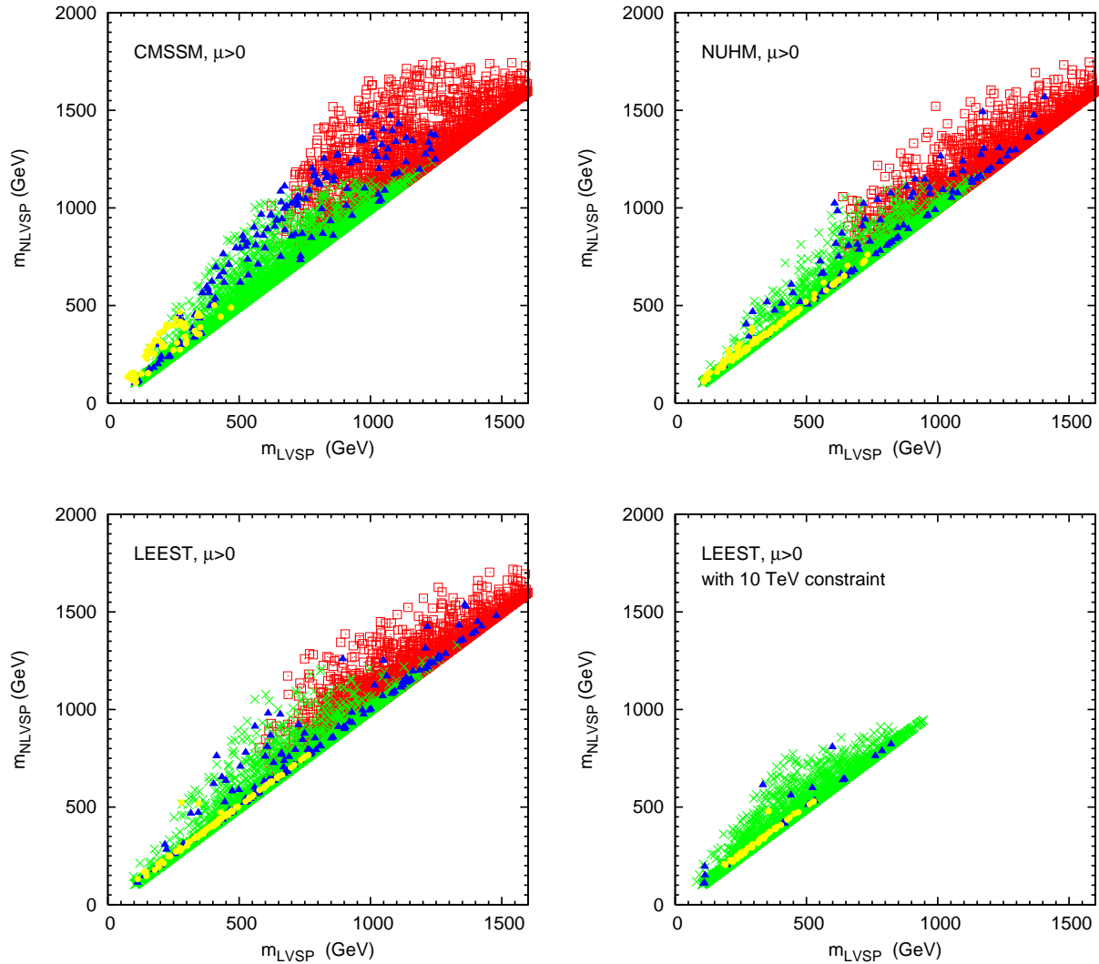
Figure 1: Scatter plots of the masses of the lightest visible supersymmetric particle (LVSP) and the next-to-lightest visible supersymmetric particle (NLVSP) in (a) the CMSSM, (b) the NUHM, (c) the LEEST and (d) the LEEST10, all for \mu > 0 . The darker (blue) triangles satisfy all the laboratory, astrophysical and cosmological constraints. For comparison, the dark (red) squares and medium-shaded (green) crosses respect the laboratory constraints, but not those imposed by astrophysics and cosmology. In addition, the (green) crosses represent models which are expected to be visible at the LHC. The very light (yellow) points are those for which direct detection of supersymmetric dark matter might be possible according to the criterion discussed in the text.
