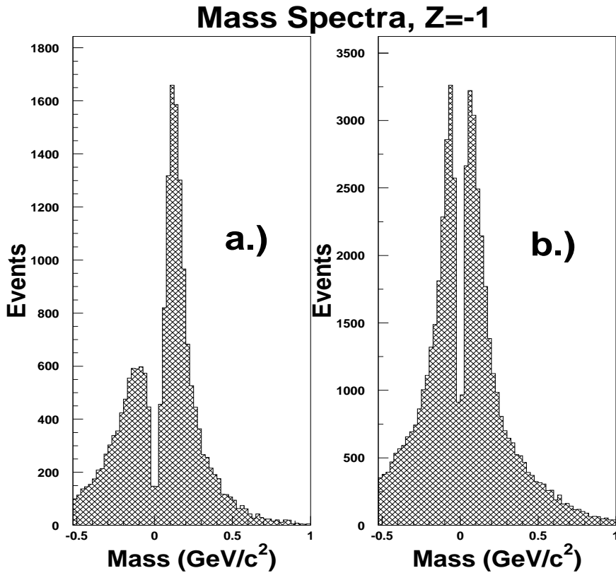
Fig. 7. Mass spectra for downward-going Z = -1 events from the excess flux region (a) and not from the excess flux region (b) in fig. 5. Note the large excess of events with masses consistent with \mu^- and \pi^- from the excess region. The meaning of negative masses are explained in the text.
