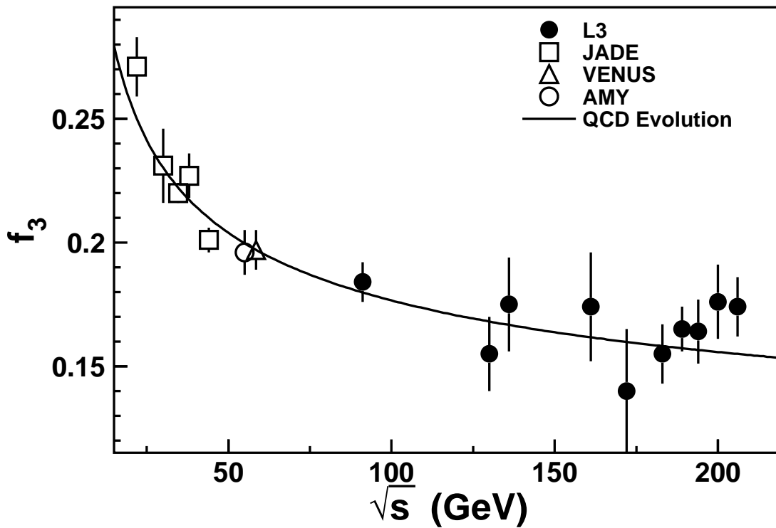
Figure 14: Energy evolution of the 3-jet fraction at y_{\text{cut}}^{\text{J}} = 0.08 with the JADE algorithm.
