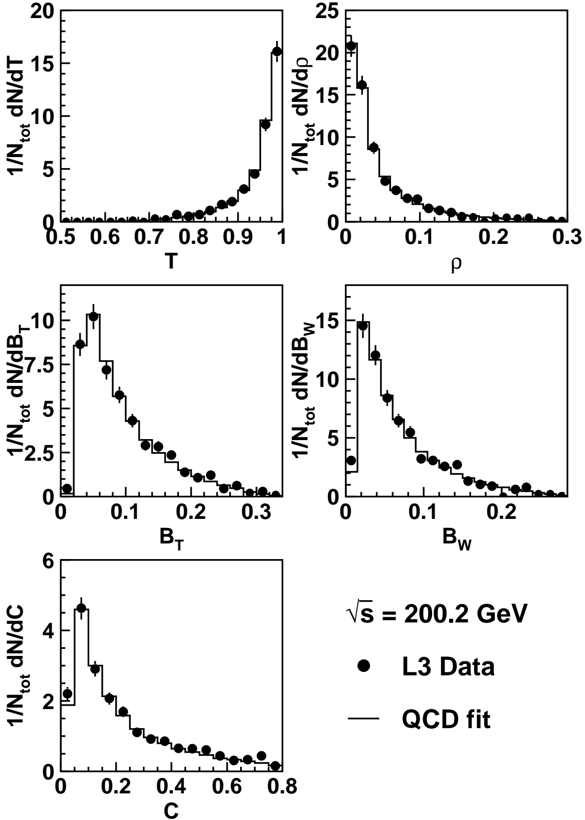
Figure 31: Measured distributions, at \langle\sqrt{s}\rangle = 200.2 \text{ GeV} , of thrust, T , scaled heavy jet mass, \rho_H , total, B_T , and wide, B_W , jet broadenings, and C -parameter compared to fitted QCD predictions. The error bars include systematic as well as statistical uncertainties.
