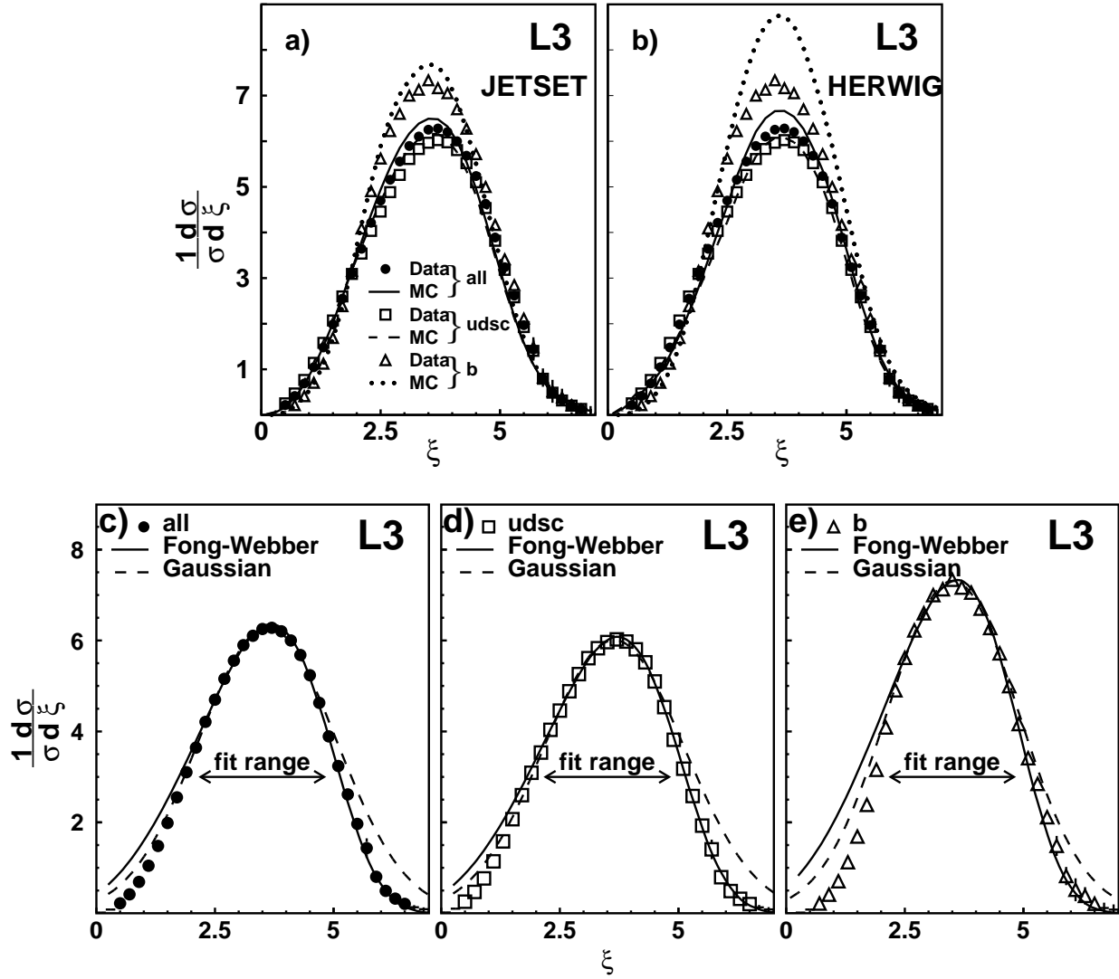
Figure 36: Corrected \xi distributions at \sqrt{s} = 91.2 GeV compared to (a) JETSET PS and (b) HERWIG and together with the results of fits to Gaussian and Fong-Webber parametrizations for the (c) all-flavour, (d) udsc- and (e) b-quark samples.
