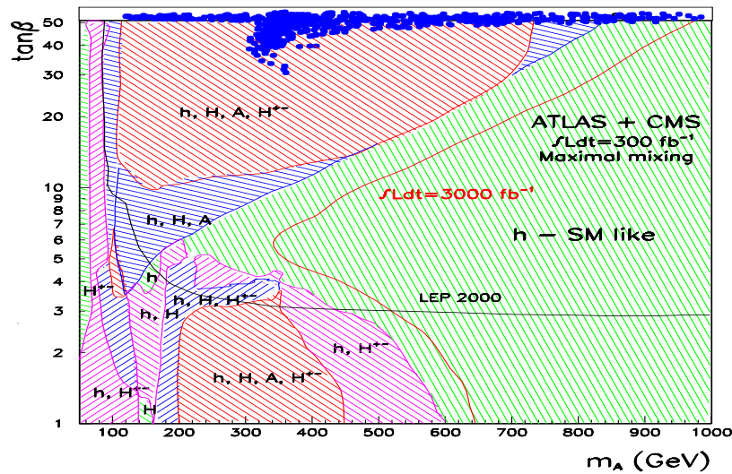
Figure 9. Estimated number of Higgs bosons observable at the LHC in the M_A , \tan\beta plane. The cosmologically interesting solutions belonging to the A funnel regions obtained with a parameter scan are shown by the dots. In the relevant region of parameters, the LHC will be essentially observing all the Higgs bosons (modified from [61]).
