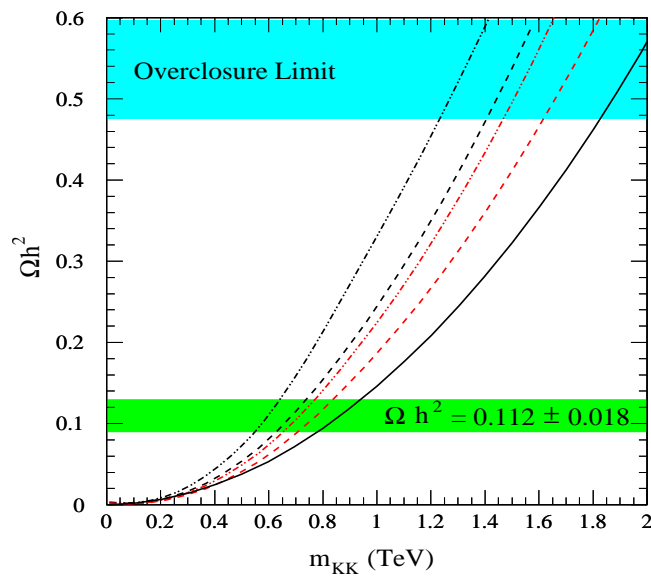
Figure 10. Relic dark matter density as a function of the UED mass scale m_{KK} = 1/R corresponding to the mass of the level one KK states. The WMAP result is shown by the horizontal band. The solid line includes only the B^{(1)} contribution. The dashed lines also include the effect of co-annihilations with one and three generations of lepton excitations for mass splittings of 1 % and 5 % (adapted from Ref. [66]).
