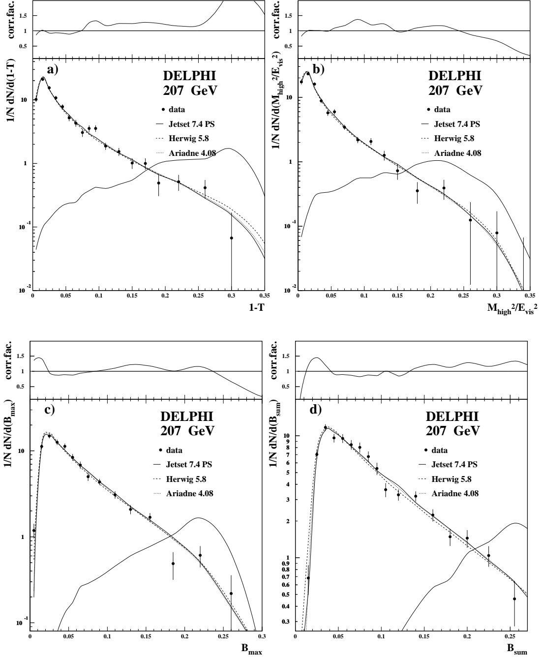
Figure 3: Event shape distributions of 1-Thrust ( 1 - T ), heavy jet mass ( M_{\text{h}}^2/E_{\text{vis}}^2 ), wide jet broadening ( B_{\text{max}} ) and total jet broadening ( B_{\text{sum}} ) at 207 GeV. The upper inset shows the acceptance corrections. The central part shows data with statistical uncertainties, simulation and the four-fermion background which was subtracted from the data.
