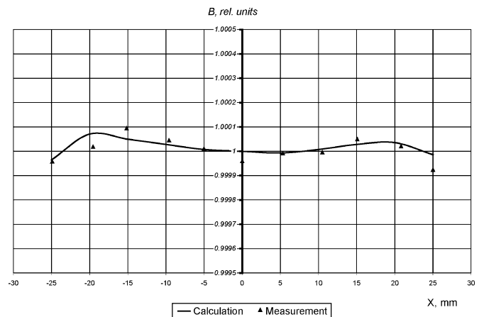
Fig. 7. Magnetic field at the center of the MBW01 magnet. Aperture 2. I = 720 A.
