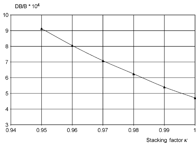
Fig. 6. Dependence of the magnetic field homogeneity within \pm 30 mm region around the equilibrium orbit from the stacking factor K at B = 1.42 T.
