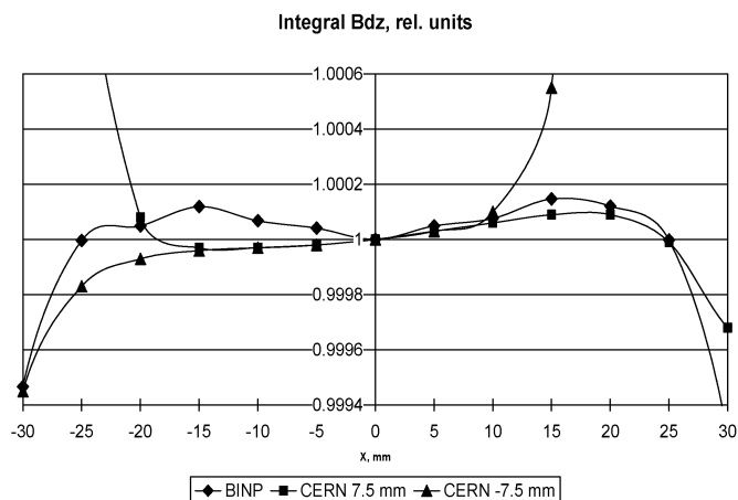
Fig. 9. Comparison between magnetic measurement with the Hall probe array and the mole and I = 720 A. BINP: measurement with an Hall probe array, CERN 7.5 mm: measurement with the mole center position at 7.5 mm. CERN -7.5 mm: measurement with the mole center position at -7.5 mm.
