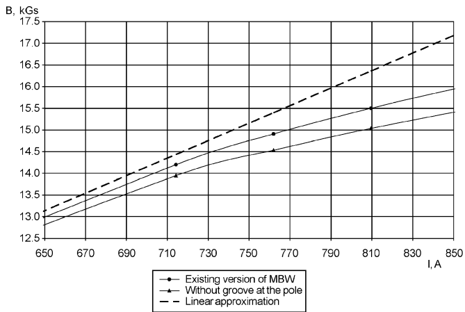
Fig. 2. Decrease of saturation by grooves at the pole.
