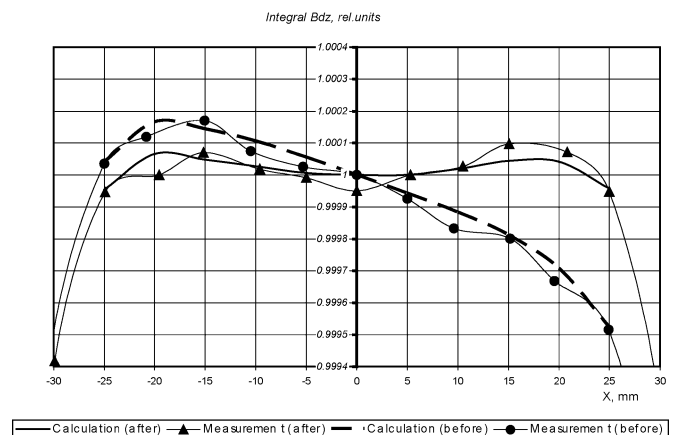
Fig. 8. Magnetic field integral of MBW01 magnet before and after correction at the end chamfers. I = 720 A.
