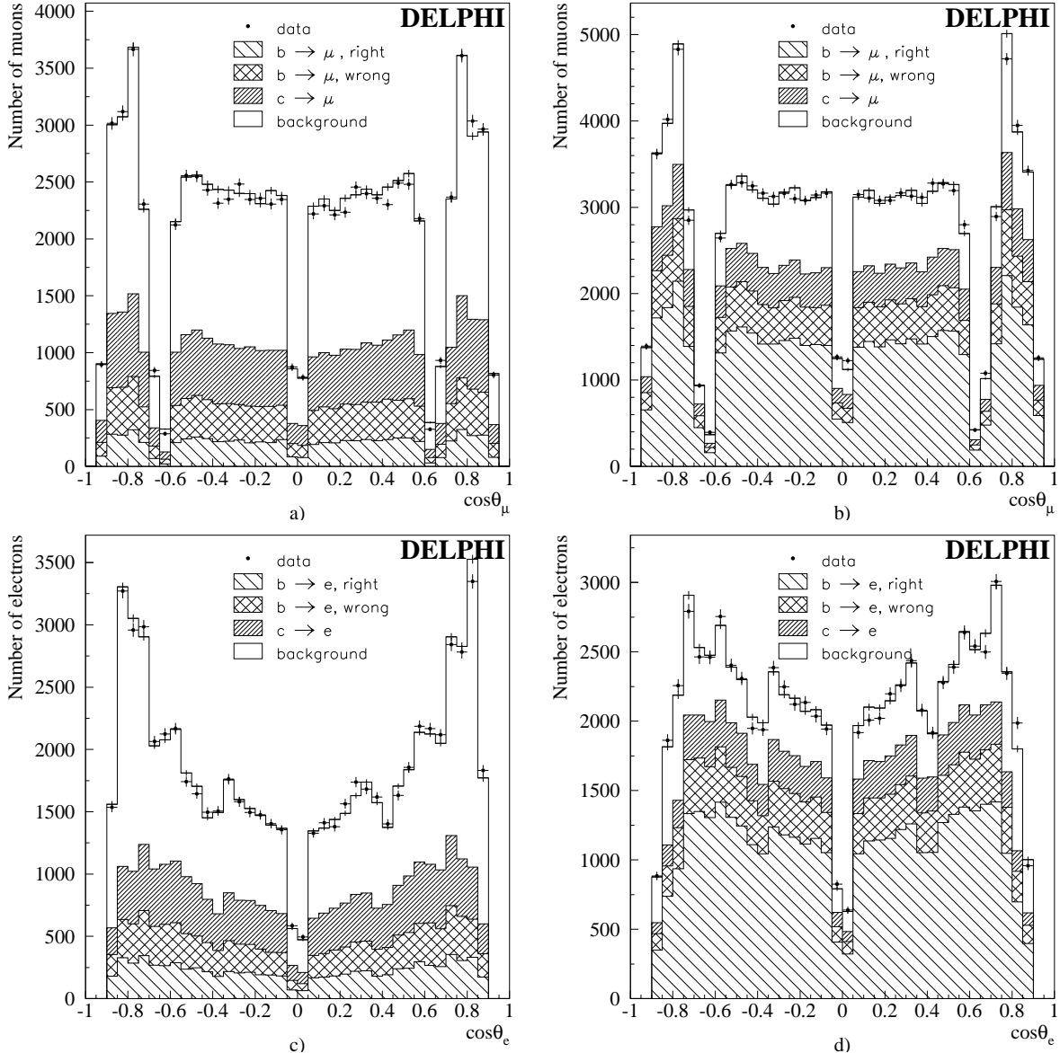
Figure 1: \cos\theta distribution for muon, upper plots, and electron, lower plots, candidates. The lepton candidates have p_T < 0.7 GeV/c in a),c) and p_T > 0.7 GeV/c in b),d) corresponding to samples enriched in background and signal respectively. The “ b \rightarrow \mu/e right (wrong)” samples correspond to leptons with the same (opposite) sign as the primary b parton (see Section 6.1). Converted photons cause the strong \cos\theta_e dependence of the background in the c) plot. Only the statistical errors are quoted in these plots. The systematics on the samples composition considered in the text are enough to cover the few discrepancies observed between the data and the simulation.
