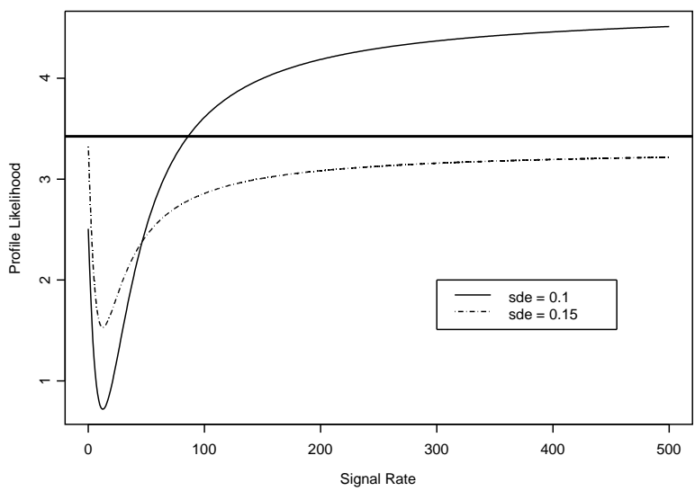
Figure 3: An illustration of why the profile likelihood method does sometimes not return a limit. Here x = 5 , y = 2.5 , \sigma_b = 0.4 and z = 0.2 . If \sigma_e = 0.1 the curve moves above the required level ( for a 90% confidence interval) and the upper limit is 85.9 but if \sigma_e = 0.15 the curve stays below the level and no limit is found.
