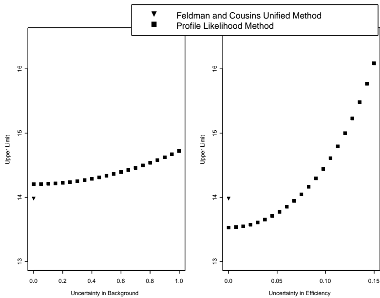
Figure 6: Upper limits as a function of the uncertainties. In both graphs the background and the efficiency are modeled as Gaussians. In the left panel we have the case x = 5 , y = 3 , z = 0.5 , \sigma_e = 0.1 and the uncertainty in the background goes from 0.0 to 1.0. In the right panel we have the case x = 5 , y = 3 , z = 0.5 , \sigma_b = 0.75 and the uncertainty in the efficiency goes from 0.0 to 0.15. We have added the limits derived from Feldman and Cousins unified method which ignores the uncertainties.
