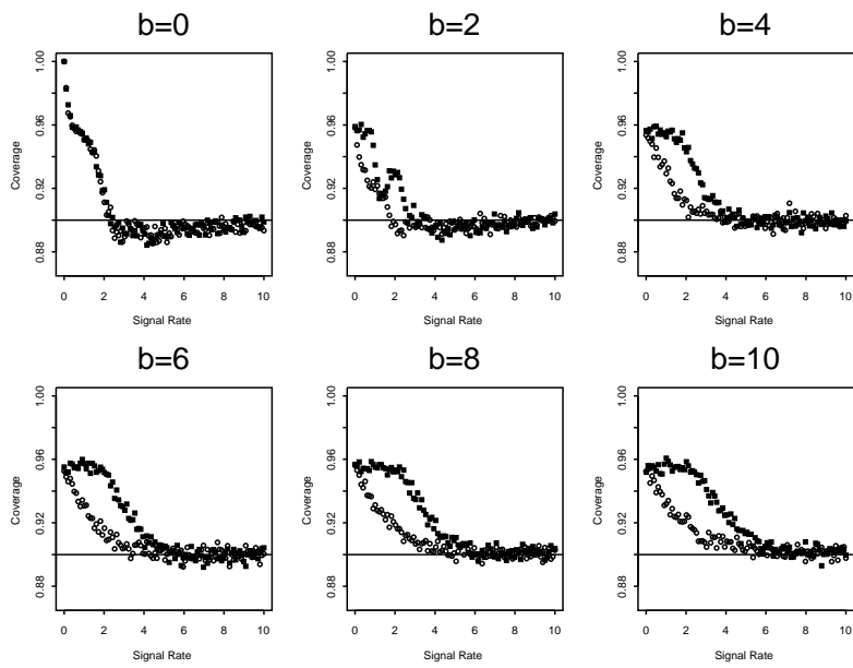
Figure 4: 90% coverage graphs when the signal and the background are modeled as Poisson and the efficiency is modeled as a Binomial with \tau = 3.5 , e = 0.85 and m = 100 . The empty circles show the coverage using the unbounded likelihood method and the solid squares show the coverage using the bounded likelihood method.
