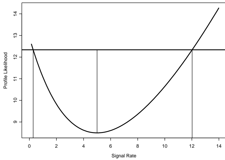
Figure 1: Example of the -2 \log \lambda curve. This is the case x = 8 , y = 15 and \tau = 5.0 . We find the 95% confidence interval to be (0.28, 12.02) .
