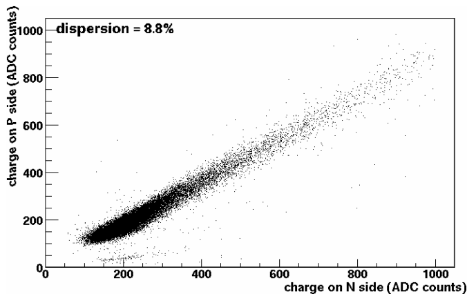
Figure 13: Charge matching of SNC0003.
