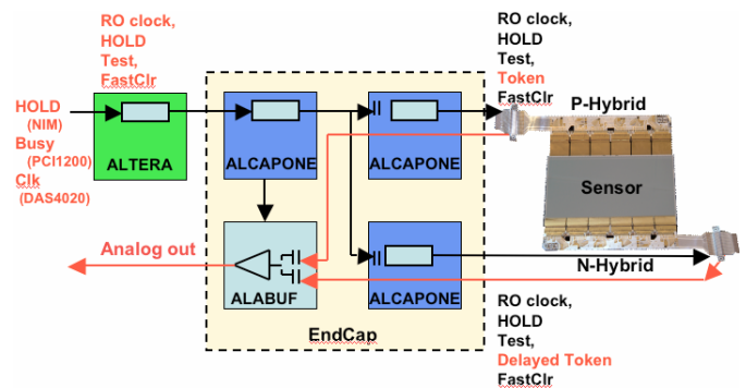
Figure 6: The module readout bloc diagram.
