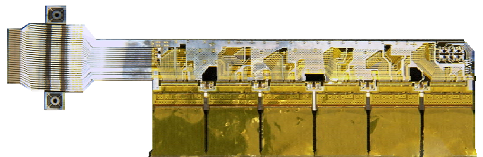
Figure 4: The hybrid supporting the FEE for 768 analogue channels.
