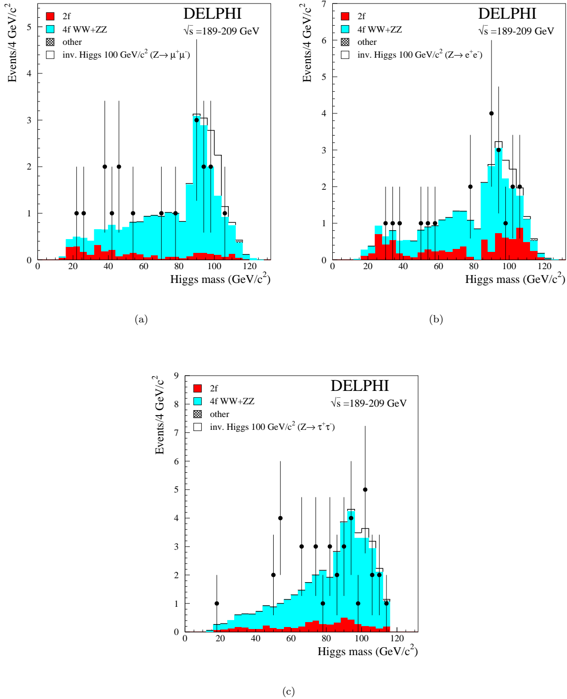
Figure 11: Leptonic channels: Reconstructed Higgs boson mass in (a) the H\mu^+\mu^- channel, (b) the H e^+e^- channel and (c) the H\tau^+\tau^- channel for 189 to 209 GeV after the final selection. The white histogram corresponds to a Higgs boson with 100 GeV/c 2 mass decaying to 100% into invisible modes.
