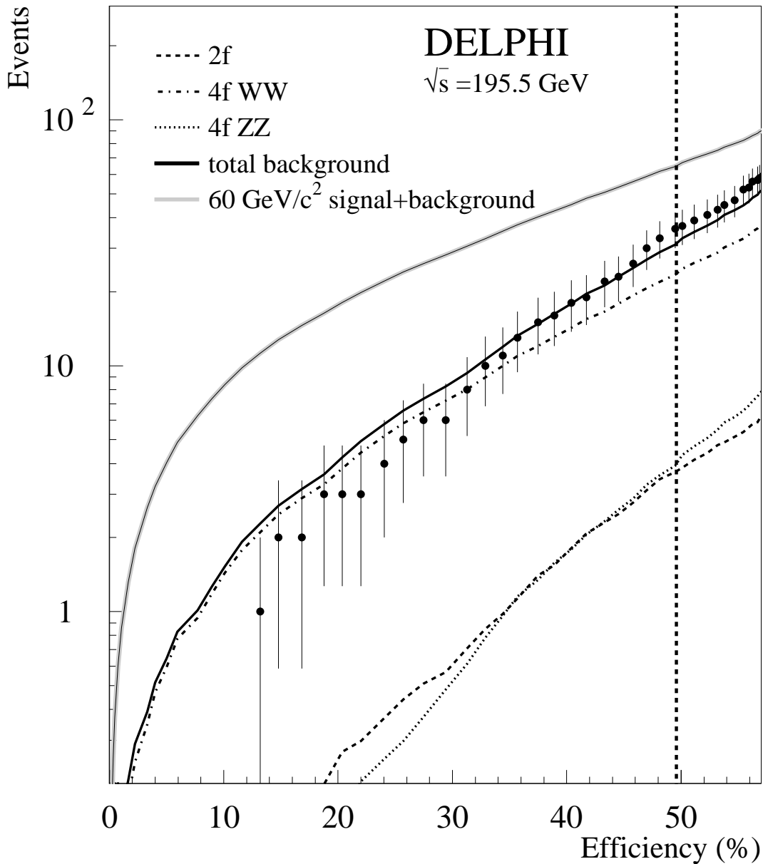
Figure 7: Hadronic channel low mass analysis: Data and expected background for the 195.5 GeV centre-of-mass energy as a function of the efficiency for an invisibly decaying Higgs boson of 60 \text{ GeV}/c^2 . The lines show number of events from the most important background reactions and the solid black line shows the sum of all the background processes. In addition the grey line shows the expectation for a 60 \text{ GeV}/c^2 Higgs signal added on top of the background. The vertical dashed line indicates the final cut chosen to maximise the sensitivity.
