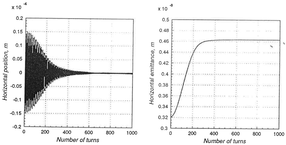
Figure 3: Left) oscillations of the beam centroid after an initial beam displacement of 1 sigma, right) growth of the relative-to-centroid beam emittance after an initial beam displacement of 1 sigma. No compensation.
