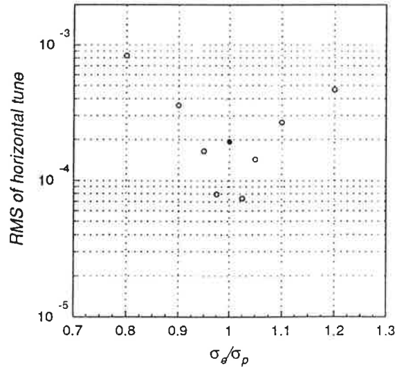
Figure 10: RMS of horizontal tune distribution of the beam particles versus the ratio of the electron to proton bunch sigmas (white circles). Black circle presents the best result for a cylindrical electron bunch (with r_e=1.3\sigma_p and Q_e=0.6Q_p ).
