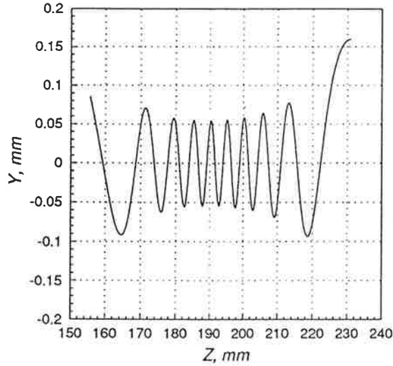
Figure 11: The trajectory of a 10 keV electron with an impact parameter of 160 \mu\text{m} colliding with a proton bunch, Z-Y view. The proton bunch is moving to the right, and the electron is moving to the left. Plus/minus 3\sigma of the proton bunch charge distribution in Z-direction is treated by the tracing code.
