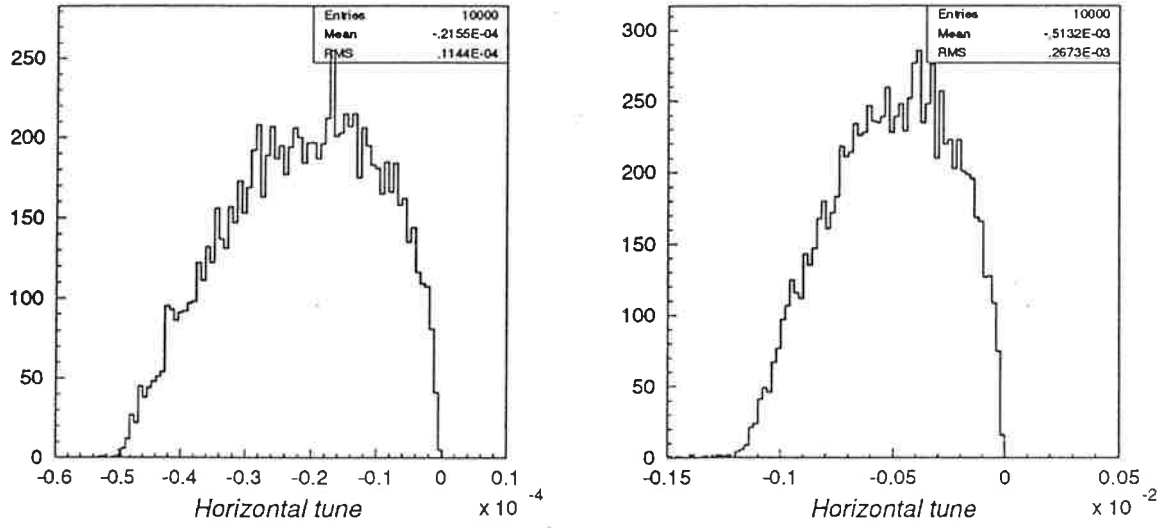
Figure 6: Horizontal tune distribution of beam particles. Left) displacement of the compensating electron beam of 0.1 \sigma , right) displacement of the compensating electron beam of 0.5 \sigma .
