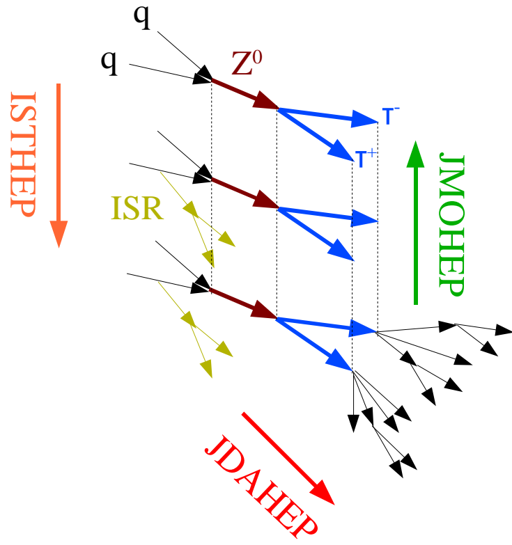
Figure 3: The usage of JMOHEP and JDAHEP pointers in PYTHIA with MSTP(128)=0 setting. While PYTHIA keeps the JDAHEP entries to point in the direction of event evolution, the JMOHEP is used to point to the copies of a particle produced when perturbative effects, such as initial state radiation (ISR) or \tau decays are added; the particle copies at different stages of event simulation are consistently distinguished by the ISTHEP tags.
