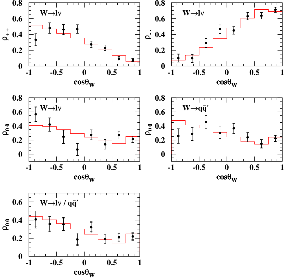
Figure 1: Luminosity-weighted averages of the diagonal elements of the SDM as functions of \cos\theta_W . The points show the data after detector and bias corrections. The inner error bars show the statistical uncertainties and the outer error bars show the total uncertainties including both the statistical and systematic contributions. The histograms show the generator-level Kandy MC prediction. The figures in the top row show \rho_{++} and \rho_{--} for leptonically decaying W bosons. The figures in the middle row show \rho_{00} for leptonically decaying W bosons and hadronically decaying W bosons separately. The figure in the bottom row shows \rho_{00} with the leptonic and hadronic decay modes combined. By construction, the diagonal elements of the SDM are related to each other by the normalisation condition \rho_{++} + \rho_{--} + \rho_{00} = 1 , but have not been individually constrained to the physically-allowed region between zero and one.
