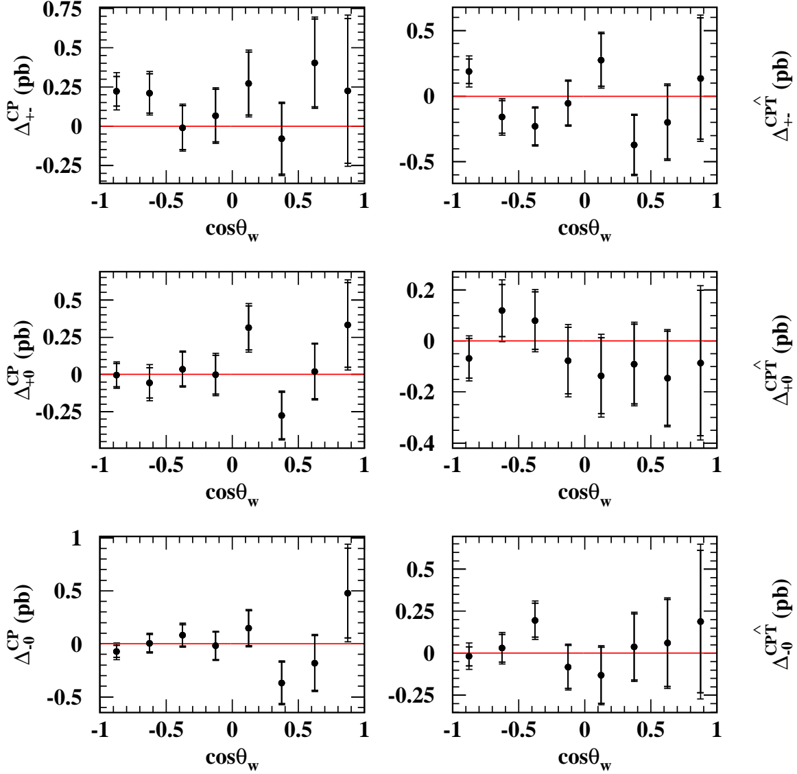
Figure 3: The luminosity-weighted average of the CP-odd and \text{CPT} -odd observables of section 2.4, where the average is over the eight nominal centre-of-mass energies and over the \cos\theta_w bin width. The observables are measured in units of picobarns and shown as functions of \cos\theta_w . The points show the data after detector correction. The inner error bars show the statistical uncertainties and the outer error bars show the total uncertainties including both the statistical and systematic contributions. The solid lines show the SM tree-level prediction.
