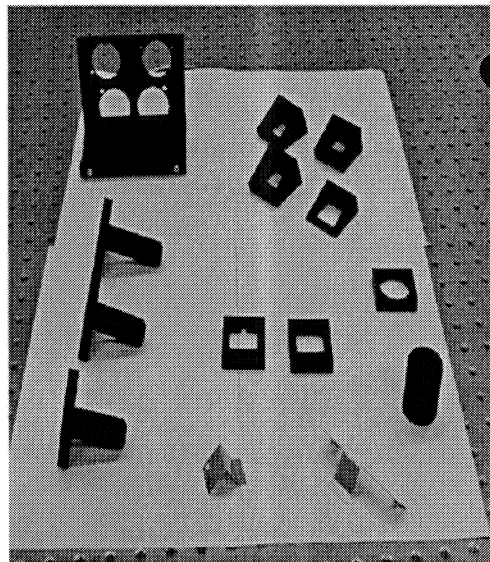
Fig. 9: This picture shows most of the mechanical pieces needed to build a praxial sensor. To ensure the quality of the assembly all elements are screwed and glued on the mechanical support (top left of this picture). The optical elements and their plastic covers are not shown. The assembly of the 2010 praxial elements has started in April 2003. The calibration of all praxial elements will take 17 months.
