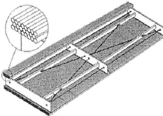
Fig. 2: This drawing shows a Monitored Drift Tube chamber (MDT). A MDT is made of 100 to 300 individual drift tubes, each 3\text{mm} in diameter, and assembled in two times three layers separated by a mechanical support. The sizes of MDTs vary from 1.5 \times 2\text{m}^2 to 2.5 \times 5\text{m}^2 .
