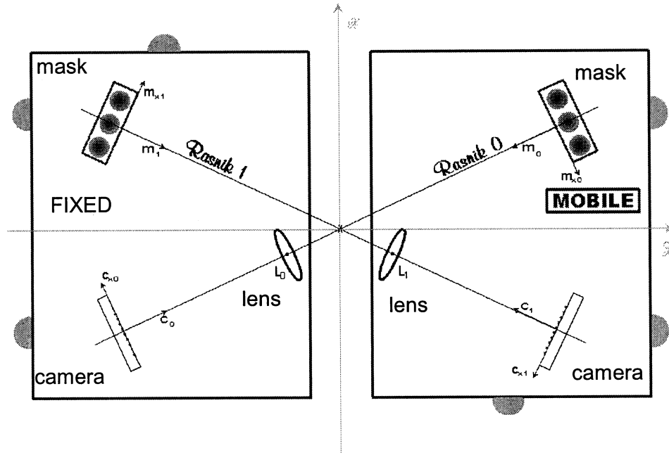
Fig. 4: Drawing of the praxial sensor. One clearly sees on this top view the two crossed Rasnik. During the calibration procedure, the element on the left, called “fixed”, is the reference whereas the element on the right, called “mobile”, is positioned at different known positions thanks to the six stages of the test bench (see text for the calibration procedure). The distance between the camera and the lens is \sim 70\text{mm} .
