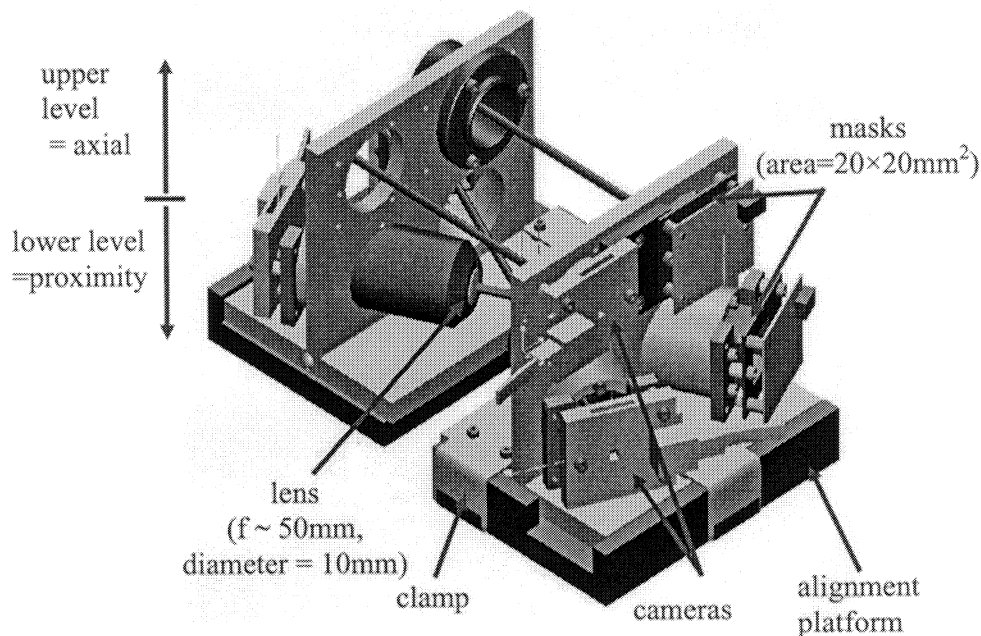
Fig. 3: The praxial sensor is made of two different elements and uses two crossed Rasnik at their "lower" level. The upper part of the sensor corresponds to the axial alignment which is used to unite a complete layer of MDT chambers (not describe in this paper). One of these two elements is on a chamber and the other one is on the neighbouring chamber. Each element is positioned on the MDT chamber through an alignment platform.
