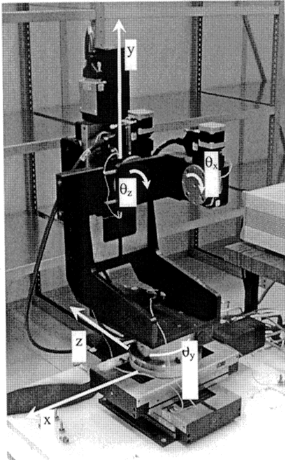
Six stage elements: three for rotations and three for translations.
