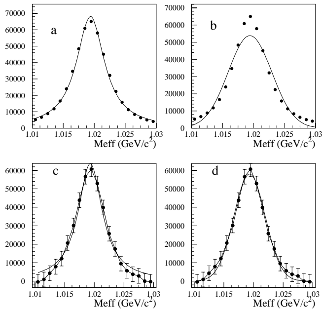
Figure 6: Signal of \phi meson after subtraction of the combinatorial background ( a and b - the explicit background, c and d - the one obtained by the polynomial fit). The curves are the fit results ( a and c - Breit-Wigner, b and d - Gaussian).
