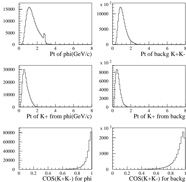
Figure 4: Different kinematical variable distributions for K^+K^- pairs and individual K^+ (see text).
