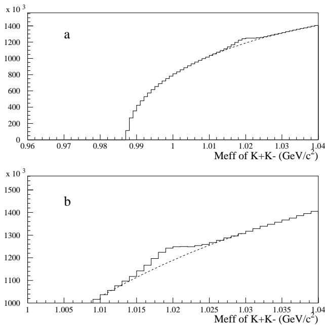
Figure 5: The same spectra as in Fig.3 but after the cut (see text). The curves are the result of combinatorial background fit by the polynomial (p2) function.
