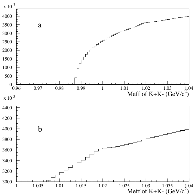
Figure 3: Spectrum of K^+K^- effective mass before any cuts ( a - full spectrum, b - an enlarged view of \phi resonance).
