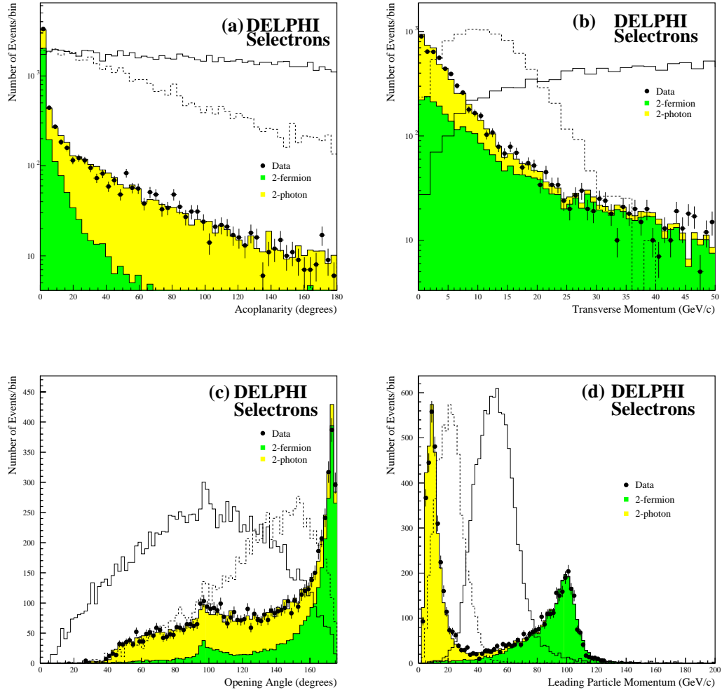
Figure 1: Comparison of data and simulation in the selectron channel at preselection level. The dots with error bars show the data, shaded histograms show the simulation. Plots include data taken in the year 2000 when the DELPHI detector was fully operational. The plots show: (a) the acoplanarity, (b) the transverse momentum, (c) the opening angle, (d) the momentum of the leading charged particle. Possible signals corresponding to the mass combinations M_{\tilde{e}}=90 \text{ GeV}/c^2, M_{\tilde{\chi}_1^0}=10 \text{ GeV}/c^2 (solid) and M_{\tilde{e}}=50 \text{ GeV}/c^2, M_{\tilde{\chi}_1^0}=40 \text{ GeV}/c^2 (dashed) are shown by the superimposed open histograms. The signal normalisation is arbitrary.
