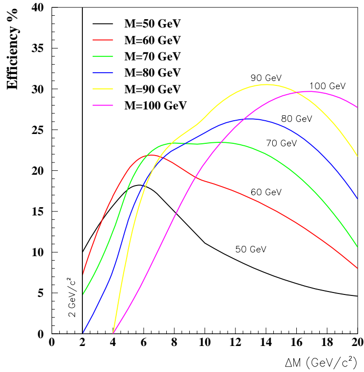
Figure 22: Signal efficiency of the stop search in the nearly degenerate scenario for different mass hypothesis as a function of \Delta M = M_{\tilde{t}_1} - M_{\tilde{\chi}_1^0} , for \sqrt{s} = 189 and 206 GeV.
