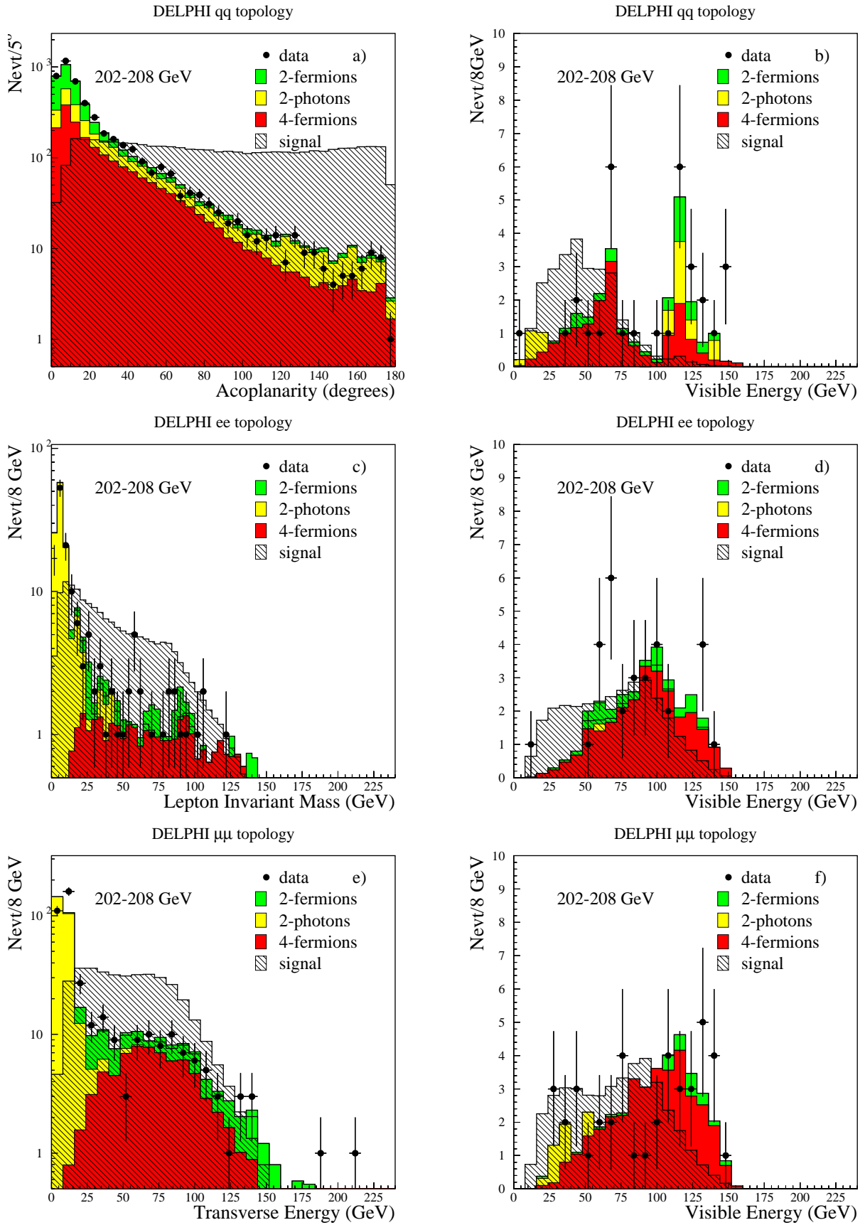
Figure 10: On the left the comparison between the real and simulated data is shown at preselection level for different variables for the q\bar{q} , ee , and \mu\mu topologies in the neutralino search. On the right the visible energy distribution is shown for the events selected at the final stage, after the likelihood selection. The signal distribution contains the contribution of all generated mass combinations and is arbitrarily normalised.
