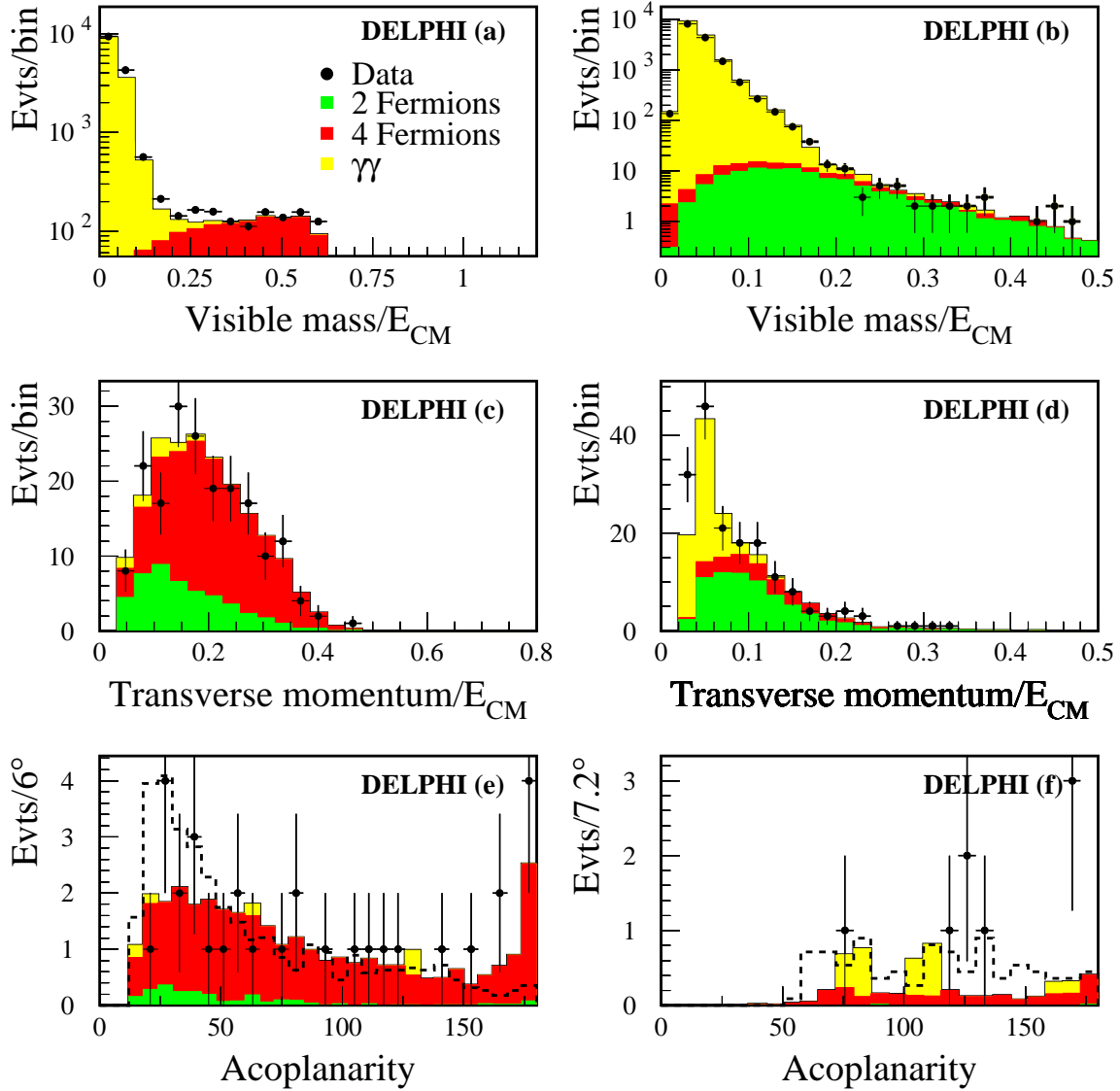
Figure 13: Comparison of real data from 1999 ( \sqrt{s} in the range 192–202 GeV) and simulation for the neutralino multilepton search (a,c,e) and asymmetric tau search (b,d,f), at the preselection (a,b), intermediate (c,d), and final selection (e,f) stages. The dashed line in (e) shows the multilepton signal expected for \tilde{\chi}_3^0 \tilde{\chi}_2^0 production with \tilde{\chi}_3^0 \rightarrow \tilde{\chi}_2^0 \ell^+ \ell^- and \tilde{\chi}_2^0 decaying to \tilde{\chi}_1^0 \ell^+ \ell^- where M_{\tilde{\chi}_3^0} = 103 \text{ GeV}/c^2 , M_{\tilde{\chi}_2^0} = 51 \text{ GeV}/c^2 and M_{\tilde{\chi}_1^0} = 45 \text{ GeV}/c^2 . In (f) the dashed line shows the tau cascade signal for \tilde{\chi}_2^0 \tilde{\chi}_1^0 production with \tilde{\chi}_2^0 \rightarrow \tilde{\tau} \tau and \tilde{\tau} \rightarrow \tilde{\chi}_1^0 \tau where M_{\tilde{\chi}_2^0} = 75 \text{ GeV}/c^2 , M_{\tilde{\tau}} = 44 \text{ GeV}/c^2 and M_{\tilde{\chi}_1^0} = 37.5 \text{ GeV}/c^2 . The signals are normalised to a cross-section of 0.4 pb.
