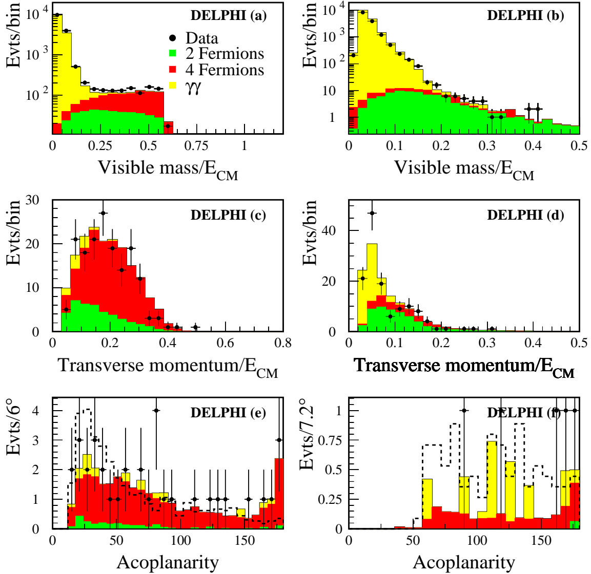
Figure 14: Comparison of real data from 2000 ( \sqrt{s} in the range 204–208 GeV) and simulation for the neutralino multilepton search (a,c,e) and asymmetric tau search (b,d,f), at the preselection (a,b), intermediate (c,d), and final selection (e,f) stages. The dashed line in (e) shows the multilepton signal expected for \tilde{\chi}_3^0\tilde{\chi}_2^0 production with \tilde{\chi}_3^0 \rightarrow \tilde{\chi}_2^0\ell^+\ell^- and \tilde{\chi}_2^0 decaying to \tilde{\chi}_1^0\ell^+\ell^- where M_{\tilde{\chi}_3^0}=103 GeV/ c^2 , M_{\tilde{\chi}_2^0}=51 GeV/ c^2 and M_{\tilde{\chi}_1^0}=45 GeV/ c^2 . In (f) the dashed line shows the tau cascade signal for \tilde{\chi}_2^0\tilde{\chi}_1^0 production with \tilde{\chi}_2^0 \rightarrow \tilde{\tau}\tau and \tilde{\tau} \rightarrow \tilde{\chi}_1^0\tau where M_{\tilde{\chi}_2^0}=75 GeV/ c^2 , M_{\tilde{\tau}}=44 GeV/ c^2 and M_{\tilde{\chi}_1^0}=37.5 GeV/ c^2 . The signals are normalised to a cross-section of 0.4 pb.
