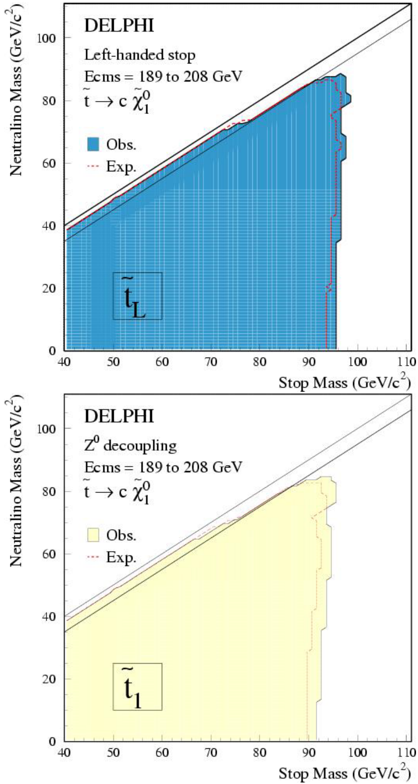
Figure 23: Excluded regions for the stop search in the plane (M_{\tilde{t}_1}, M_{\tilde{\chi}_1^0}) for purely left handed stops (top) and for the states at the Z decoupling (bottom). The shaded areas show the observed excluded regions and the lines correspond to the expected exclusions (for a discussion on the low stop mass region see section 6.3).
