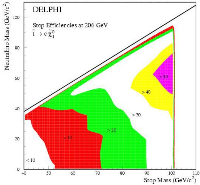
Figure 21: Squark signal detection efficiencies (in %) in the plane (M_{\tilde{q}_1}, M_{\tilde{\chi}_1^0}) in the non-degenerate scenario.
