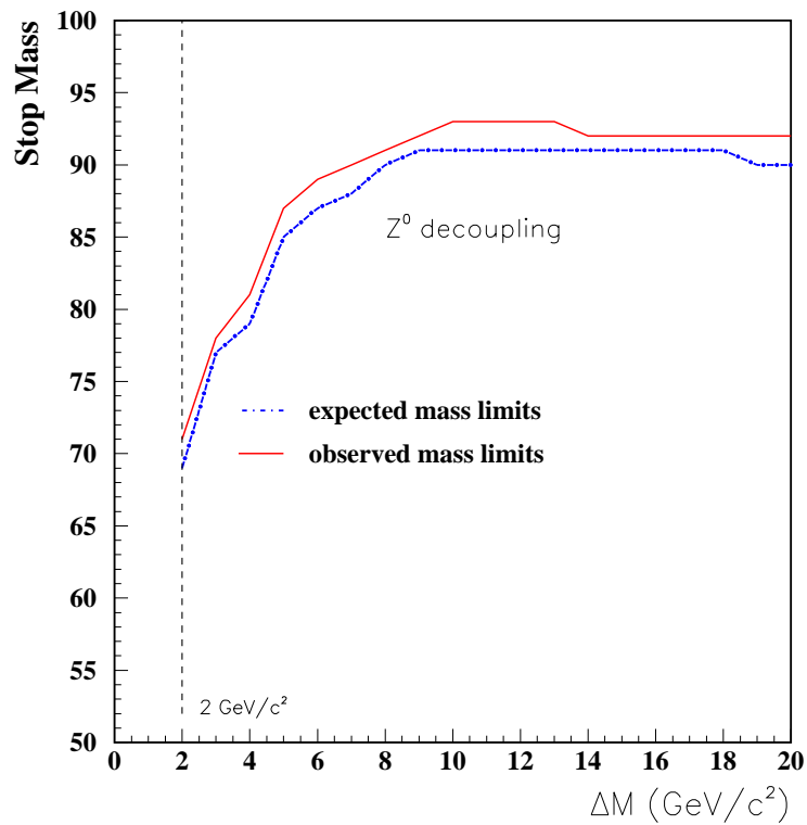
Figure 25: Stop mass limit as a function of \Delta M for a purely left-handed stop and for the stop mixing angle which minimises the cross-section.
