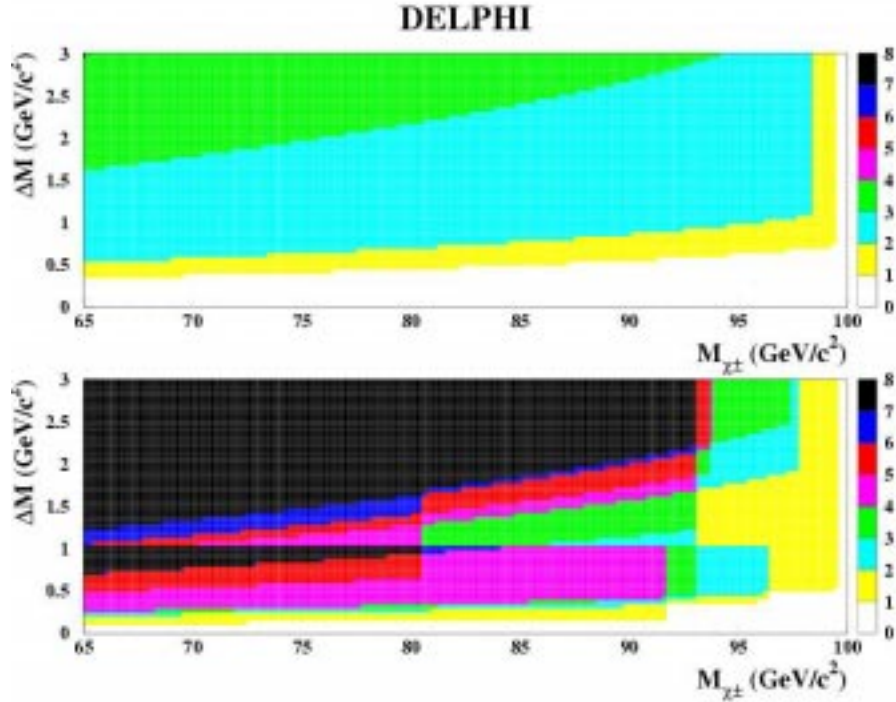
Figure 35: Expected number of background events (top) and number of selected events in the real data (bottom) after the final selection, for the year 2000 data with the TPC fully operational, as function of the points in the plane (M_{\chi_{\pm}}, \Delta M) considered in the chargino search with an ISR photon.
