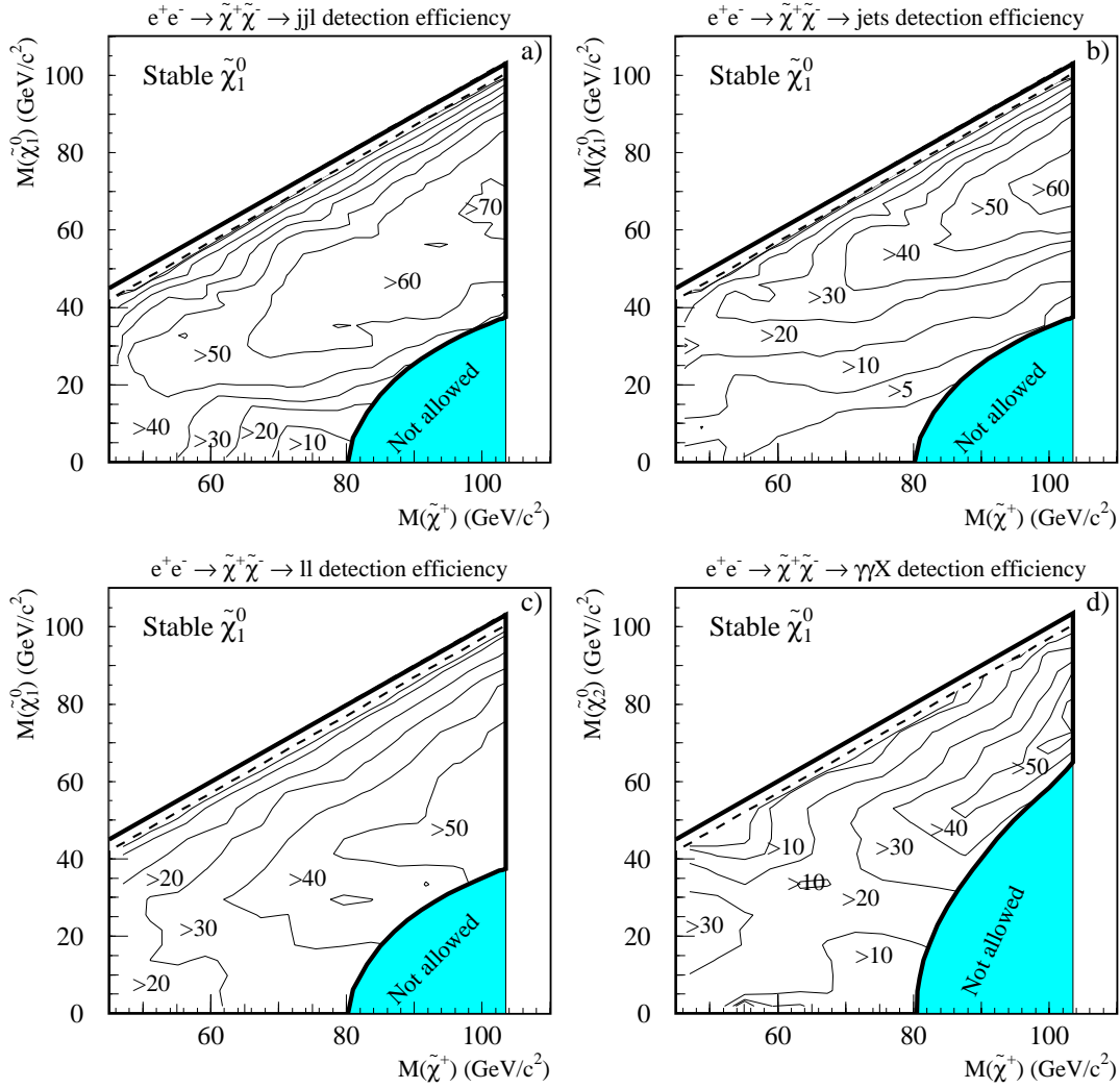
Figure 27: Chargino pair-production detection efficiencies (%) for the four decay channels a) jjl , b) jets , c) ll and d) rad , at 206.5 GeV in the (M_{\tilde{\chi}_\pm}, M_{\tilde{\chi}_0}) plane. TPC sector 6 is off and a stable \tilde{\chi}_1^0 is assumed. The shaded areas are disallowed in the MSSM scheme.
