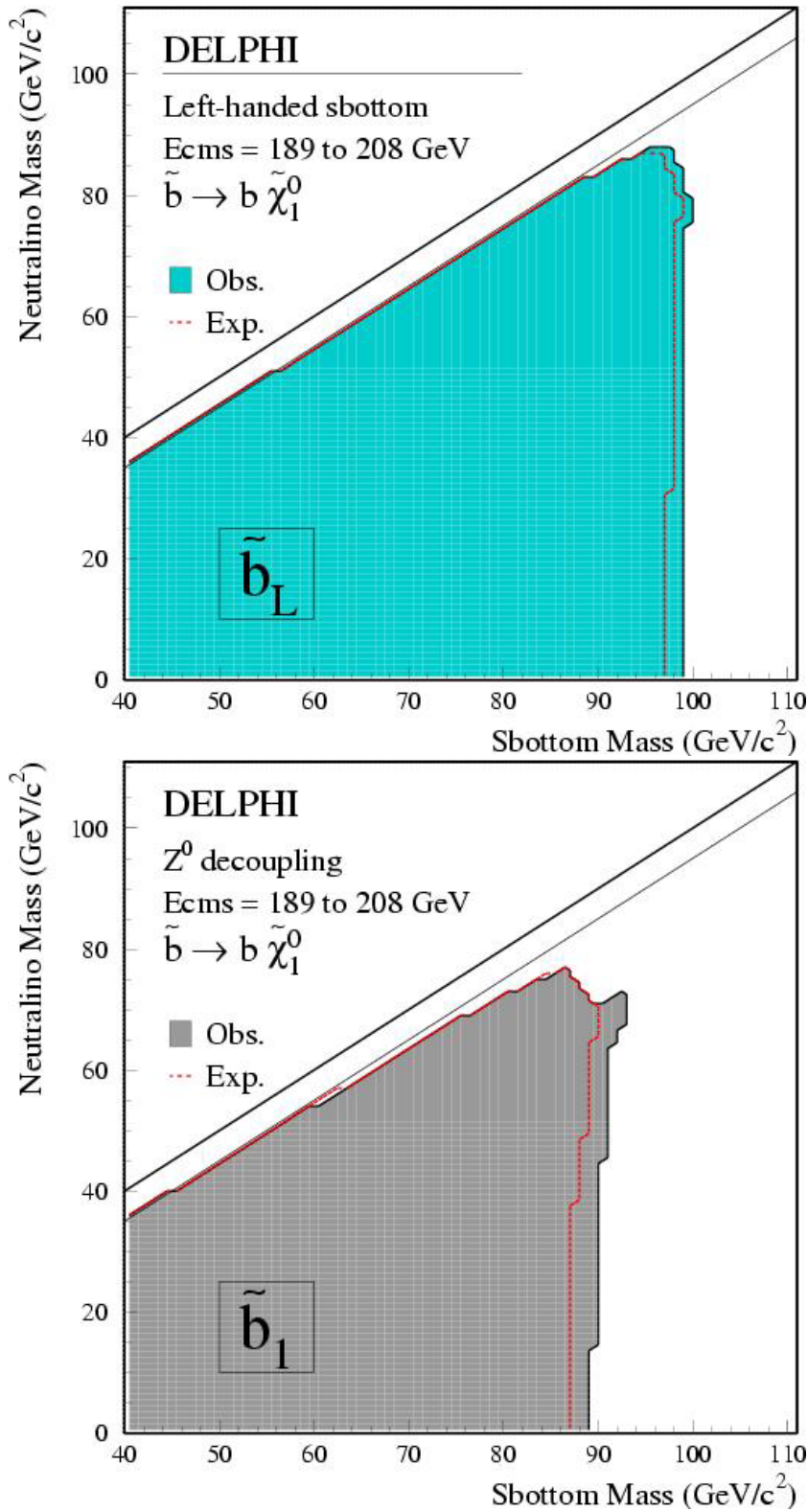
Figure 24: Excluded regions at for the sbottom search in the plane (M_{\tilde{b}_1}, M_{\tilde{\chi}_1^0}) for purely left handed sbottoms (top) and for the states at the Z decoupling (bottom). The shaded areas show the observed excluded regions and the lines correspond to the expected exclusions (for a discussion on the low sbottom mass region see section 6.3).
