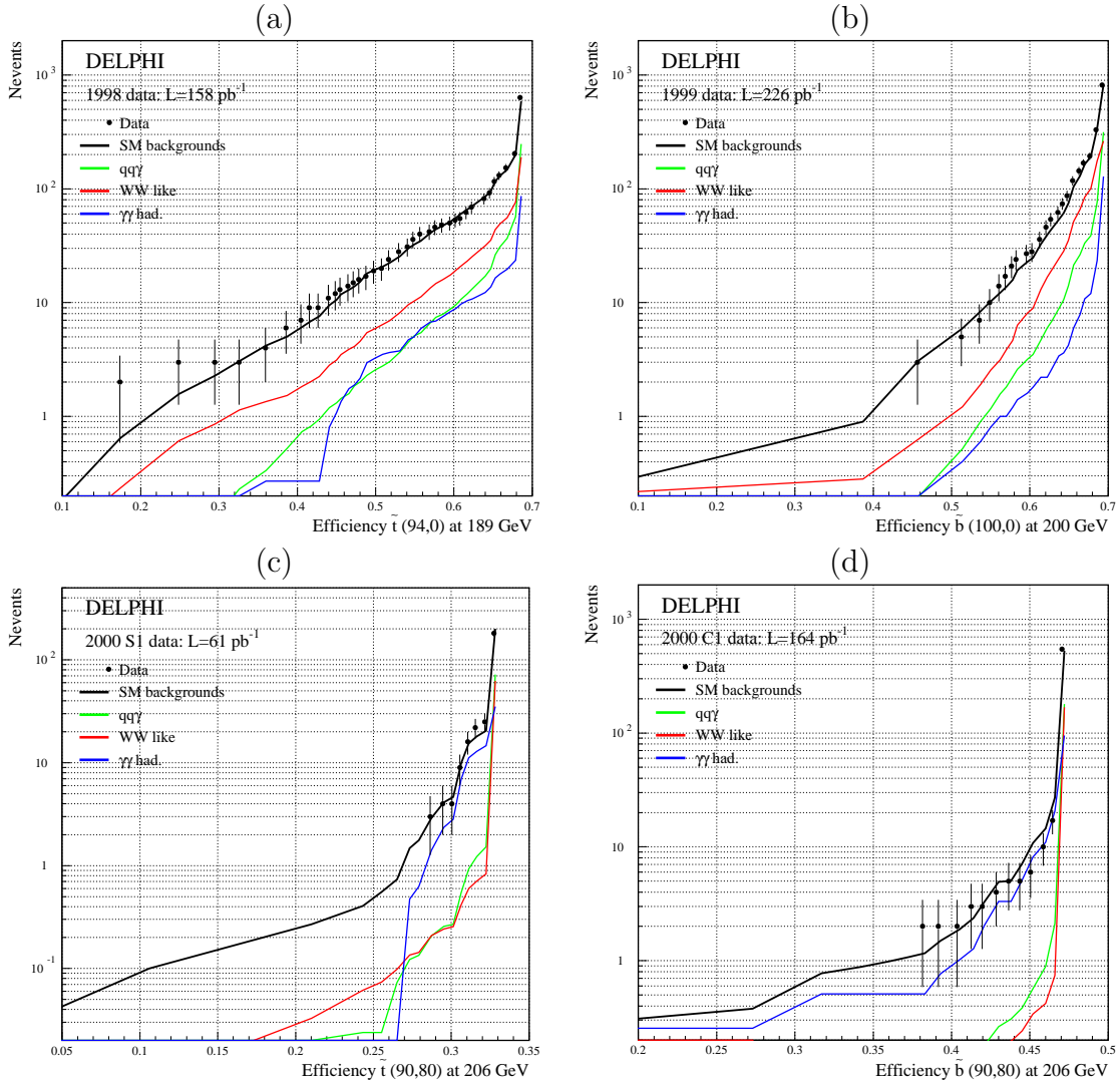
Figure 5: Number of events as a function of the signal detection efficiencies in the non-degenerate squark analysis: (a) 1998 data at 189 GeV: stop analysis for \Delta M > 20 \text{ GeV}/c^2 , (b) 1999 data from 192 to 202 GeV: sbottom analysis for \Delta M > 20 \text{ GeV}/c^2 , (c) 2000 data with TPC sector 6 off: stop analysis for 5 \leq \Delta M \leq 20 \text{ GeV}/c^2 , (d) 2000 data with TPC sector 6 on: sbottom analysis for 5 \leq \Delta M \leq 20 \text{ GeV}/c^2 . The efficiencies are for a given combination of squark and LSP masses, indicated in the parentheses.
