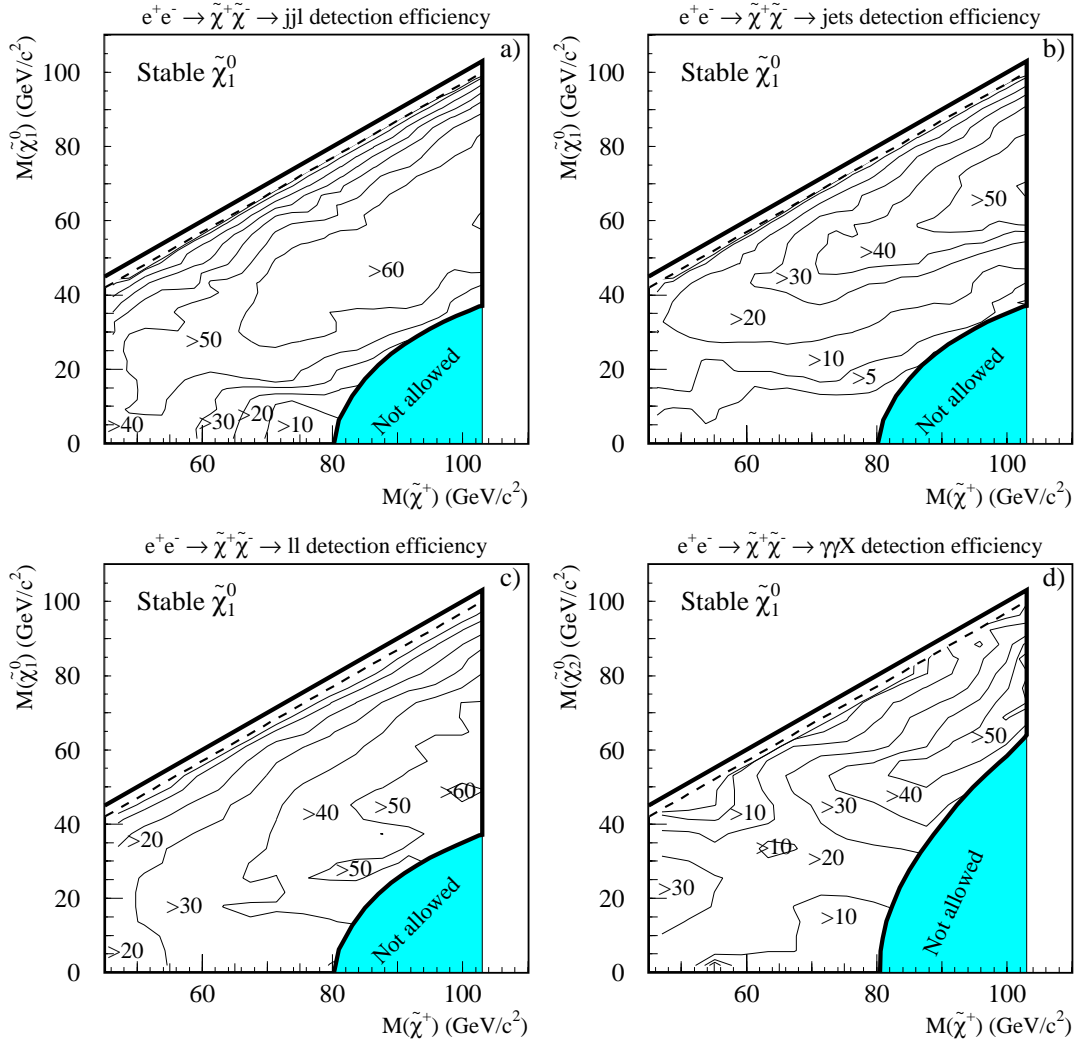
Figure 26: Chargino pair-production detection efficiencies (%) for the four decay channels a) jjl , b) jets , c) ll and d) rad , at 206 GeV in the (M_{\tilde{\chi}_\pm}, M_{\tilde{\chi}_1^0}) plane. TPC sector 6 is on and a stable \tilde{\chi}_1^0 is assumed. The shaded areas are disallowed in the MSSM scheme.
