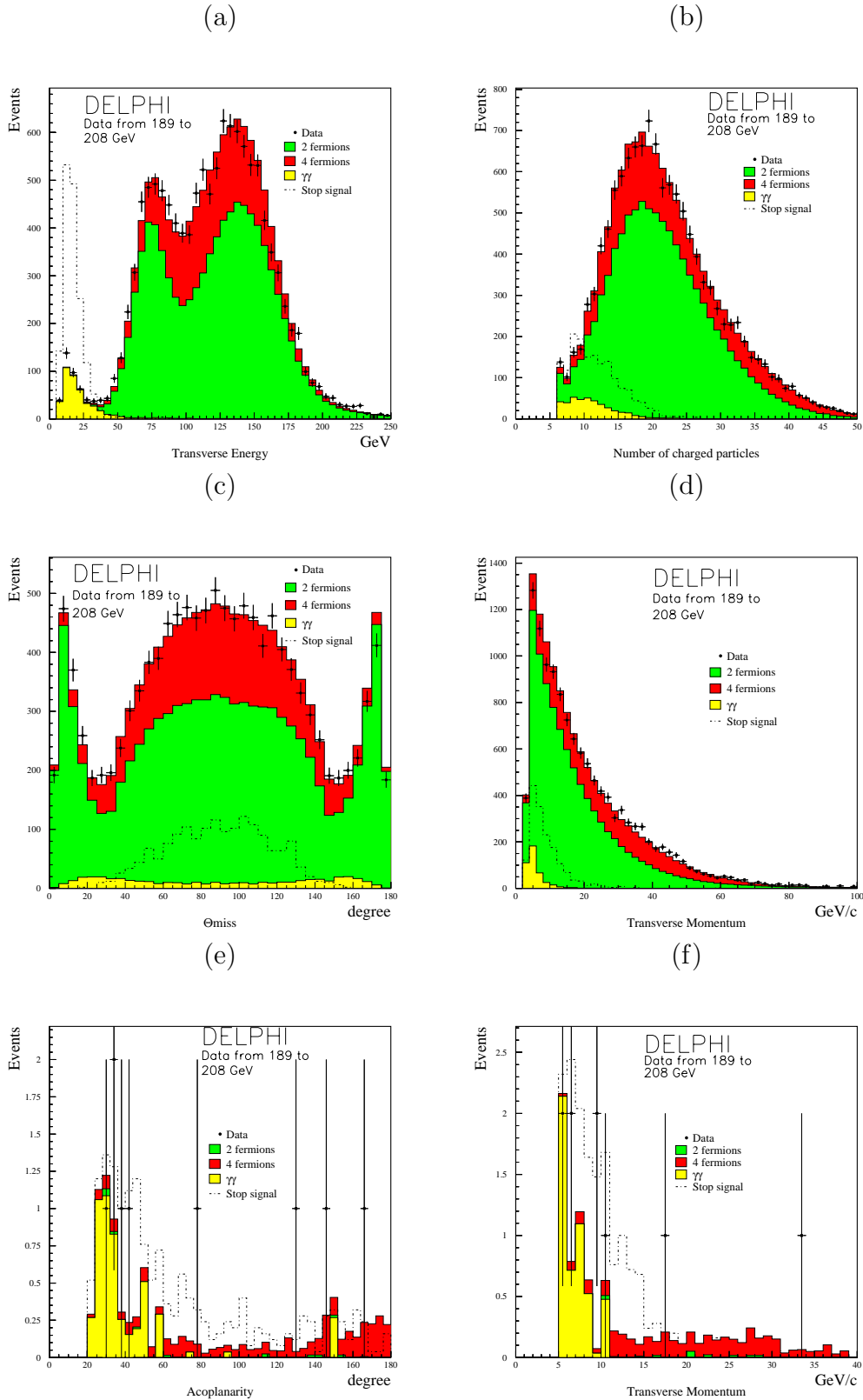
Figure 6: Comparison of data and simulation in the nearly degenerate squark analysis at preselection and final selection level. The distributions of (a) the total transverse energy, (b) total number of charged particles, (c) angle between the missing momentum and the beam axis and (d) transverse momentum are shown at preselection level. At the final selection level the distributions of (e) the acoplanarity and (f) the transverse momentum are shown. All DELPHI data from 189 to 208 GeV is included. A signal corresponding to M_{\tilde{t}} = 60 \text{ GeV}/c^2 and \Delta M = 4 \text{ GeV}/c^2 is also shown (with arbitrary normalisation at preselection level and normalised to a cross-section of 0.16 pb in (e) and (f)).
