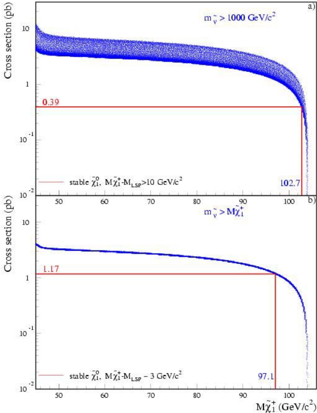
Figure 28: Expected cross-sections in pb at 208 GeV (dots) versus the chargino mass in a) for \Delta M > 10 \text{ GeV}/c^2 and b) for \Delta M \sim 3 \text{ GeV}/c^2 . The spread in the dots originates from the random scan over the parameters \mu and M_2 . A heavy sneutrino ( m_{\tilde{\nu}} > 1000 \text{ GeV}/c^2 ) has been assumed in a) and m_{\tilde{\nu}} > M_{\tilde{\chi}_1^\pm} in b). The minimal cross-sections below the mass limits are indicated by the horizontal lines.
