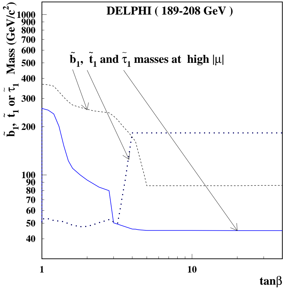
Figure 41: The masses as a function of \tan\beta of the lightest stau (solid curve), stop (dotted curve) and sbottom (dashed curve), at the largest allowed |\mu| for the smallest non-excluded M_2 value. Mass splitting in the stau (sbottom, stop) sector in the form A_\tau - \mu\tan\beta ( A_b - \mu\tan\beta , A_t - \mu/\tan\beta ) was assumed, with A_\tau = 0 ( A_b = A_t = 0 ).
