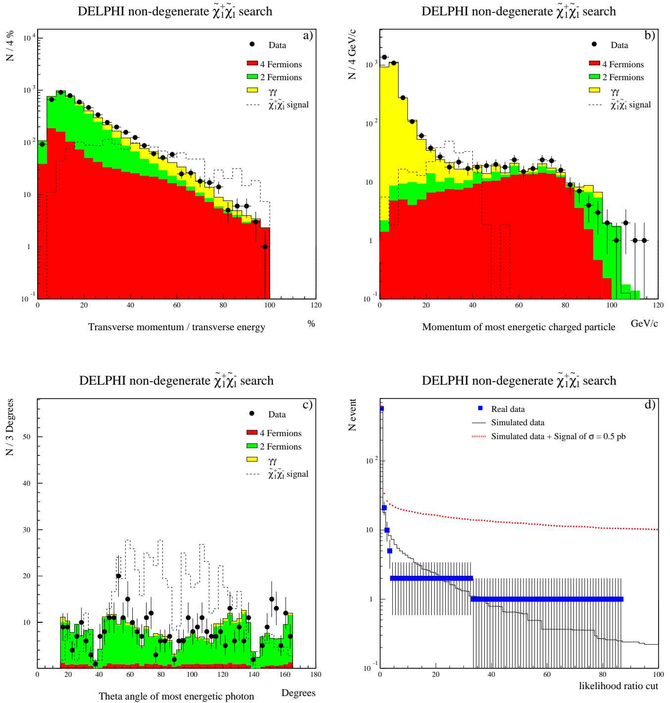
Figure 7: a), b) and c) show comparisons between real data (dots) and simulated background events (histogram) for the jets , ll and rad topologies respectively, using a logical OR of the 6 preselection cut functions of the corresponding topology. The dashed lines indicate how a characteristic chargino signal would appear (arbitrary normalisation). d) shows the number of events selected by the standard chargino analysis as a function of the \mathcal{L}_{\mathcal{R}_{CU\bar{T}}} cut in the jjll topology for 25 \leq \Delta M < 35 \text{ GeV}/c^2 . The squares are the data and the solid line is the background simulation. The dotted curve shows a possible signal, M_{\tilde{\chi}_1^\pm} = 102.8 \text{ GeV}/c^2 , M_{\tilde{\chi}_1^0} = 73 \text{ GeV}/c^2 , of 0.5 pb. In all cases the data collected in the year 2000 with the TPC sector 6 on are shown.
