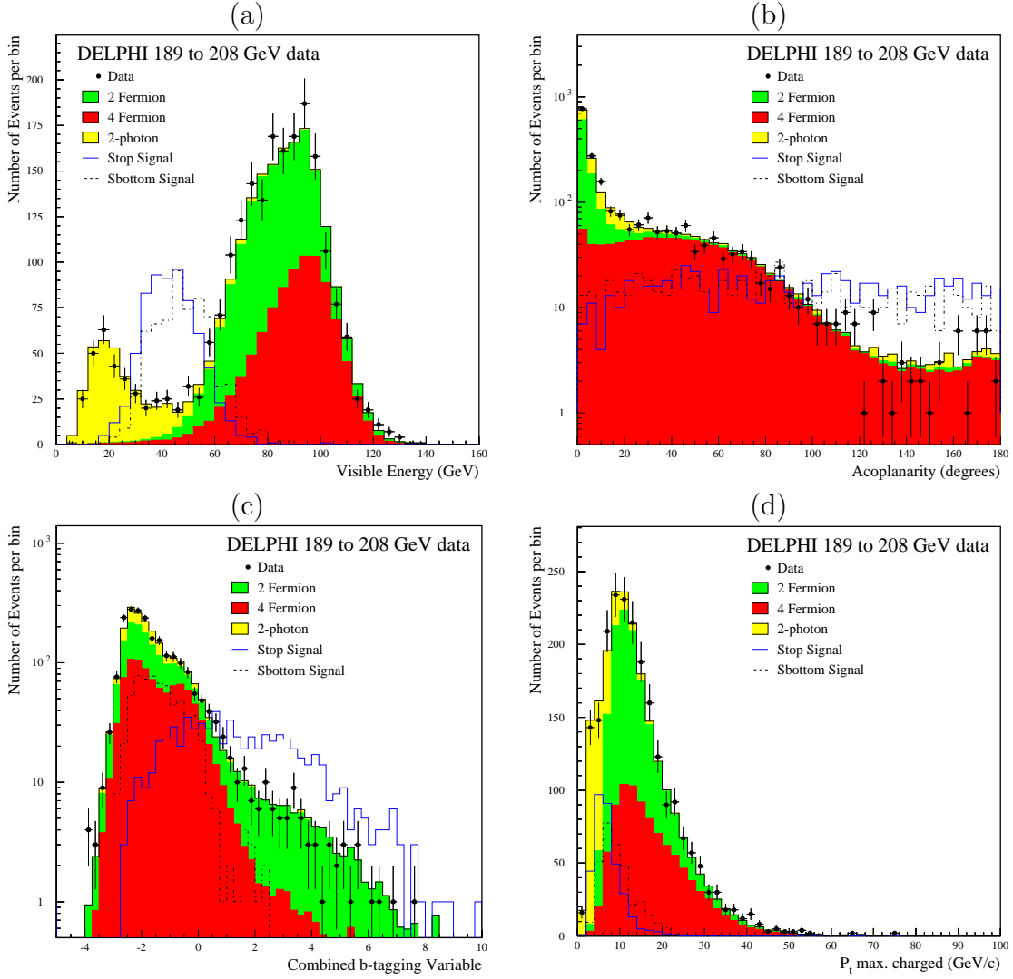
Figure 4: Comparison of data and simulation at the preselection level in the non-degenerate squark analysis. Plots include all DELPHI data from 189 to 208 GeV: (a) visible energy, (b) acoplanarity, (c) combined b-tagging variable, (d) maximal transverse momentum of a charged particle. The expected signal distributions at \sqrt{s} = 200 GeV are shown for one possible stop and sbottom signal ( M_{\tilde{q}}=90 GeV/ c^2 , M_{\tilde{\chi}_1^0} = 60 GeV/ c^2 ), with arbitrary normalisation.
