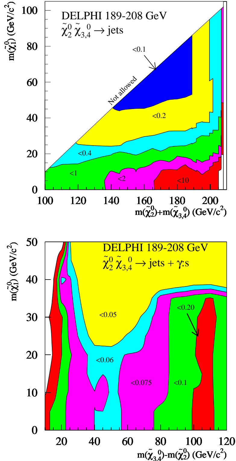
Figure 38: Upper limits on the cross-sections for \tilde{\chi}_2^0 \tilde{\chi}_i^0 production with \tilde{\chi}_i^0 \rightarrow \tilde{\chi}_2^0 q \bar{q} ( i=3,4 ) including data up to \sqrt{s} = 208 GeV. The different shadings correspond to regions where the cross-section limit in picobarns is below the indicated number. The \tilde{\chi}_2^0 was assumed to decay 100% into \tilde{\chi}_1^0 q \bar{q} (left plot), and into \tilde{\chi}_1^0 \gamma (right plot). The limits in the left plot are based on the acoplanar jets and multijets selections, while those in the right plot derive from the search for multijets with photons.
