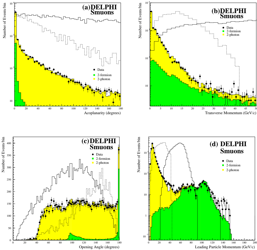
Figure 2: Comparison of data and simulation in the smuon channel at preselection level. The dots with error bars show the data, shaded histograms show the simulation. Plots include data taken in the year 2000 when the DELPHI detector was fully operational. The plots show: (a) the acoplanarity, (b) the transverse momentum, (c) the opening angle, (d) the momentum of the leading charged particle. Possible signals corresponding to the mass combinations M_{\tilde{\mu}}=90 \text{ GeV}/c^2, M_{\tilde{\chi}_1^0}=10 \text{ GeV}/c^2 (solid) and M_{\tilde{\mu}}=50 \text{ GeV}/c^2, M_{\tilde{\chi}_1^0}=40 \text{ GeV}/c^2 (dashed) are shown by the superimposed open histograms. The signal normalisation is arbitrary.
