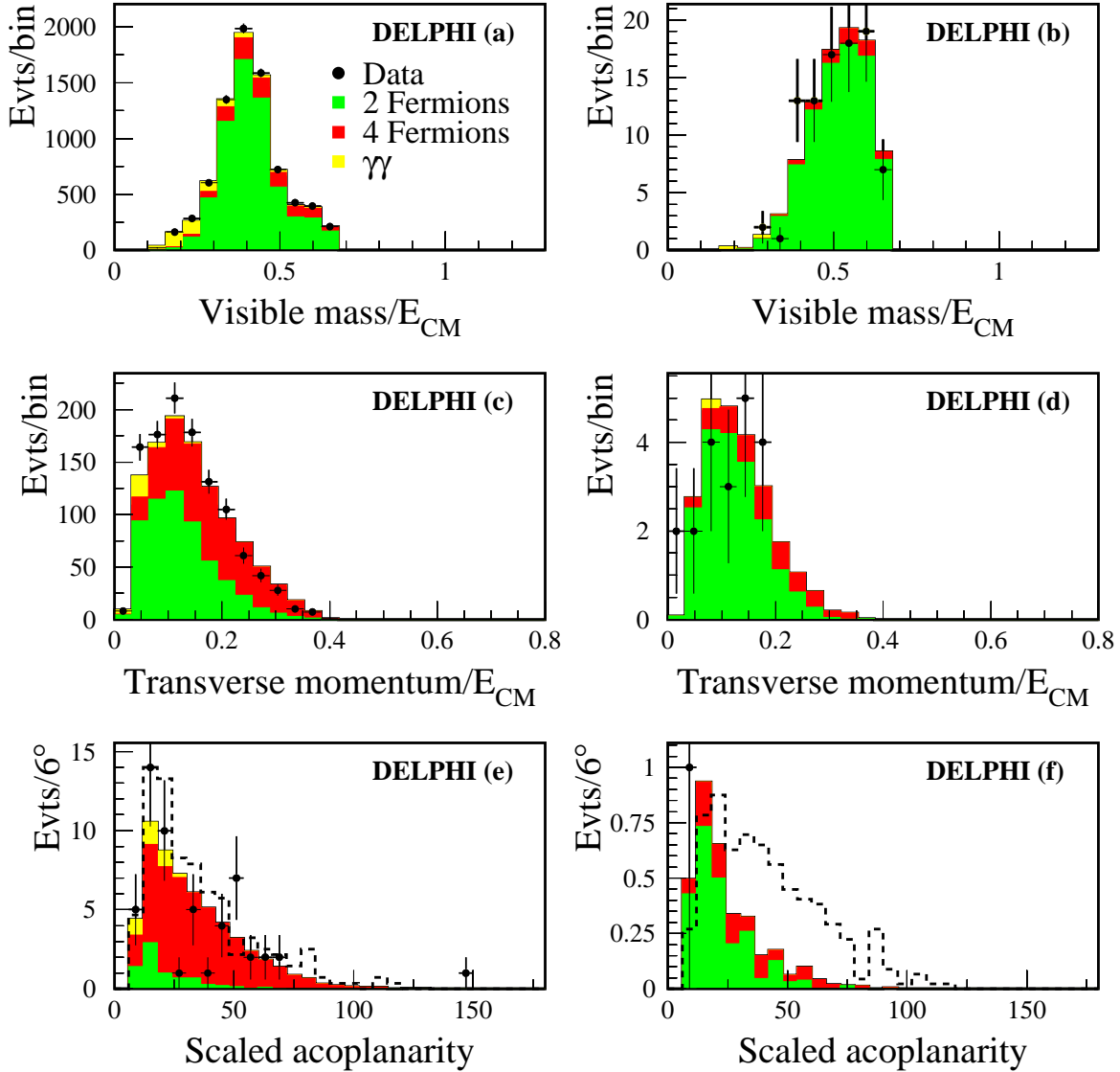
Figure 11: Comparison of real data from 1999 ( \sqrt{s} in the range 192–202 GeV) and simulation for the neutralino multijet selection without photons (a,c,e) and with photons (b,d,f), at the preselection (a,b), intermediate (c,d), and final selection (e,f) stages. The distributions expected for \tilde{\chi}_3^0 \tilde{\chi}_2^0 production with \tilde{\chi}_3^0 \rightarrow \tilde{\chi}_2^0 q \bar{q} and \tilde{\chi}_2^0 decaying to \tilde{\chi}_1^0 q \bar{q} or \tilde{\chi}_1^0 \gamma are shown as dashed histograms where M_{\tilde{\chi}_3^0} = 112 \text{ GeV}/c^2 , M_{\tilde{\chi}_2^0} = 75 \text{ GeV}/c^2 and M_{\tilde{\chi}_1^0} = 41 \text{ GeV}/c^2 . The signals are normalised to cross-sections of 0.8 pb (e) and 0.1 pb (f).
