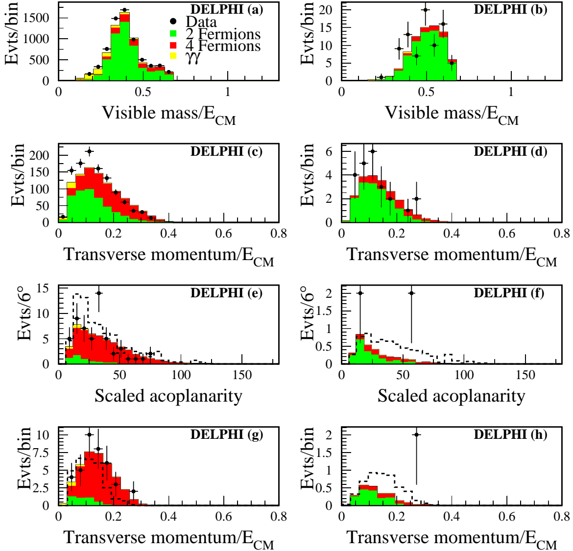
Figure 12: Comparison of real data from 2000 ( \sqrt{s} in the range 204–208 GeV) and simulation for the neutralino multijet selection without photons (a,c,e,g) and with photons (b,d,f,h), at the preselection (a,b),intermediate (c,d), and final selection(e,f,g,h) stages. In (g,h) only the data collected with the TPC sector 6 on are shown. The distributions expected for \tilde{\chi}_3^0\tilde{\chi}_2^0 production with \tilde{\chi}_3^0 \rightarrow \tilde{\chi}_2^0 q \bar{q} and \tilde{\chi}_2^0 decaying to \tilde{\chi}_1^0 q \bar{q} or \tilde{\chi}_1^0 \gamma are shown as dashed histograms where M_{\tilde{\chi}_3^0}=112 GeV/ c^2 , M_{\tilde{\chi}_2^0}=75 GeV/ c^2 and M_{\tilde{\chi}_1^0}=41 GeV/ c^2 . The signals are normalised cross-sections of 0.8 pb (e), 0.1 pb (f,h) and 0.4 pb (g).
