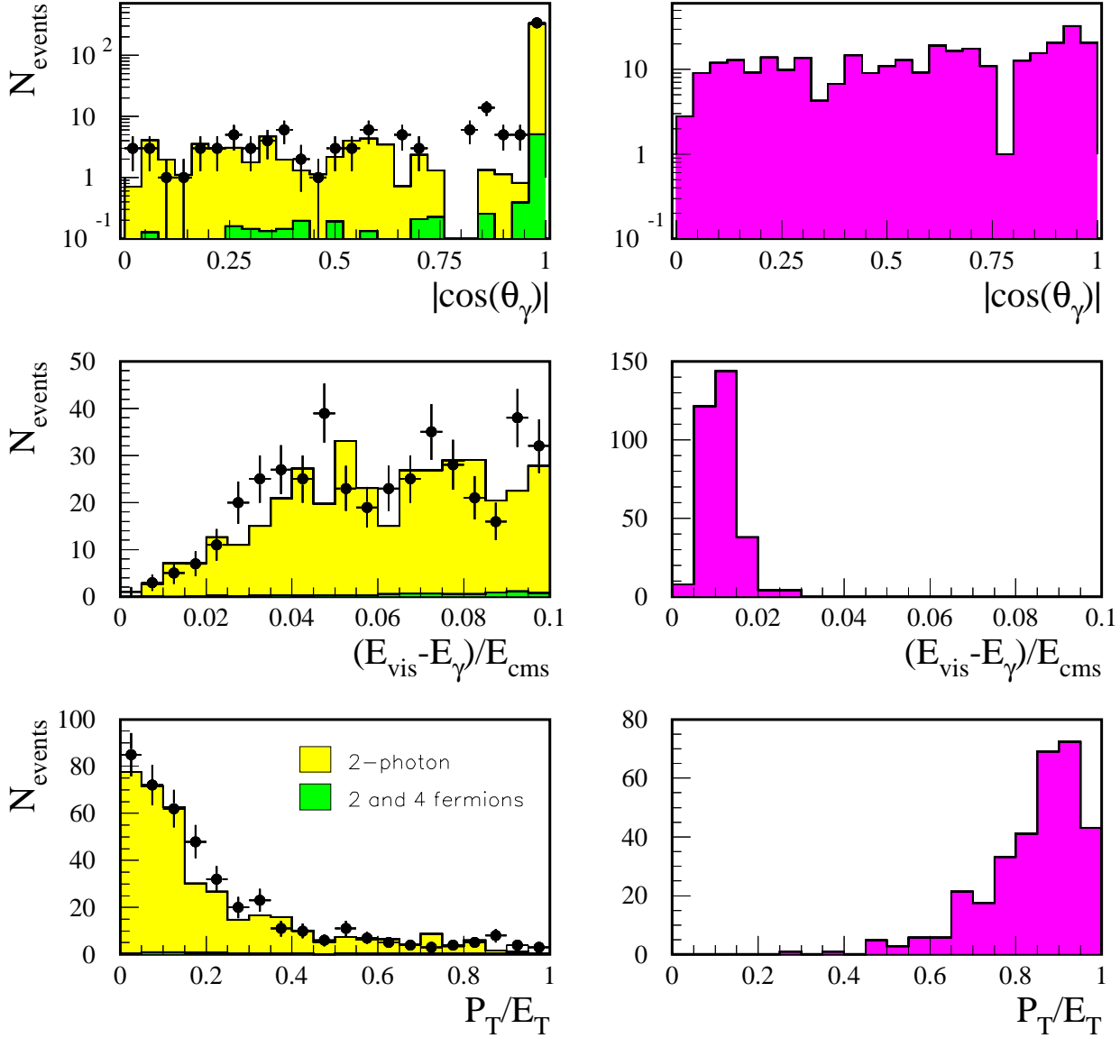
Figure 9: Some of the variables used in the selection for mass-degenerate charginos with an ISR photon tag. In the plots on the left the data (dots) are compared with the SM expectations. On the right, as an example, the corresponding distributions (with arbitrary normalisation) are shown for the signal with M(\tilde{\chi}_1^\pm) = 80 \text{ GeV}/c^2 and \Delta M = 1 \text{ GeV}/c^2 .
