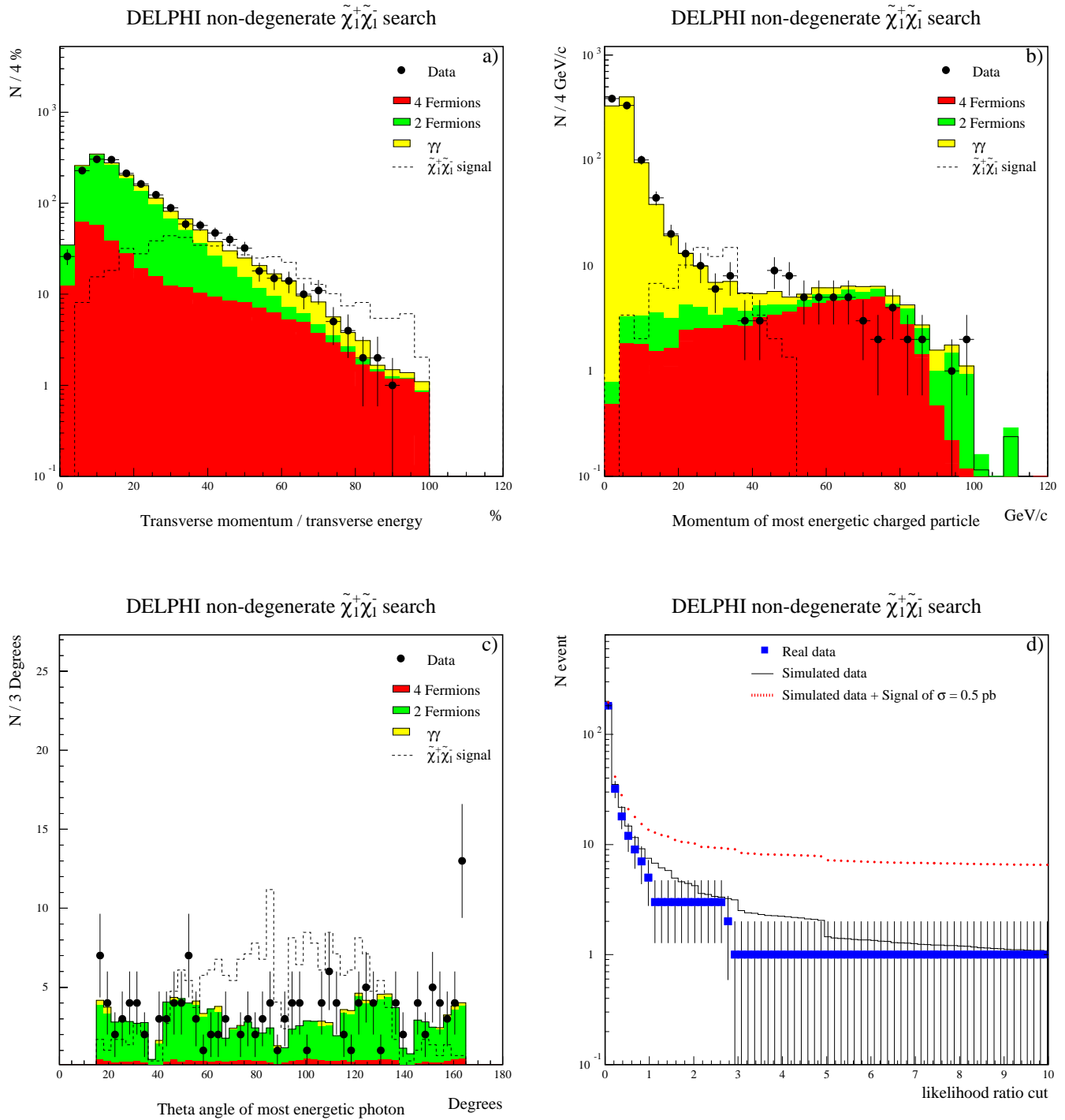
Figure 8: a), b) and c) show comparisons between real data (dots) and simulated background events (histogram) for the jets , ll and rad topologies respectively, using a logical OR of the 6 preselection cut functions of the corresponding topology. The dashed lines indicate how a characteristic chargino signal would appear (arbitrary normalisation). d) shows the number of events selected by the standard chargino analysis as a function of the \mathcal{L}_{\mathcal{R}_{CU\bar{T}}} cut in the jjll topology for 25 \leq \Delta M < 35 \text{ GeV}/c^2 . The squares are the data and the solid line is the background simulation. The dotted curve shows a possible signal, M_{\tilde{\chi}_1^\pm} = 102.8 \text{ GeV}/c^2 , M_{\tilde{\chi}_1^0} = 73 \text{ GeV}/c^2 , of 0.5 pb. In all cases the data collected in the year 2000 with the TPC sector 6 off are shown.
