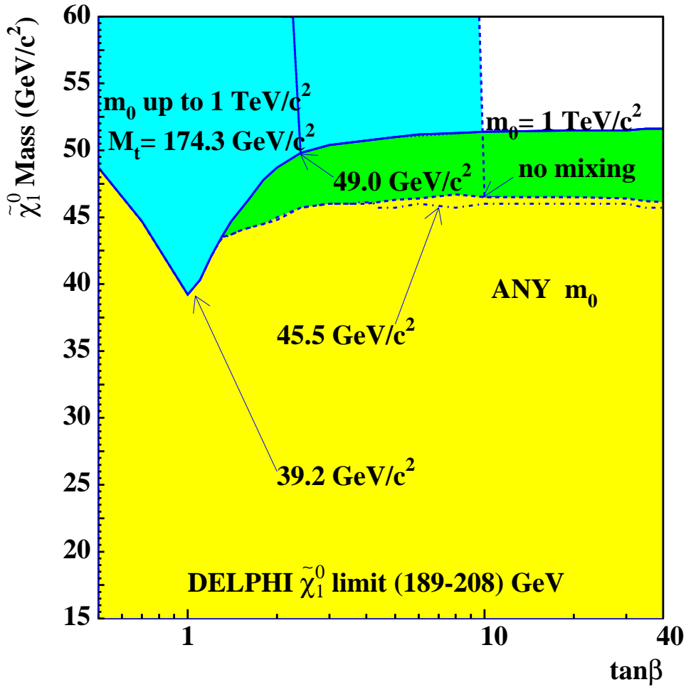
Figure 40: The lower limit on the mass of the lightest neutralino, \tilde{\chi}_1^0 , as a function of \tan\beta assuming a stable \tilde{\chi}_1^0 . The solid curve shows the limit obtained for m_0 = 1000 GeV/ c^2 , the dashed curve shows the limit obtained allowing for any m_0 assuming that there is no mixing in the third family ( A_\tau = \mu \tan\beta , A_b = \mu \tan\beta , A_t = \mu/\tan\beta ), and the dash-dotted curve shows the limit obtained for any m_0 allowing for mixing with A_\tau = A_b = A_t = 0 . The steep solid (dashed) line shows the effect of the searches for the Higgs boson for the maximal M_{h^0} scenario (no mixing scenario), m_0 \leq 1000 GeV/ c^2 and M_t = 174.3 GeV/ c^2 , which amounts to excluding the region of \tan\beta < 2.36(9.7) .
