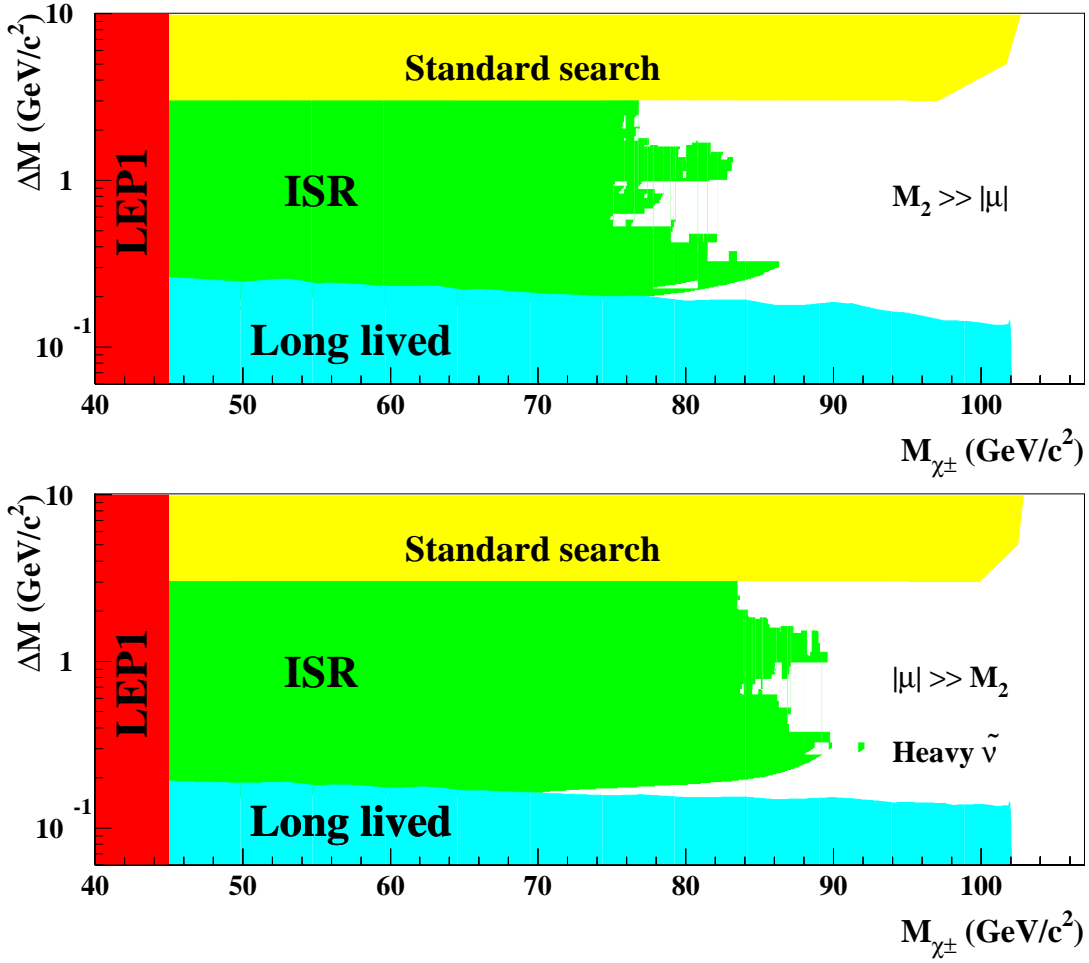
Figure 36: Regions in the plane (M_{\tilde{\chi}_1^\pm}, \Delta M) excluded using: the search for high \Delta M charginos; the search for soft particles accompanied by ISR; and the search for long-lived charginos. The two scenarios are (upper plot) the one in which the lightest chargino is a higgsino and (lower plot) the one in which the lightest chargino is a gaugino. For the second scenario, the limits are valid in the heavy sfermion approximation, while for the higgsino scenario it is sufficient that M_{\tilde{f}} > M_{\tilde{\chi}_1^\pm} .
