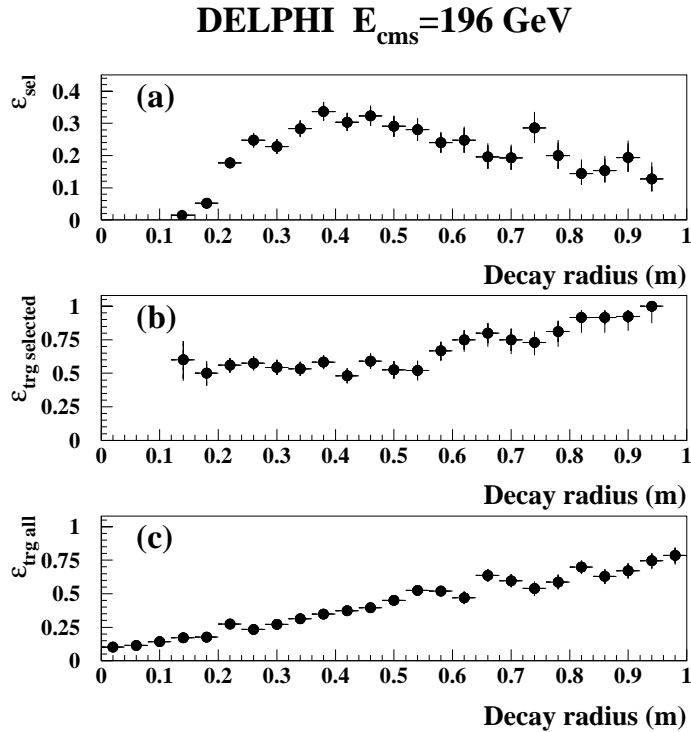
Figure 33: (a) Efficiency for selecting a single 75 \text{ GeV}/c^2 chargino in the search for displaced decay vertices (kinks) at the centre-of-mass energy of 196 GeV, as function of its decay radius. (b) Trigger efficiency for the selected charginos. (c) Trigger efficiency for all 75 \text{ GeV}/c^2 charginos, whether or not they were selected.
