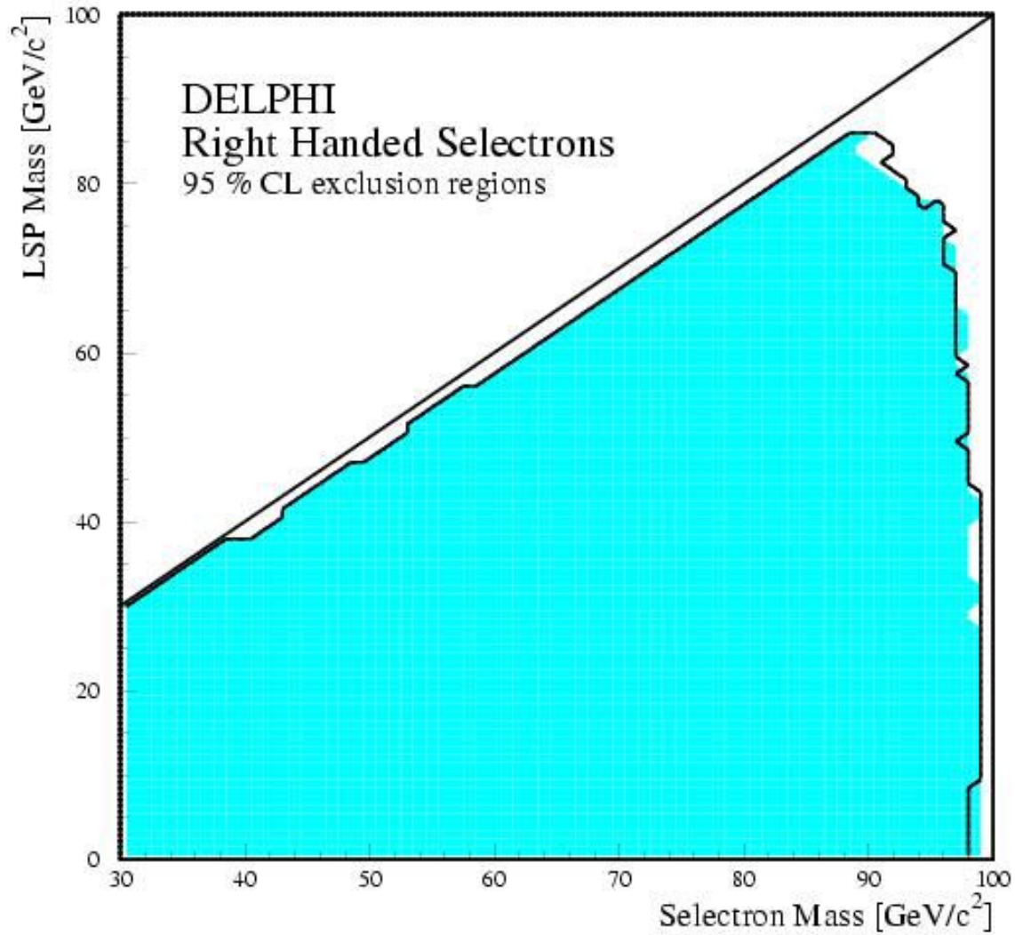
Figure 15: Excluded region in the (M_{\tilde{e}_R}, M_{LSP}) plane. The solid line shows the expected limit and the shaded region shows the obtained limit. The cross-section and the branching ratios for each mass point were determined with the SUSY parameters \tan \beta=1.5 and \mu=-200 \text{ GeV}/c^2 (for a discussion on the low selectron mass region see section 6.3).
