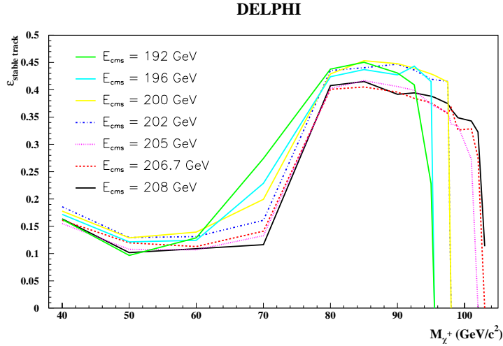
Figure 32: Efficiency for selecting a single almost stable chargino, as function of its mass, at the centre-of-mass energies of the years 1999 and 2000.
