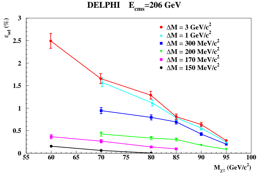
Figure 34: Selection times trigger efficiency in the search for nearly mass-degenerate charginos in the search with an ISR photon. The efficiency for higgsinos at \sqrt{s} = 206 \text{ GeV} at the different chargino masses and \Delta M values fully simulated is given as an example.
