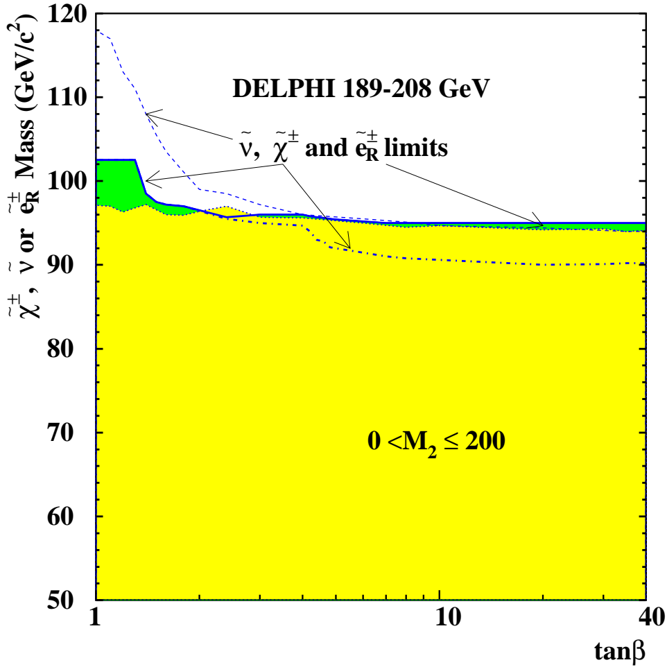
Figure 43: The minimum sneutrino mass (thin dashed curve) and the \tilde{e}_R mass (thin dotted curve and light shading) allowed by the slepton and neutralino searches, as a function of \tan\beta , together with the limits on the chargino mass (thick solid curve and dark shading, and thick dash-dotted curve). The chargino mass limit indicated by the solid curve and the sneutrino and selectron mass limits were obtained assuming no mass splitting in the third sfermion family ( A_\tau - \mu \tan\beta = 0 in particular). The selectron mass limit is valid for M_{\tilde{e}_R} - M_{\tilde{\chi}_1^0} > 10 \text{ GeV}/c^2 . The chargino mass limit indicated with the dash-dotted curve was obtained allowing for mass splitting in the third sfermion family, with A_\tau = A_b = A_t = 0 .
