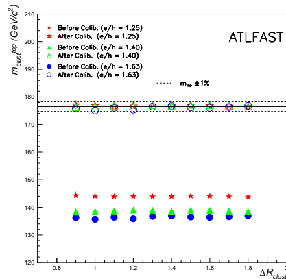
Fig. 32. Reconstructed m_{clust}^{top} mass values before and after the rescaling from the W reconstruction in the inclusive sample for three values of e/h .
