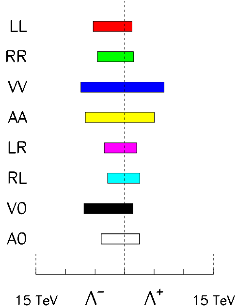
Figure 8: The 95% CL limits on the scale of Contact Interactions in e^+e^- \rightarrow b\bar{b} and e^+e^- \rightarrow c\bar{c} using Heavy Flavour LEP combined results from 133 to 207 GeV.
