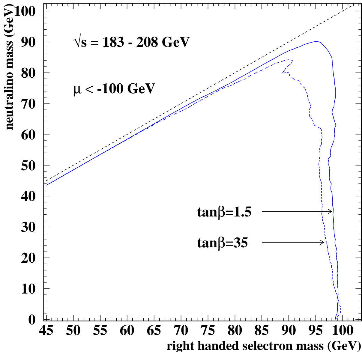
Figure 13: For two values of \tan\beta and \mu < -100 GeV, 95% CL exclusion regions for right-handed selectron pairs within the MSSM, obtained by combining the \sqrt{s} = 183 - 208 GeV data-sets. The excluded regions are calculated taking into account the predicted branching ratio for \tilde{e}_R^\pm \rightarrow e^\pm \tilde{\chi}_1^0 . The gauge unification relation, M_1 = \frac{5}{3} \tan^2 \theta_W M_2 , is assumed in calculating the MSSM cross-sections and branching ratios. The kinematically allowed region lies below the dashed line.
