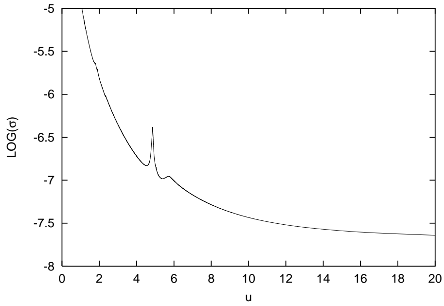
Figure 8. The opacity cross-section, \sigma , (in atomic units) for the 6-element mix at \log(T) = 7.2 , \log(N_e) = 26 , \log(R) = -1.306 .
