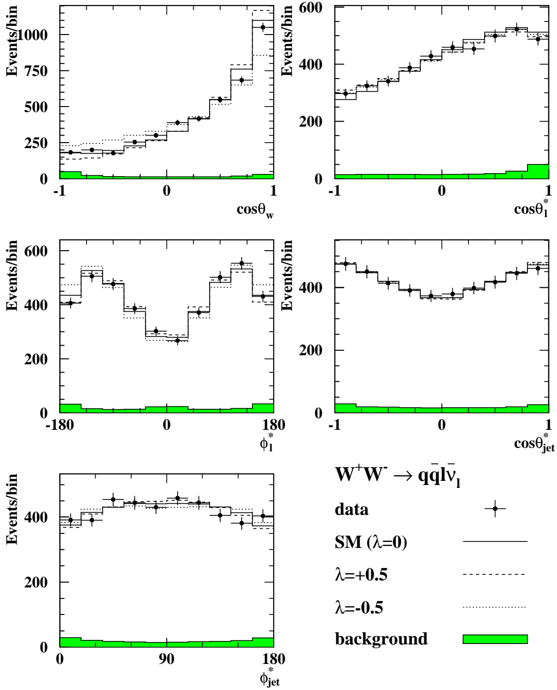
Figure 1: Distributions of the kinematic variables \cos\theta_w , \cos\theta_\ell^* , \phi_\ell^* , \cos\theta_{\text{jet}}^* and \phi_{\text{jet}}^* , obtained from the q\bar{q}l\bar{\nu}_\ell candidates. The solid points represent the data. The histograms show the Monte Carlo expectation of the Standard Model (solid line) and the cases of \lambda = +0.5 and \lambda = -0.5 (dashed and dotted lines respectively). The Monte Carlo histograms are normalised to the number of data events. The shaded histograms show the non- q\bar{q}l\bar{\nu}_\ell background. In the case of W^+ \rightarrow \bar{\ell}\nu decays the value of \phi_\ell^* is shifted by 180^\circ in order to overlay W^+ and W^- distributions in the same plot, which is valid so long as CP is conserved.
