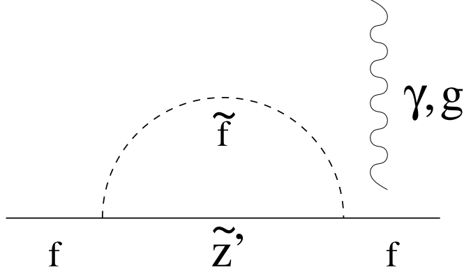
Figure 1: The \tilde{Z}' -sfermion diagram which contributes to the (chromo-)electric and (chromo-)magnetic dipole moments of the fermion f . The photon ( \gamma ) or gluon ( g ) are to be attached in all possible ways.
