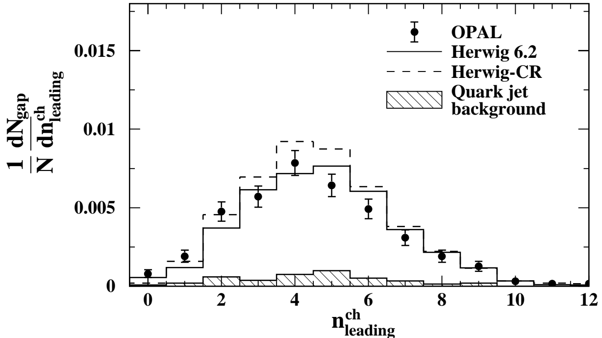
Figure 11: Distribution of n_{\text{leading}}^{\text{ch}} in the leading part of gluon jets, based on the y_{\text{min}} selection (see Sect. 6). “N” represents the total number of selected gluon jets and “ N_{\text{gap}} ” the number of gluon jets with a rapidity gap. The distributions include the effects of initial-state photon radiation and detector acceptance and resolution. The results are shown in comparison to the predictions of the Herwig and Herwig-CR models. The uncertainties are statistical only. The hatched area shows the quark jet background evaluated using Herwig.
