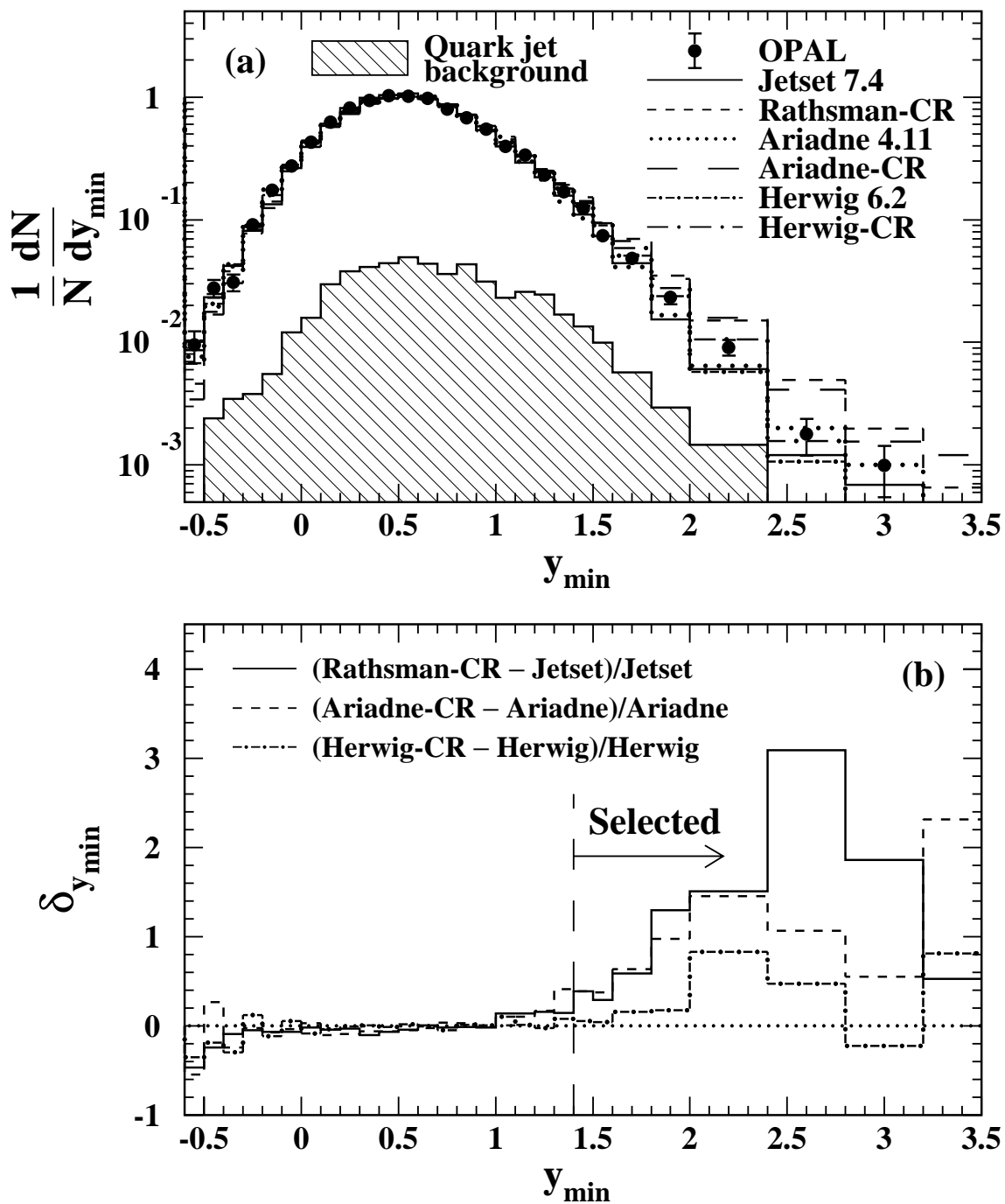
Figure 8: (a) Distribution of y_{\min} in the tagged gluon jets. The distribution includes the effects of initial-state photon radiation and detector acceptance and resolution. The uncertainties are statistical only. The results are shown in comparison to the predictions of QCD Monte Carlo programs which include detector simulation and the same analysis procedures as are applied to the data. The hatched area shows the quark jet background evaluated using Jetset. (b) Fractional difference between the results of a Monte Carlo program with color reconnection and the corresponding model without reconnection. To define gluon jets with a rapidity gap, the region y_{\min} \geq 1.4 , to the right of the vertical dashed line, is selected.
