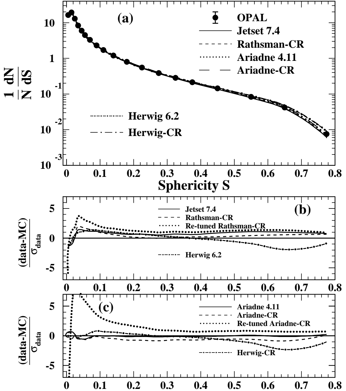
Figure 2: (a) The Sphericity distribution for inclusive Z^0 events, in comparison to the predictions of models with and without color reconnection (CR). The data have been corrected for initial-state photon radiation and detector response. The statistical uncertainties are too small to be visible. The vertical lines attached to the data points (barely visible) show the total uncertainties, with statistical and systematic terms added in quadrature. (b) and (c) show the deviations of the Monte Carlo predictions from the data in units of the total experimental uncertainties, \sigma_{\text{data}} .
