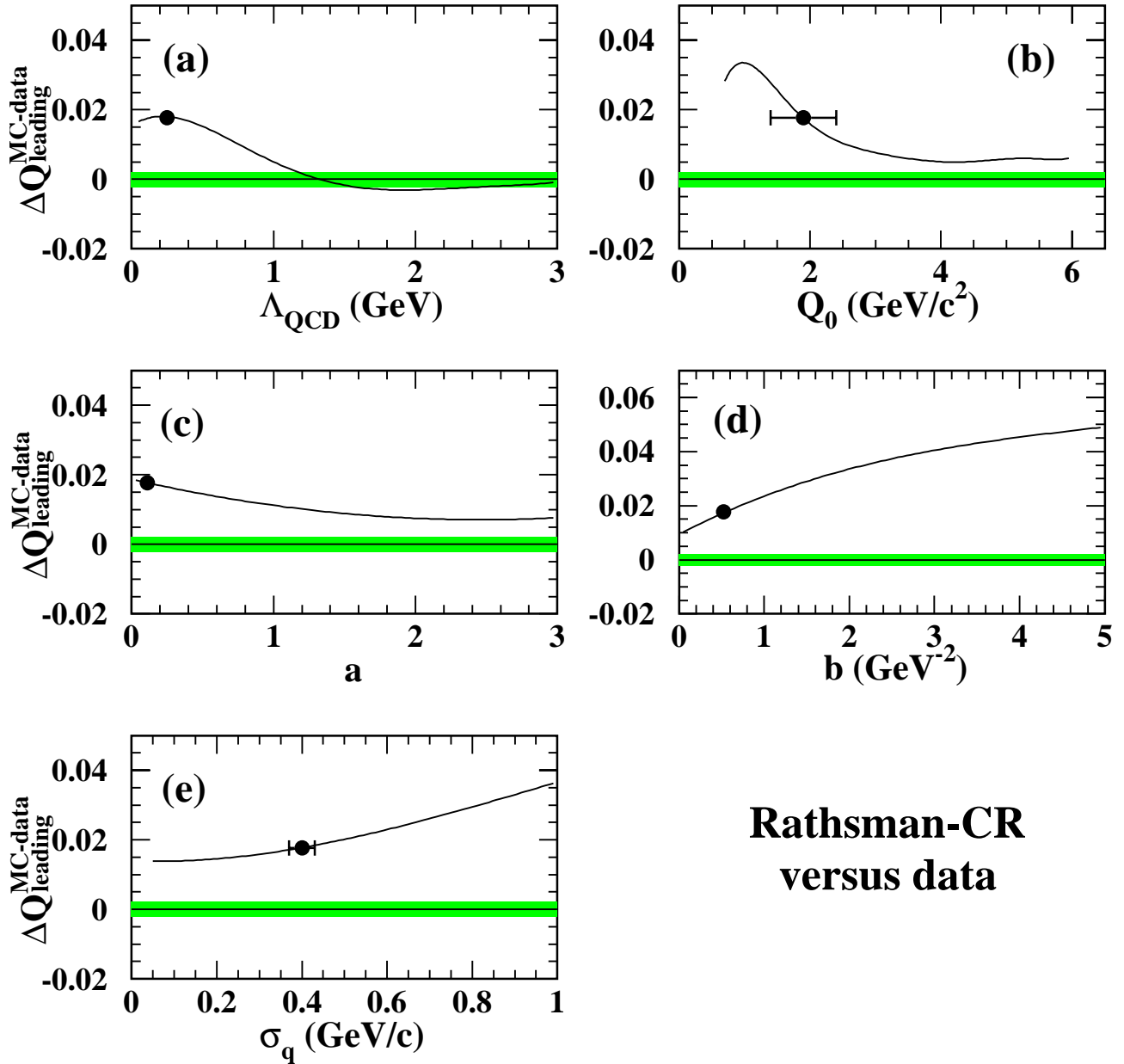
Figure 15: Results for the difference between the Rathsman-CR Monte Carlo prediction and the experimental result for the Q_{\text{leading}} = 0 bin in Fig. 13b, \Delta Q_{\text{leading}}^{\text{MC-data}} , as the principal parameters of the model are changed with the other parameters at their default settings. The solid dots indicate the standard values of the parameters. The horizontal error ranges show the uncertainties attributed to the parameter values in [23]. For the parameters \Lambda_{\text{QCD}} and b , these uncertainties are too small to be visible. Note an uncertainty is not evaluated for the a parameter. The width of the shaded band centered on \Delta Q_{\text{leading}}^{\text{MC-data}} = 0 equals twice the total experimental uncertainty of \Delta Q_{\text{leading}}^{\text{MC-data}} .
