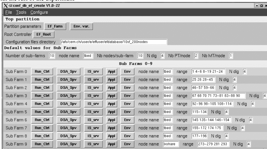
Figure 1: Graphical User Interface for database entry program
