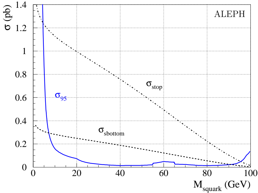
Figure 9: The production cross sections for e^+e^- \rightarrow \tilde{t}\tilde{t} and \tilde{b}\tilde{b} at \sqrt{s} = 209 GeV, as a function of the squark mass. Also shown is the observed 95% C.L. upper limit on the cross section, derived from the stable stop search of Ref. [3].
