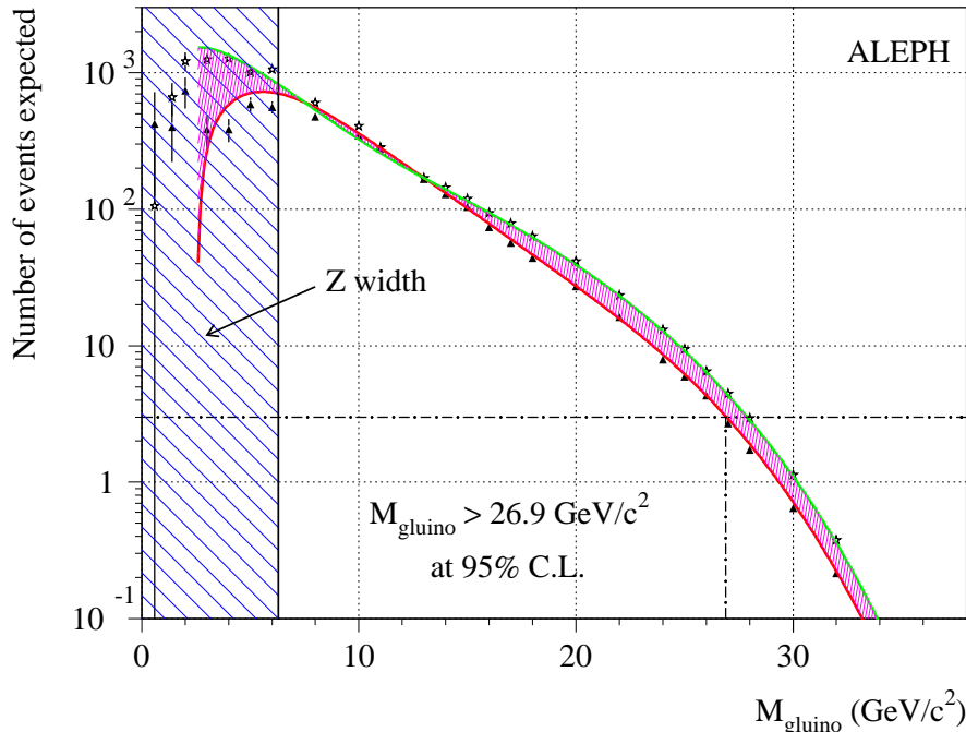
Figure 6: The number of q\bar{q}\tilde{g}\tilde{g} events expected to be selected in the LEP1 data by the neutral and charged R-hadron searches, as a function of the gluino mass, for P_{\tilde{g}\tilde{g}} varying between 0 and 1 (shaded area). The markers with error bars (triangles for P_{\tilde{g}\tilde{g}} = 1 , stars for P_{\tilde{g}\tilde{g}} = 0 ) show the individual values obtained from each of the simulated signal samples. Also shown is the region excluded by the Z lineshape measurement (hatched region), and the lower limit on the gluino-LSP mass (dot-dashed lines).
