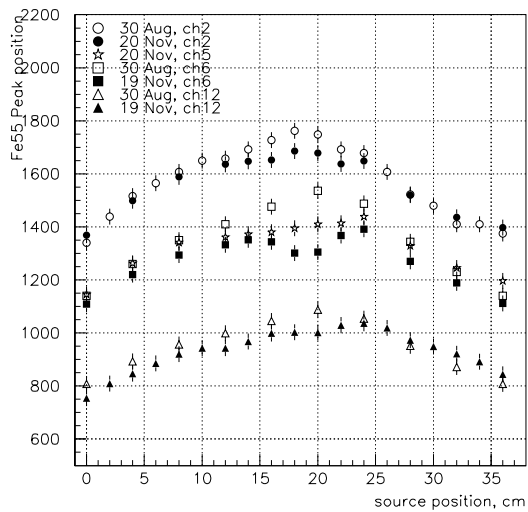
Fig. 6. Peak position of the 55 Fe spectrum along the wire for several irradiated wires after an accumulated charge of 600 mC/cm in chambers operated with Ar/CF 4 /CO 2 (65:30:5) (full symbols), compared with the situation before irradiation (open symbols). The gain drop is between 6-10 % in the center of the irradiation zone due to the swelling of the anode wires.
