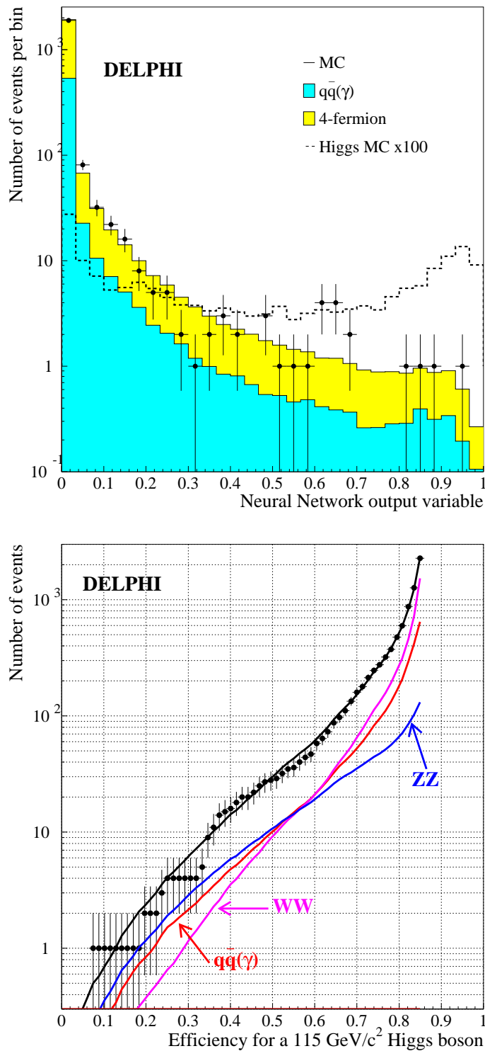
Figure 17: Hq\bar{q} channel: Top: the distribution of the neural network variable used to select Higgs candidates in the 2000 data. The signal expectation is shown for a 115 \text{ GeV}/c^2 Higgs, normalised to 100 times the expected rate. The dots represent the data. Bottom: curve of the expected SM background rate in the 2000 data as a function of the efficiency for a 115 \text{ GeV}/c^2 Higgs signal when varying the cut on the neural network variable. The different background contributions are shown separately. The dots represent the data.
