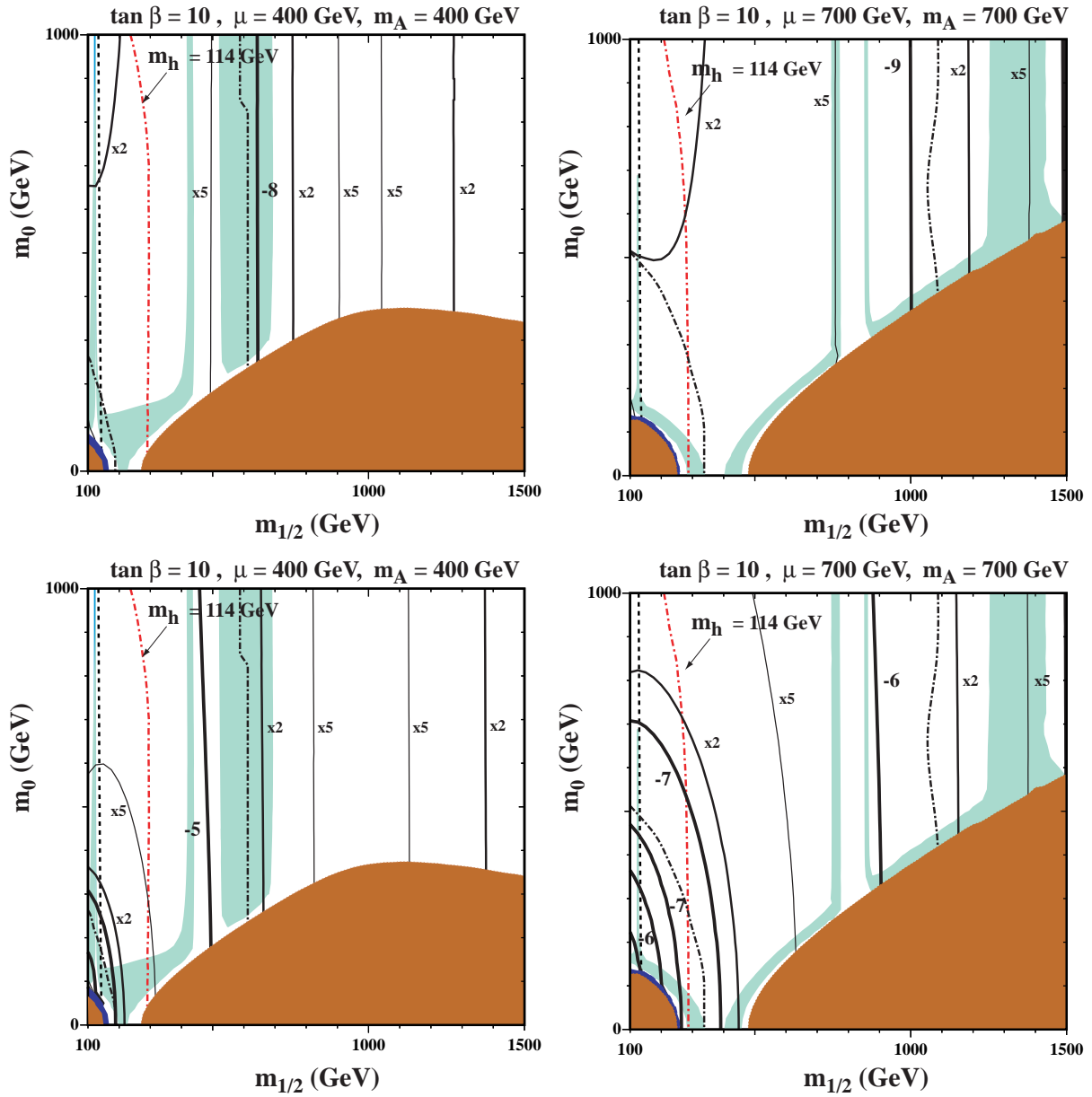
Figure 1: Contours of (a,b) the spin-independent and (c,d) the spin-dependent cross sections (solid black lines) are superimposed on the NUHM (m_{1/2}, m_0) planes for \tan\beta = 10 and (a,c) \mu = 400 GeV and m_A = 400 GeV, and (b,d) \mu = 700 GeV and m_A = 700 GeV. The near-vertical (red) dot-dashed lines are the contours m_h = 114 GeV, and the near-vertical (black) dashed lines at lower m_{1/2} are the contours m_{\chi^\pm} = 103.5 GeV. The dark (brick red) shaded regions is excluded because a charged particle is lighter than the neutralino, and the darker (dark blue) shaded regions is excluded because the LSP is a sneutrino. The light (turquoise) shaded areas are the cosmologically preferred regions with 0.1 \leq \Omega_\chi h^2 \leq 0.3 . The dark (black) dot-dashed lines indicate the GUT stability constraint. There are two such lines for each panel and only the areas in between are allowed by this constraint.
