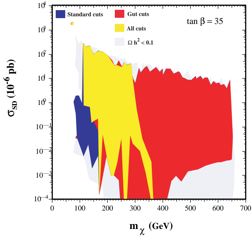
Figure 9: Ranges of (a) the spin-independent and (b) the spin-dependent cross sections for \tan \beta = 35 . The shadings are the same as in Fig. 7.
