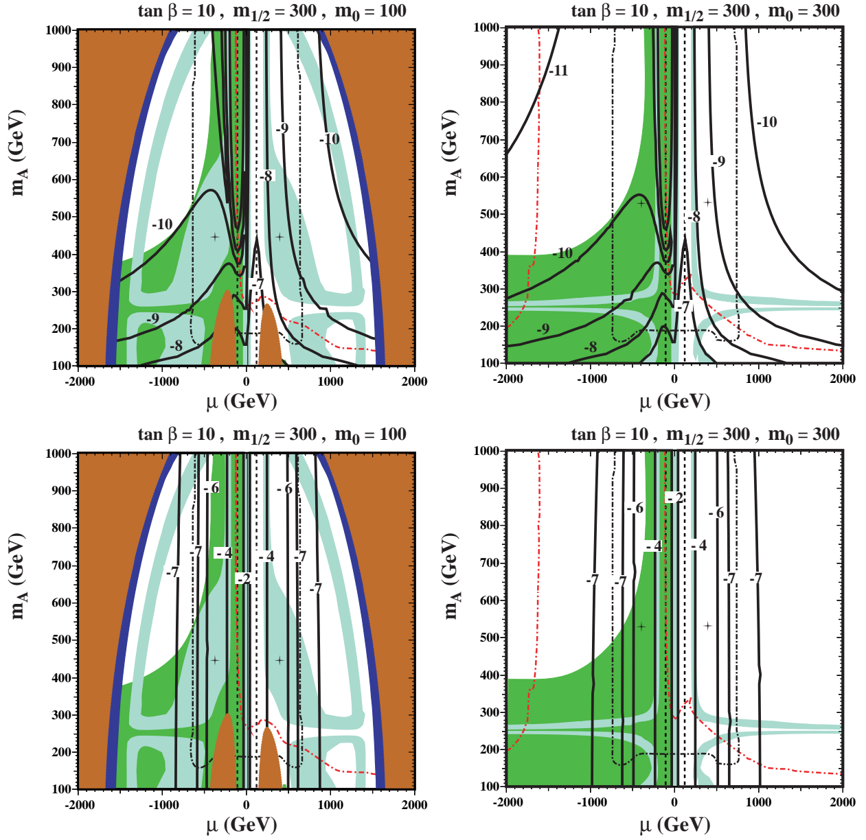
Figure 2: Contours of (a,b) the spin-independent and (c,d) the spin-dependent cross sections (solid black lines) are superimposed on the NUHM ( \mu, m_A ) planes for \tan\beta = 10 , (a,c) m_0 = 100 GeV and m_{1/2} = 300 GeV, (b,d) m_0 = 300 GeV and m_{1/2} = 300 GeV. The shadings and line styles are the same as in Fig. 1. Here, we see in addition the constraint from b \rightarrow s\gamma . The excluded region is medium (green) shaded. The crosses denote the CMSSM points for these choices of m_0 and m_{1/2} .
