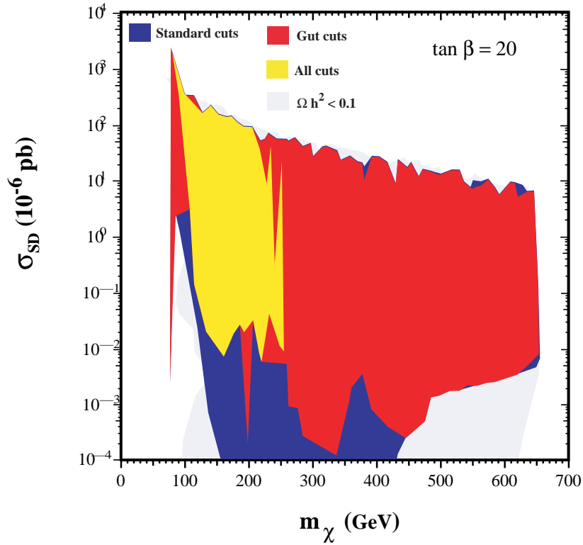
Figure 8: Ranges of (a) the spin-independent and (b) the spin-dependent cross sections for \tan \beta = 20 . The shadings are the same as in Fig. 7.
