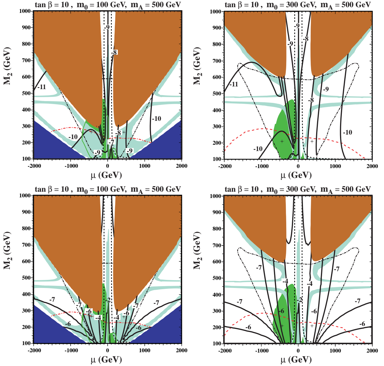
Figure 3: Contours (a,b) of the spin-independent and (c,d) spin-dependent cross sections (solid black lines) are superimposed on the NUHM (\mu, M_2) planes for \tan \beta = 10 , (a,c) m_0 = 100 GeV and m_A = 500 GeV, (b,d) m_0 = 300 GeV and m_A = 500 GeV. The shadings and line styles are the same as in Fig. 2, and the crosses denote the CMSSM points for these choices of m_0 and m_A .
