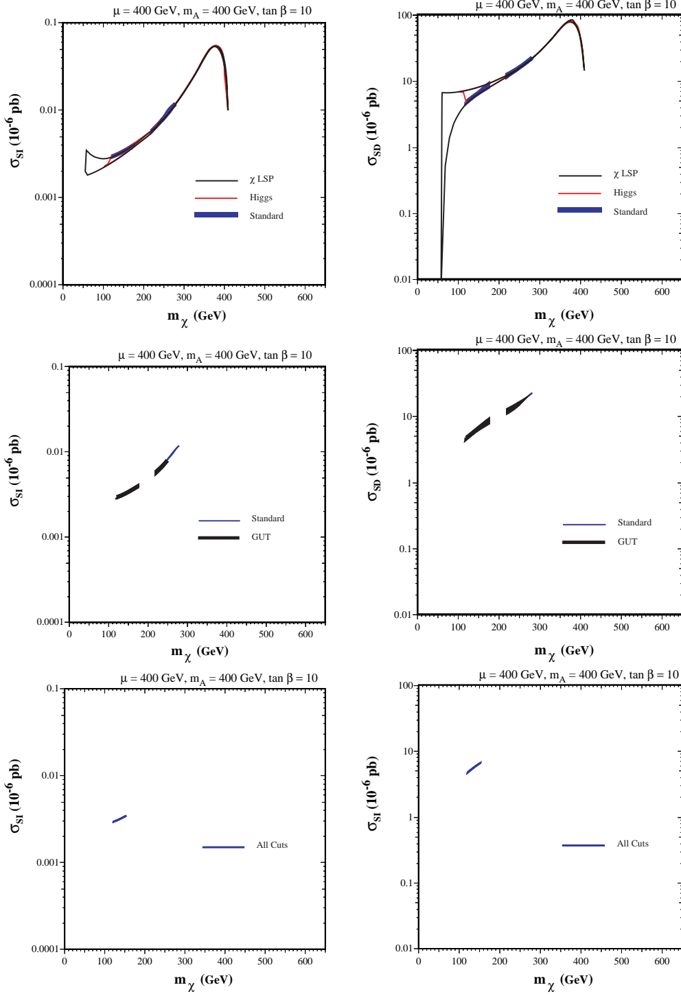
Figure 4: Cross sections allowed in a slice through the NUHM parameter space provided by the (m_{1/2}, m_0) plane for \tan \beta = 10 and \mu = m_A = 400 GeV. Panels (a,b) are with our cuts on the LSP (dark lines), m_h (lighter lines) and standard cut (shaded), panels (c,d) also have the GUT stability constraint imposed, and panels (e,f) apply all cuts, including the possible g_\mu - 2 constraint. The right (left) panels show the spin-(in)dependent cross section, plotted against m_\chi .
