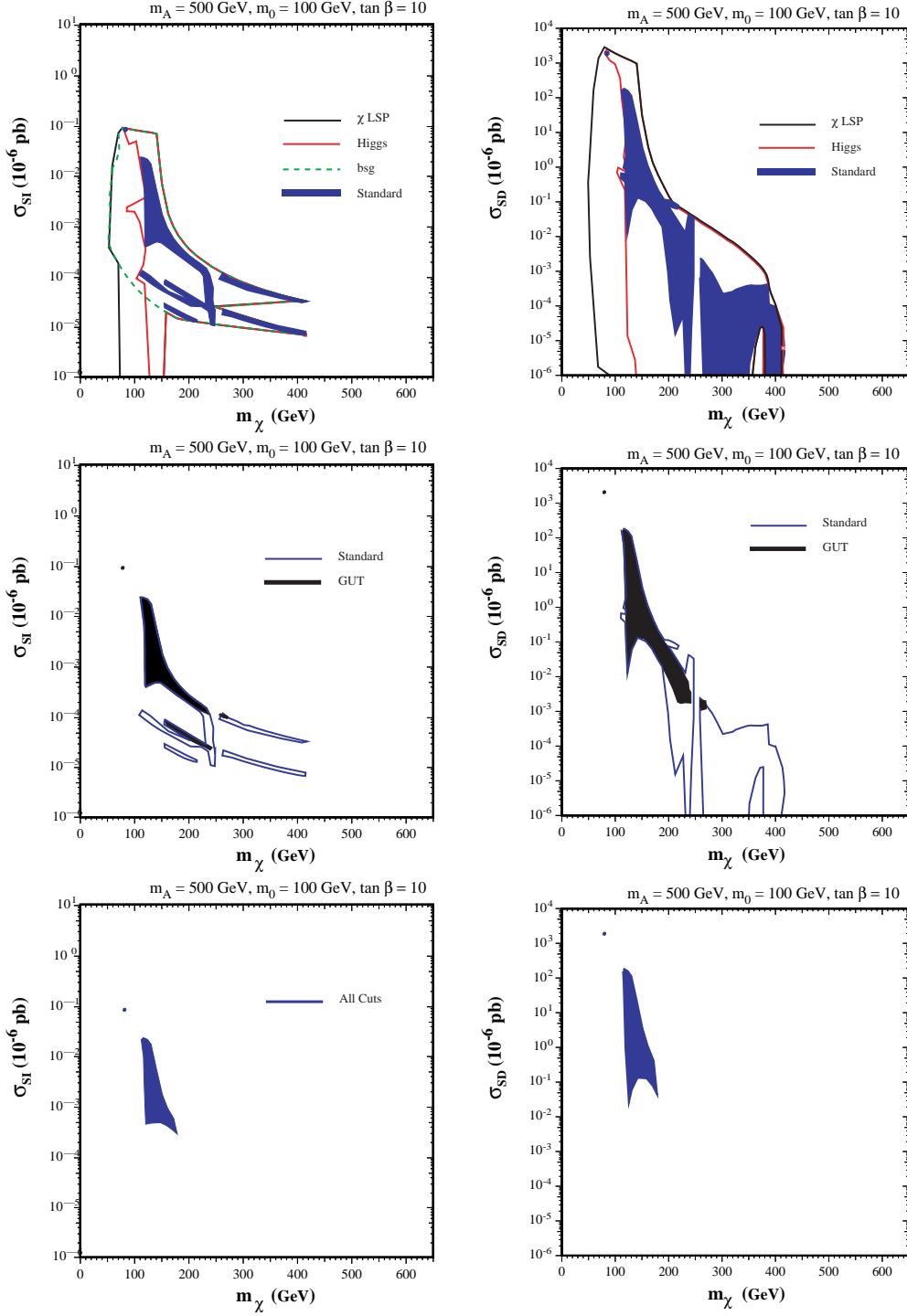
Figure 6: Cross sections allowed in a slice through the NUHM parameter space provided by the (\mu, M_2) plane for \tan\beta = 10 and m_0 = 100 GeV, m_A = 500 GeV. The selections of points in the different panels are the same as in Fig. 5, as are their indications.
