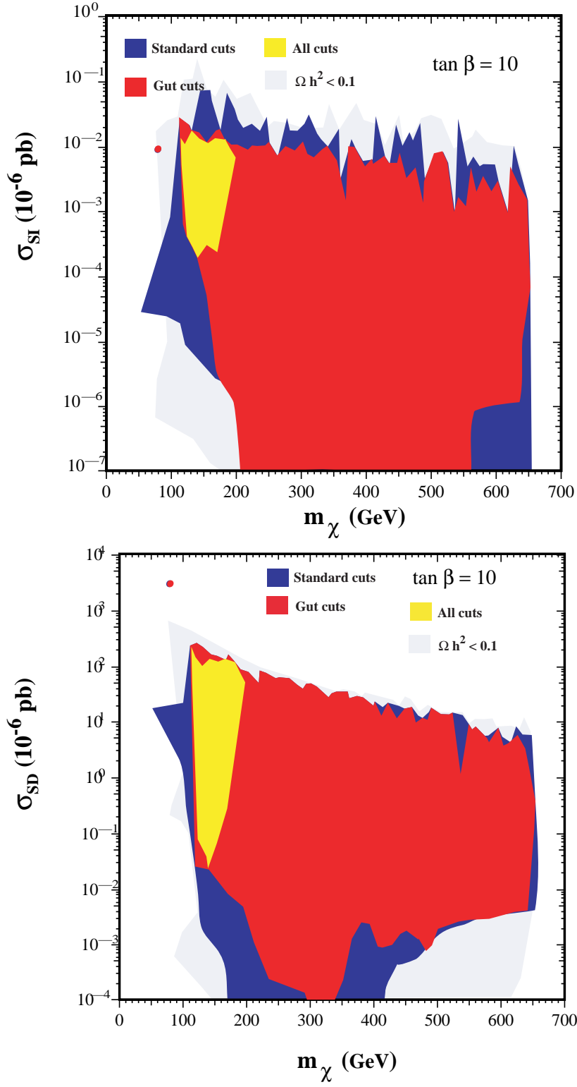
Figure 7: Ranges of (a) the spin-independent and (b) the spin-dependent cross sections for \tan \beta = 10 . The ranges allowed by the standard cuts on \Omega_\chi h^2 , m_h and b \rightarrow s\gamma have dark shading, those still allowed by the GUT stability cut have medium shading, and those still allowed after applying all the cuts including g_\mu - 2 have light shading. The pale shaded region corresponds to the extra area of points with low relic densities, whose cross sections have been rescaled appropriately.
