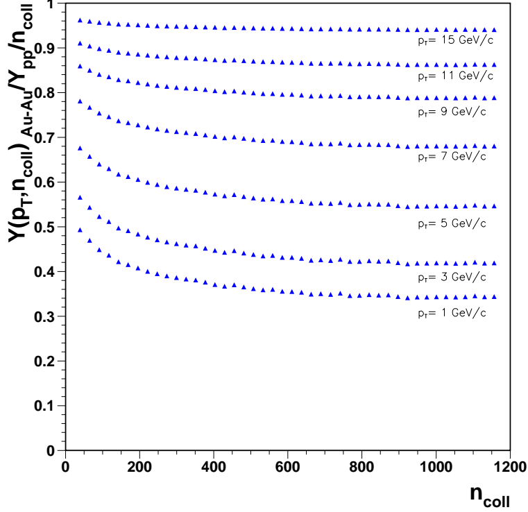
Figure 3: The ratio Y_{\text{Au+Au}}(p_T, b)/[n_{\text{coll}}(b) Y_{pp}(p_T)] plotted as a function of n_{\text{coll}}(b) for p_T = 1 \text{ GeV}/c , p_T = 3 \text{ GeV}/c , p_T = 5 \text{ GeV}/c , p_T = 7 \text{ GeV}/c and p_T = 9 \text{ GeV}/c in Au+Au interactions at RHIC. Parameters are given in the text, \sigma_0 = 8 \text{ mb} .
