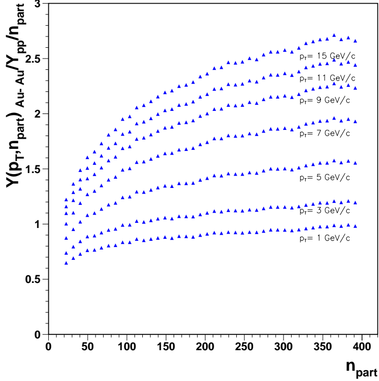
Figure 2: The ratio Y_{\text{Au+Au}}(p_T, b) / [n_{\text{part}}(b) Y_{pp}(p_T)] plotted as a function of n_{\text{part}}(b) for p_T = 1 \text{ GeV}/c , p_T = 3 \text{ GeV}/c , p_T = 5 \text{ GeV}/c , p_T = 7 \text{ GeV}/c and p_T = 9 \text{ GeV}/c in Au+Au interactions at RHIC. Parameters are given in the text, \sigma_0 = 8 \text{ mb} .
