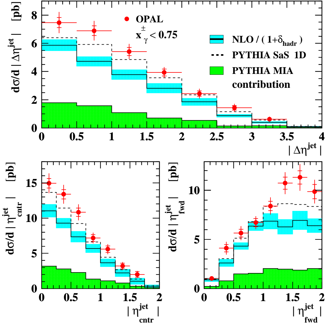
Figure 16: The di-jet cross-section as a function of |\Delta\eta^{\text{jet}}| for the two leading jets in E_T^{\text{jet}} and separately for the central and the forward jet. For these cross-sections x_{\gamma}^{\pm} < 0.75 is required. The total of statistical and systematic uncertainties added in quadrature is shown where larger than the marker size. The inner error bars show the statistical errors. The numerical values are given in Tables 7, 8 and 9. The NLO calculation and MC simulation are the same as in Figure 11.
