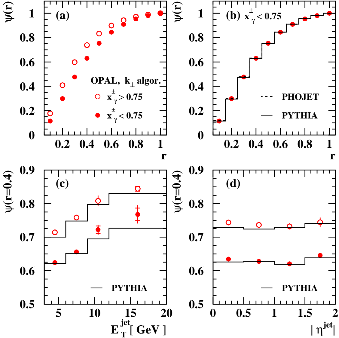
Figure 7: The jet shape, \Psi(r) , for the two regions of x_{\gamma}^{+}-x_{\gamma}^{-} -space indicated in the figure (a), and \Psi(r) for x_{\gamma}^{\pm} < 0.75 compared to the predictions of the LO MC generators PHOJET and PYTHIA (b). Figures (c) and (d) show the value of \Psi(r = 0.4) as a function of the transverse energy and pseudo-rapidity of the jet respectively, compared to the PYTHIA prediction. The total of statistical and systematic uncertainties added in quadrature is shown where larger than the marker size. The inner error bars show the statistical errors.
