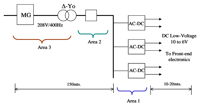
Figure 1: Distribution system scheme for HCAL/EMU sub-detectors
