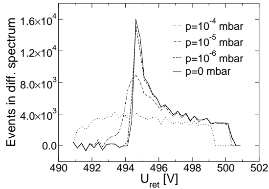
Figure 7: Effect of the residual gas on the shape of the response function (for 1 \cdot 10^7 events, E = 500 \text{ eV} , \sigma = 1.2\% ). The calculation was performed for Argon buffer gas. For Helium buffer gas the indicated pressures have to be multiplied by a factor of \approx 0.1 . In order to get a response function with a well-defined peak the residual gas pressure in the cooler trap needs to be \leq 10^{-6} \text{ mbar} or better.
