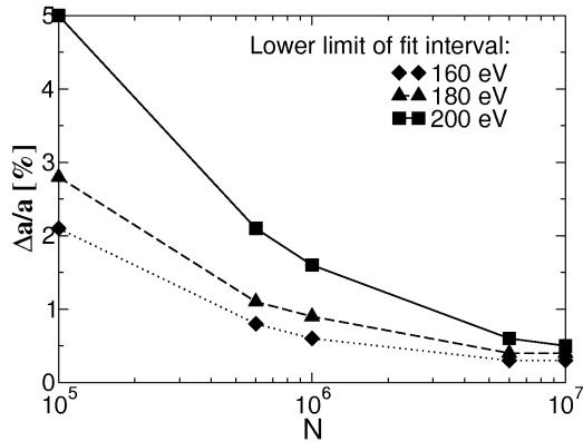
Figure 8: Precision achievable on the \beta - \nu angular correlation coefficient a ( CL = 68.3\% ). This is the result of a simulation for ^{26}\text{Al}^m(E_0 = 280 \text{ eV}) . Three curves are shown for different analysis intervals. The x-axis displays the number of events N in the total differential recoil energy spectrum. Typically, to get one differential event \approx 10^4 ions have to be trapped.
