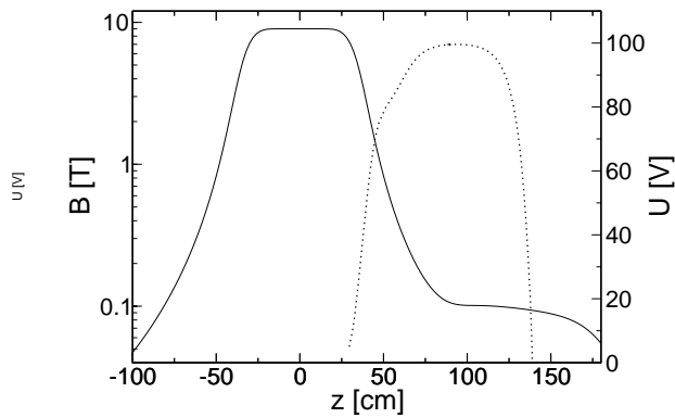
Figure 4: Magnetic (solid line) and electric (dashed line) fields on the axis of the retardation spectrometer. The two Penning traps are in the region with B = 9\text{ T} . The electric field has been calculated for U_{ret} = 100\text{ V} . The trap potential is not shown.
