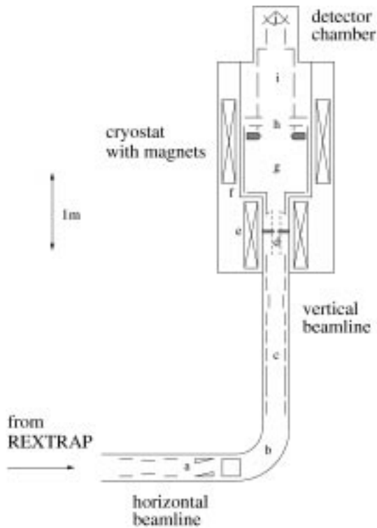
Figure 2: The experimental set-up consists of several parts: A horizontal beamline (a), which is connected via a spherical 90^\circ bender (b) to a vertical beamline (c). Both beamlines contain electrostatic ion optics, e.g. steerers and an Einzel lens in the horizontal beamline and retardation electrodes as well as a pulsed drift tube in the vertical beamline. Two Penning traps (d) are located in the bore of a 9\text{ T} magnet (e). The retardation spectrometer is formed by this magnet, a 0.1\text{ T} magnet (f) and retardation electrodes (g). Finally, the set-up contains an electrostatic acceleration section (h), a large Einzel lens (i) and an ion detector (j). For details of the Penning traps and the retardation spectrometer see Figs. 3 and 5. This figure is only approximately to scale.
