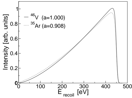
Figure 1: Calculated differential recoil energy spectra for a = 1 ( ^{46}\text{V} ) and a = 0.908 ( ^{35}\text{Ar} ). The energy axis of the spectrum of ^{46}\text{V} has been scaled in order to have the same endpoint energies for both spectra. The experiment discussed in this article intends to distinguish between a = 1 and a = 0.995 .
