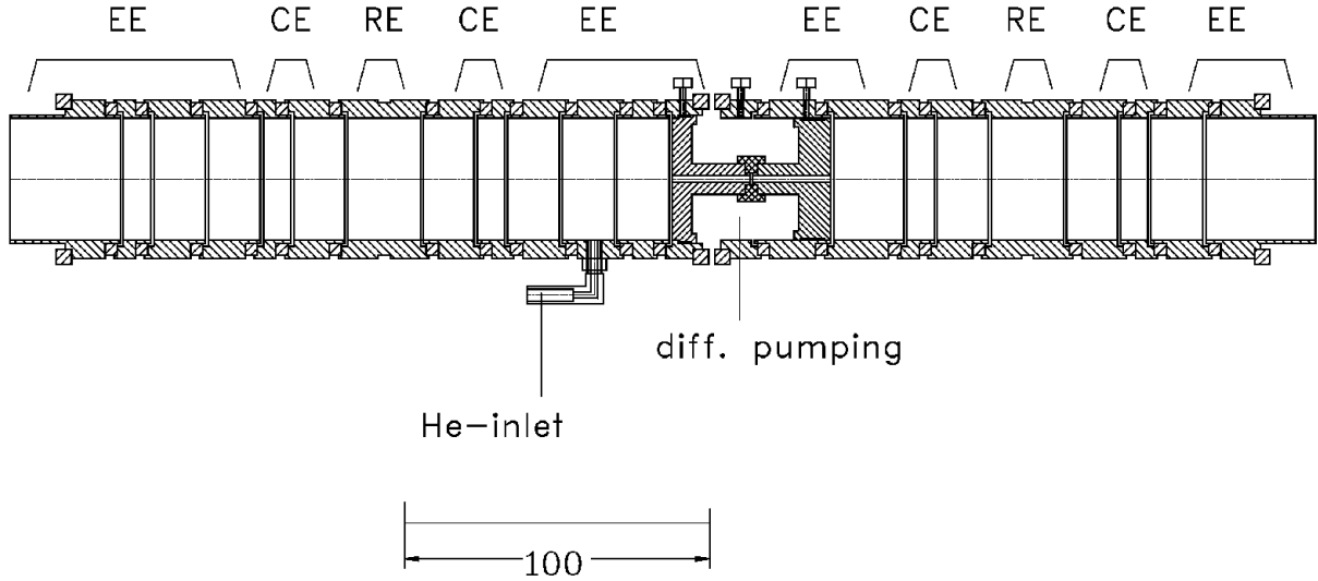
Figure 3: Geometry of the Penning traps. The cooler trap (left) is separated from the decay trap (right) by a differential pumping barrier. The inner diameter of the trap electrodes is 4\text{ cm} . The distance between the trap centers is 21.1\text{ cm} and the total length of the two traps 42.8\text{ cm} . EE denotes the end-cap electrodes, CE the correction electrodes and RE the central ring electrode of the traps. The buffer gas inlet is also indicated.
