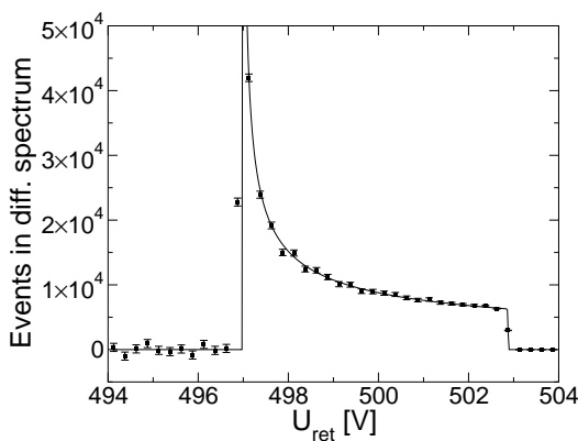
Figure 6: Theoretical (solid line) and simulated (symbols, 6 \cdot 10^5 events, E = 503 \text{ eV} , \sigma = 1.2\% , see text) response functions. This is the lineshape in the differential recoil energy spectrum. At E \cdot (1 - \sigma) is a pole in the theoretical response function. The good agreement between the theoretical and simulated lineshape indicates that the ion motion will be sufficiently adiabatic for the field configurations used in the experiment.
