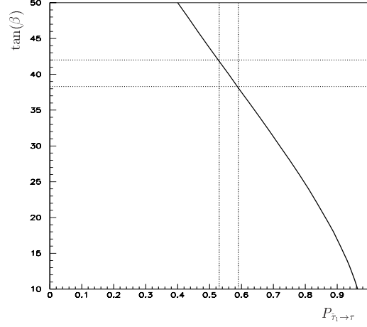
Figure 6. Determination of \tan\beta from the tau polarization P_{\tilde{\tau}_1 \rightarrow \tau} in the decay \tilde{\tau}_1^- \rightarrow \tau^- \tilde{\chi}_1^0 .
