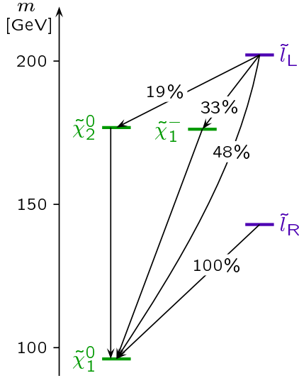
Figure 1. Masses and branching ratios of sleptons of the first two generations in the SPS1 scenario [3]. The total widths are \Gamma_{\tilde{l}_R} = 210 MeV and \Gamma_{\tilde{l}_L} = 250 MeV.
