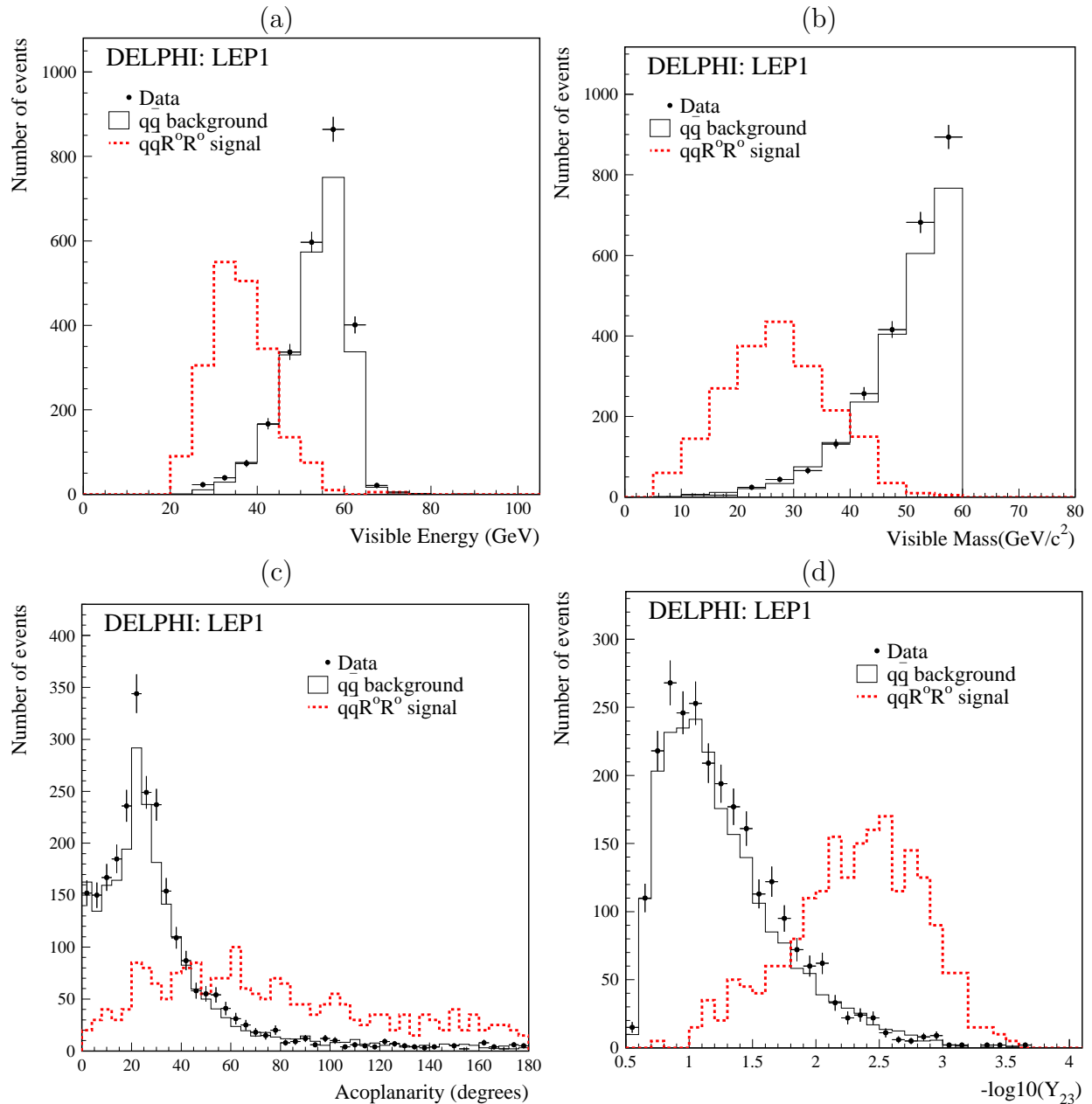
Figure 8: Comparison between data and simulation in the q\bar{q}R^oR^o analysis at LEP1. (a) visible energy, (b) visible mass, (c) acoplanarity (d) DURHAM distance Y_{23} . Dotted lines show the q\bar{q}R^oR^o signal distributions with arbitrary normalization when all simulated samples are added together.
