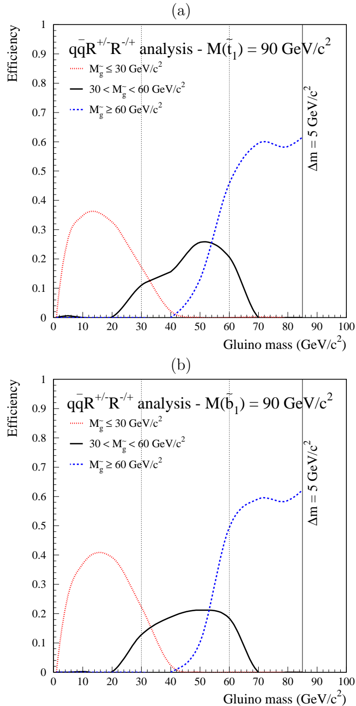
Figure 10: Signal detection efficiencies at \sqrt{s} = 200 \text{ GeV} for the stop (a) and sbottom (b) qqR^{\pm}R^{\pm} analysis as a function of the gluino mass ( m_{\tilde{q}_1} = 90 \text{ GeV}/c^2 ). \Delta M is the mass difference between the squark and the gluino. Vertical lines show the limits of the mass analysis window. The last one ends at \Delta M = 5 \text{ GeV}/c^2 which corresponds the last simulated signal points.
