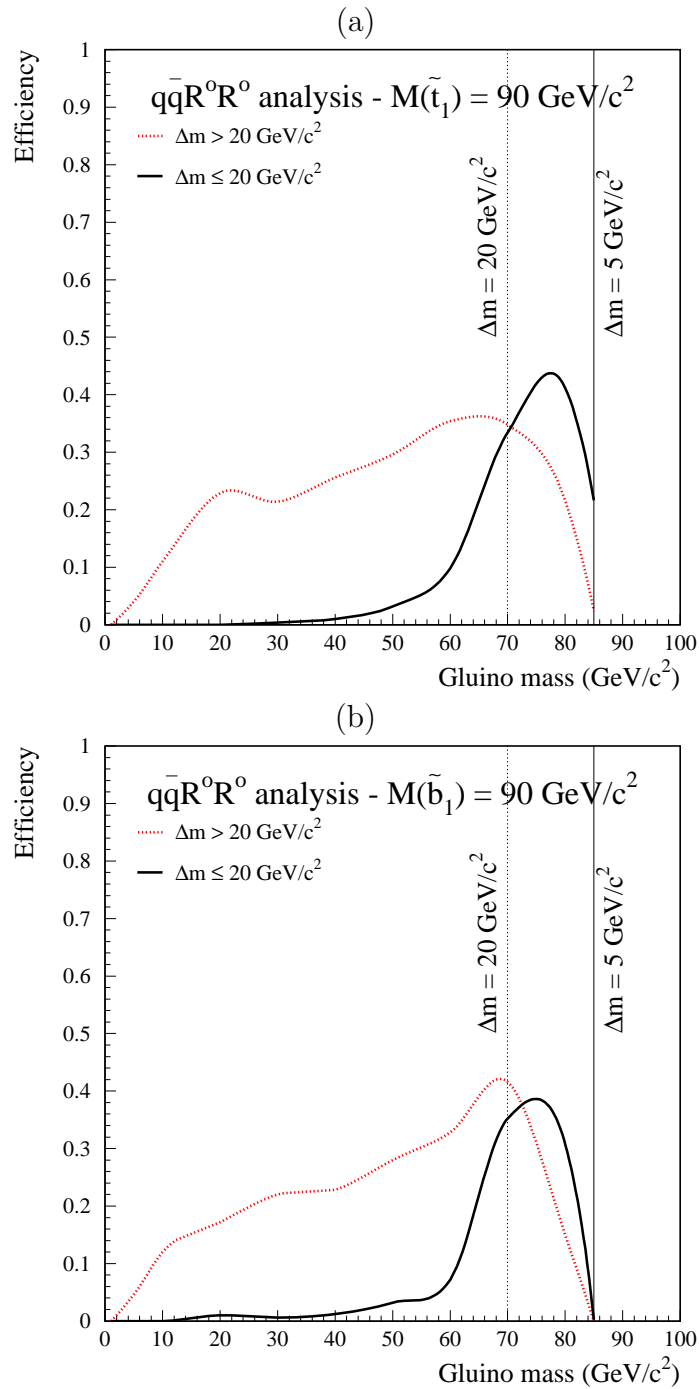
Figure 16: Signal detection efficiencies at \sqrt{s} = 200 \text{ GeV} for the stop (a) and sbottom (b) qq\bar{R}^0R^0 analysis as a function of the gluino mass ( m_{\tilde{q}_1} = 90 \text{ GeV}/c^2 ).
