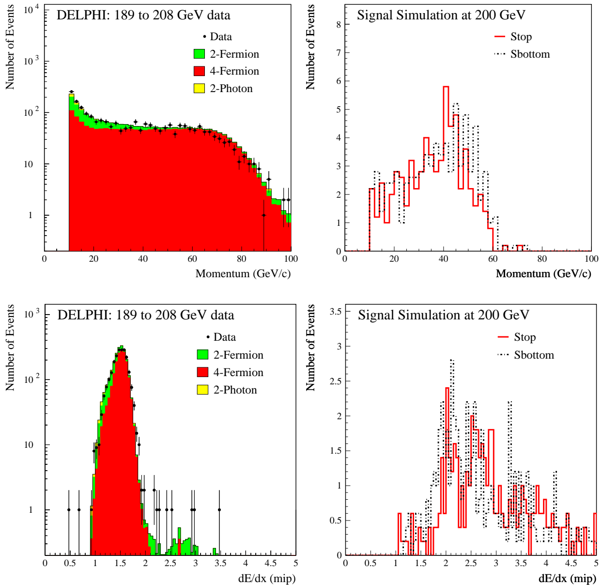
Figure 11: Momentum and dE/dx of the charged R-hadron candidates selected by the q\bar{q}R^{\pm}R^{\circ} analysis at LEP2. Data taken in the centre-of-mass energy range between 189 and 208 GeV were included. Right-hand side histograms show the expected distributions for one possible stop and sbottom signal ( m_{\tilde{q}_1} = 90 \text{ GeV}/c^2 , m_{\tilde{g}} = 60 \text{ GeV}/c^2 ) at \sqrt{s} = 200 \text{ GeV} with arbitrary normalization.
