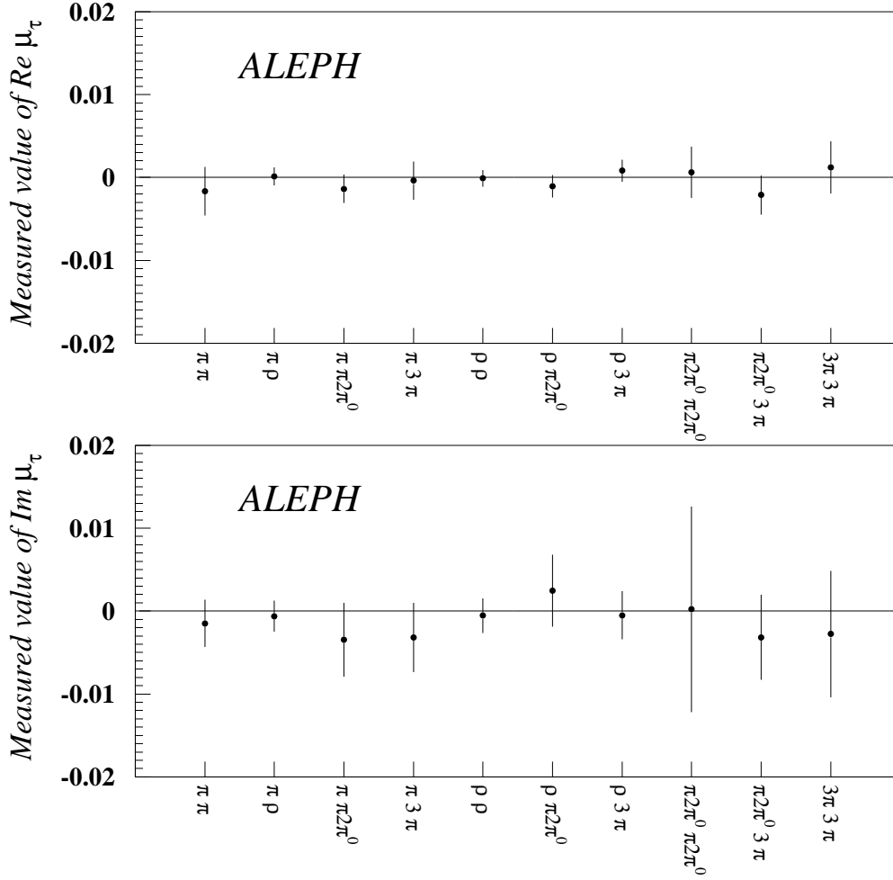
Figure 4: Results on \mu_\tau for the various decay modes, including both the statistical and the systematic uncertainties. The results on \text{Re } \mu_\tau are shown at the top, and on \text{Im } \mu_\tau at the bottom.
