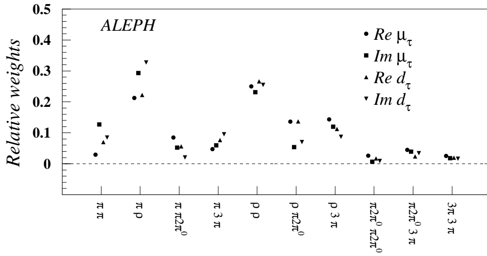
Figure 6: Relative weights of the different decay topologies for the four measured anomalous weak dipole moments, normalised to the total weight.
