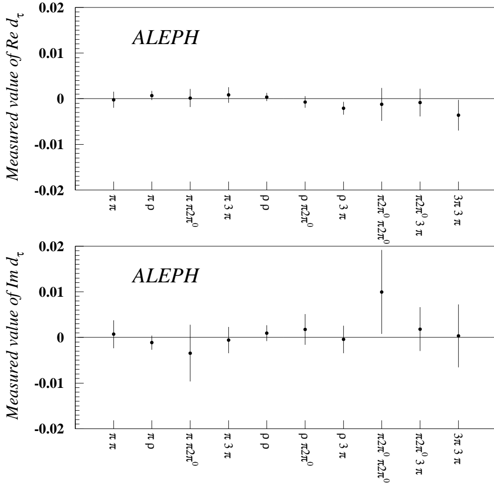
Figure 5: Results on d_\tau for the various decay modes, including both the statistical and the systematic uncertainties. The results on \text{Re } d_\tau are shown at the top, and on \text{Im } d_\tau at the bottom. The anomalous weak electric dipole moment is assumed dimensionless in these figures.
