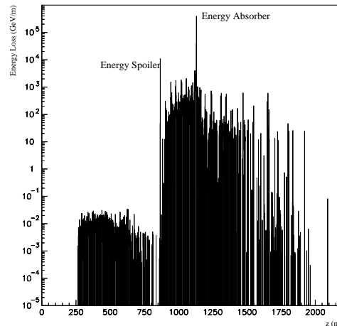
Figure 5: Energy loss in the BDS determined using BDSIM as a function of distance from the linac for a CLIC bunch generated in PLACET with energy 2% lower than nominal. The energy loss before the spoiler is due to synchrotron radiation. 1000 1.5 TeV electrons plus secondaries have been tracked for this plot. Only the first part of the collimation system is shown, since little energy is lost further downstream. Simulation with better statistics needs to be performed to obtain meaningful results for this region.
