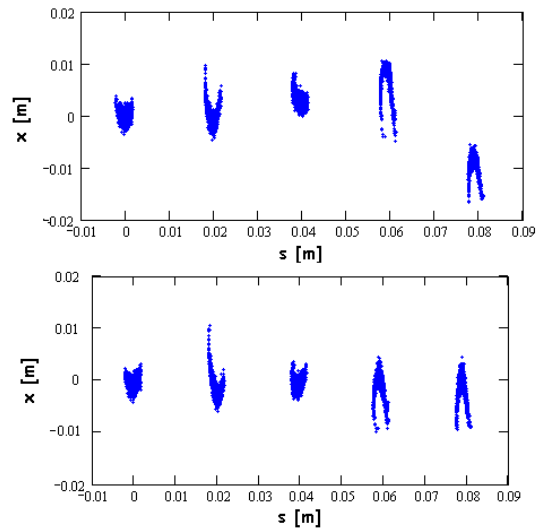
Figure 5: Simulated bunch combination factor of five with phase errors on the RF deflectors. Top: Relative phase error of 5^\circ between the first and the second deflector, losses are close to 40%. Bottom: Phase jitter of -5^\circ in both deflectors, losses are below 5%.
