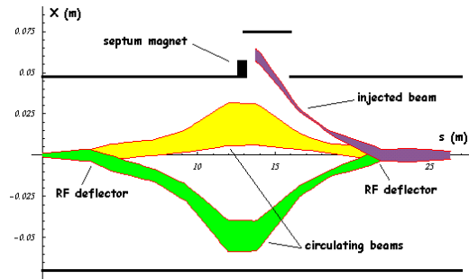
Figure 2: Beam envelopes of the bunches of Figure 1. From top to bottom: injected bunch, circulating bunches with phase \frac{2\pi}{5} and \frac{4\pi}{5} . The lines are the limits of the vacuum chamber and the rectangle stands for the injection septum.
