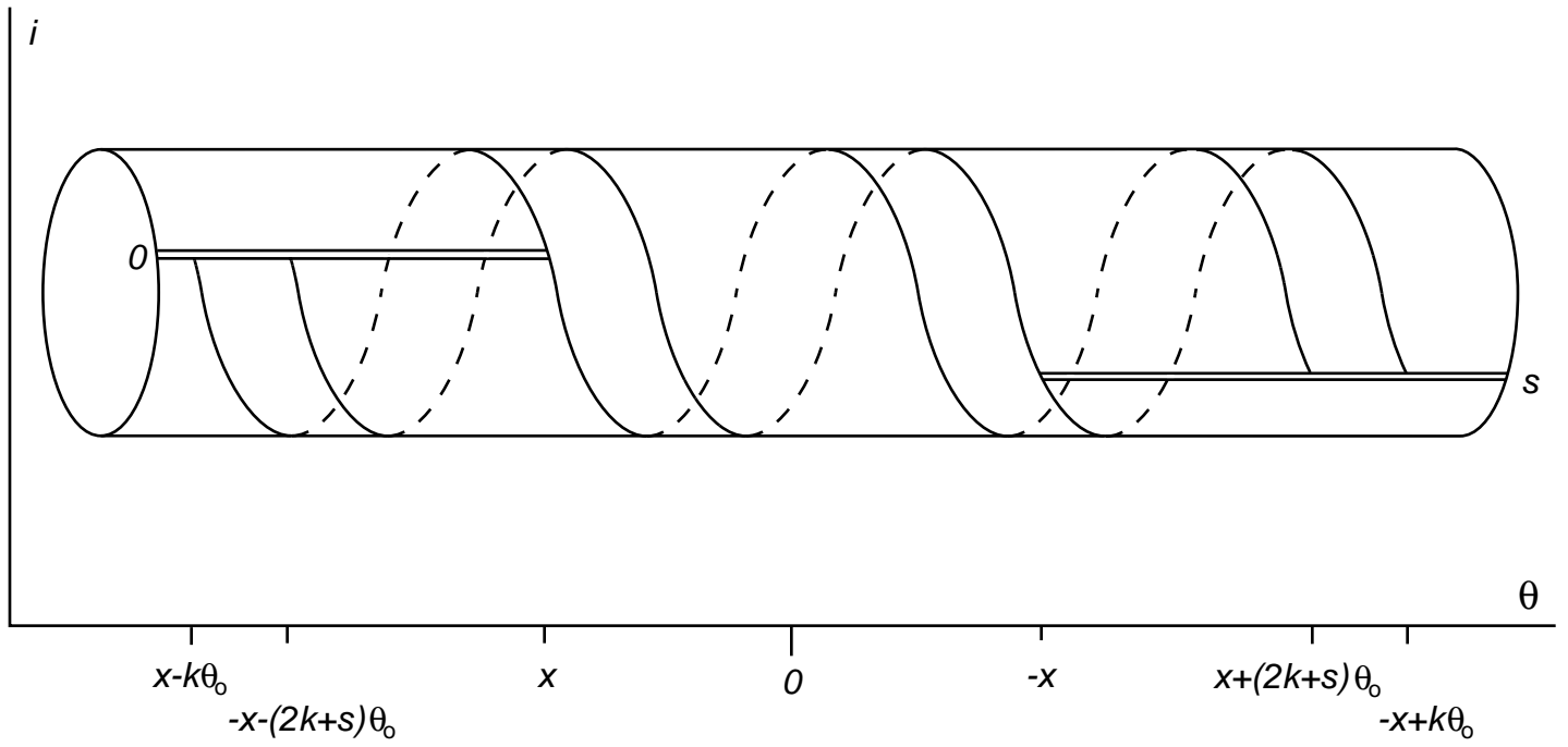
Figure 1 : The arrangement of kinks around the cylinder.
