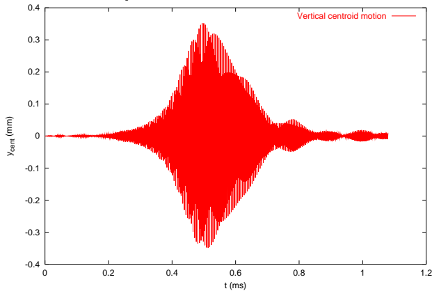
Figure 4: Vertical centroid motion of an SIS bunch (single bunch configuration) when the cooler parameters are n_e = 10^{12} \text{ m}^{-3} and B = 0.67 \text{ mT} .
