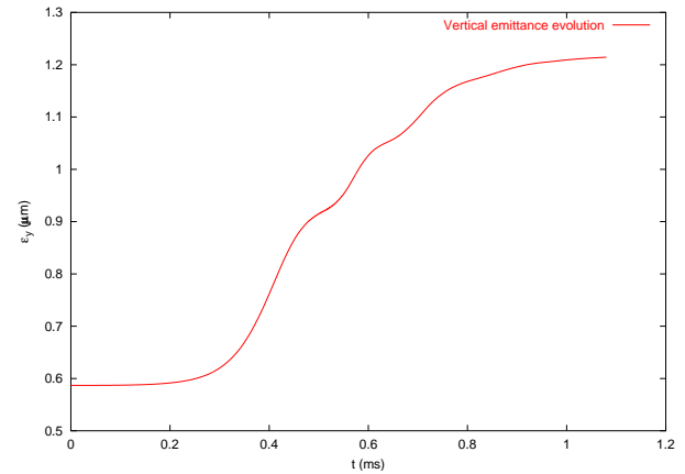
Figure 5: Emittance growth of an SIS bunch (single bunch configuration) when the cooler parameters are n_e = 10^{12} \text{ m}^{-3} and B = 0.67 \text{ mT} .
