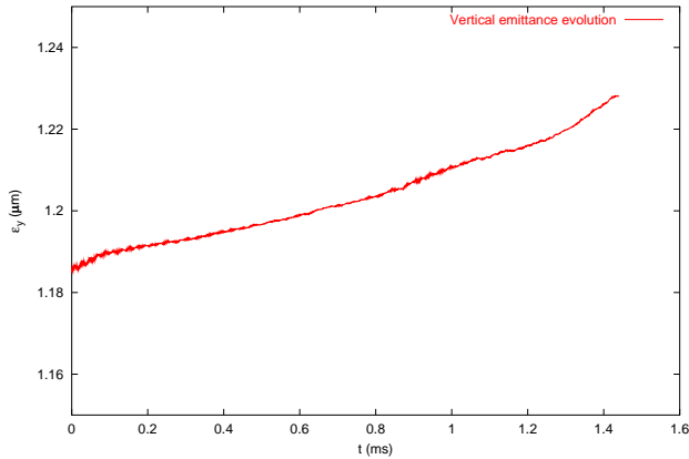
Figure 3: Emittance growth of an SIS bunch when the cooler parameters are n_e = 6 \times 10^{13} \text{ m}^{-3} and B = 9.5 \text{ mT} .
