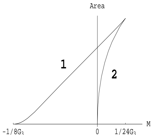
Figure 1: Mass dependence of the 4D area of black holes on an AdS_3 brane.
