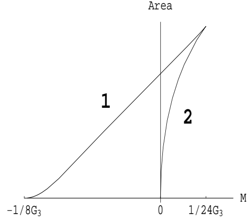
Figure 1: Mass dependence of the 4D area of black holes on an AdS_3 brane.
