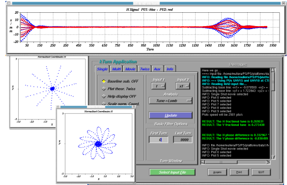
Figure 2: Screen shot of the KiTA toolkit with main form, representations of measured horizontal beam centre-of-charge position at two pick-ups as a function of turn and reconstructed normalised phase space for different turn ranges (0–250 and 1450–1850, respectively).
