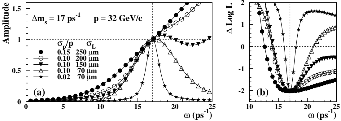
Figure 3: (a) Expected amplitude shape for a true frequency \Delta m_s = 17 \text{ ps}^{-1} , monochromatic B_s mesons of p = 32 \text{ GeV}/c and different values of momentum and decay length resolutions (taken to be Gaussian)
